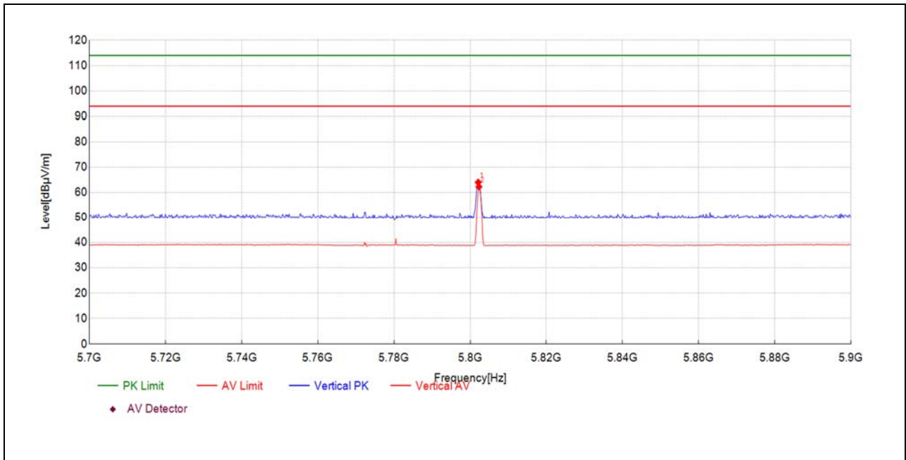
(5801MHz, Antenna Vertical)
