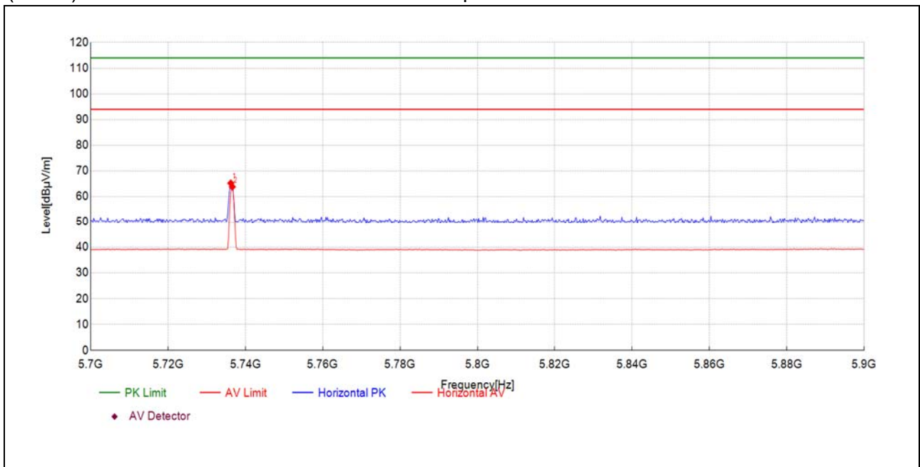
(5735MHz, Antenna Horizontal)
