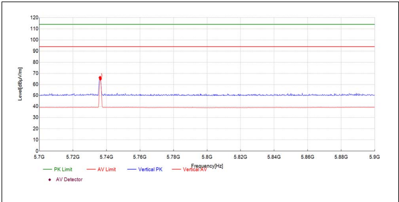
(5735MHz, Antenna Vertical)
