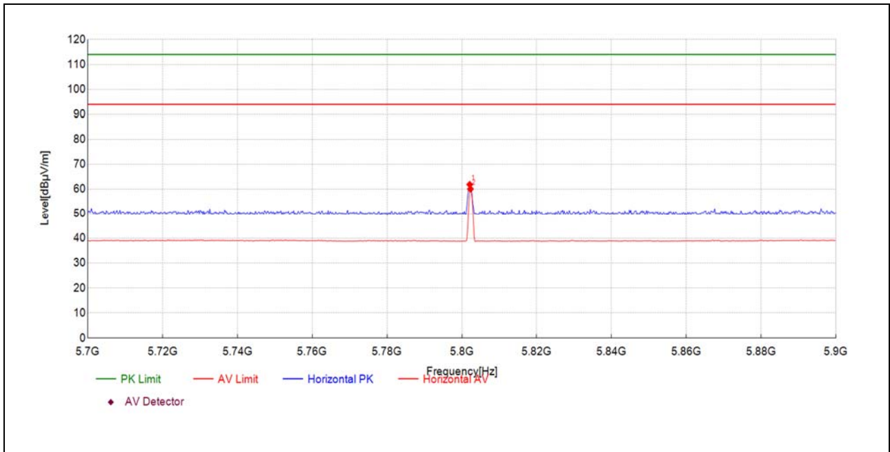
(5801MHz, Antenna Horizontal)
