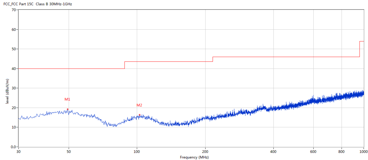
Test Figure: TX mode
