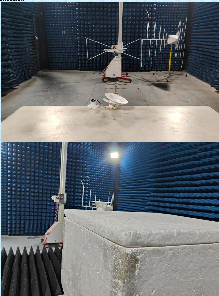
Radiated Emission
