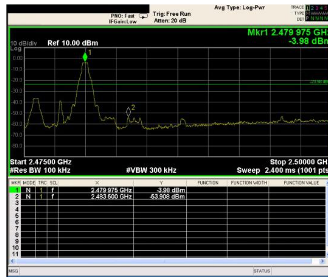
GFSK: Band Edge-High Channel (Hopping Mode)
