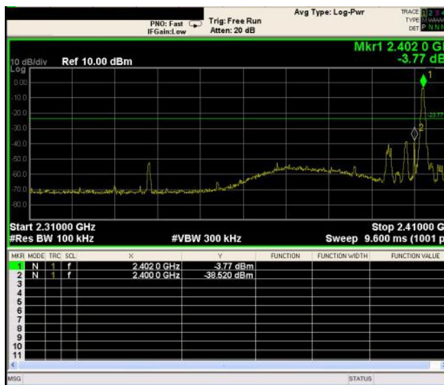
GFSK: Band Edge-Low Channel (Hopping Mode)
