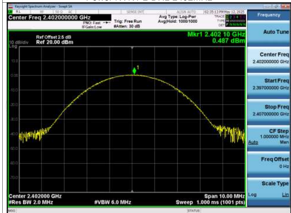
Power NVNT 2-DH1 2402MHz
