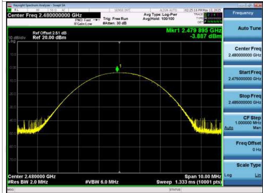
Power NVNT 1-DH1 2480MHz
