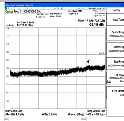
Band66_15MHz_16QAM_132047_1RB#0_3000 ~20000_3000~20000
