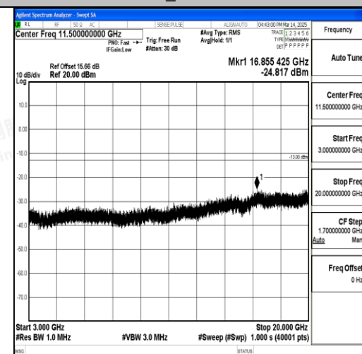
Band66_15MHz_16QAM_132597_1RB#0_3000 ~20000_3000~20000
