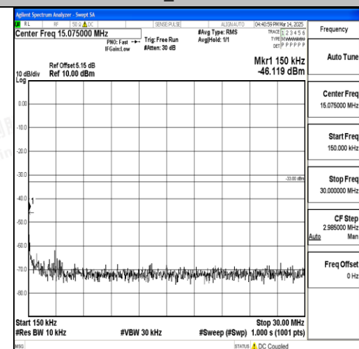
Band66_15MHz_QPSK_132322_1RB#0_0.15~3 0_0.15~30
