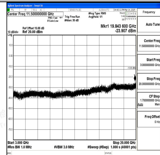
Band66_15MHz_QPSK_132047_1RB#0_3000~ 20000_3000~20000
