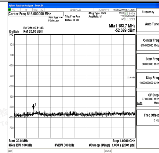
Band66_20MHz_QPSK_132572_1RB#0_30~10 00_30~1000
