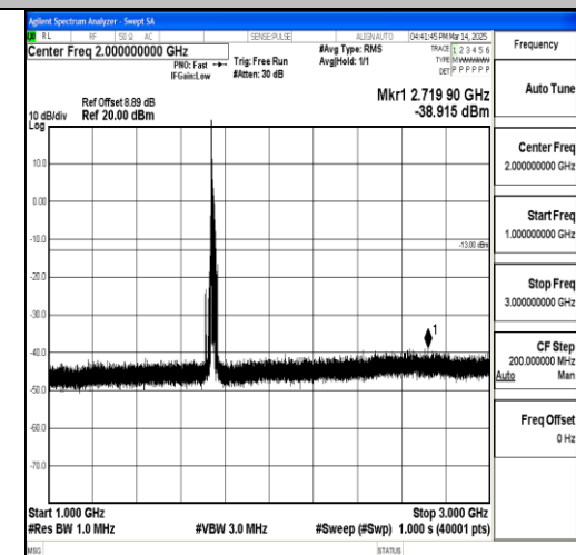
Band66_15MHz_16QAM_132322_1RB#0_1000 ~3000_1000~3000
