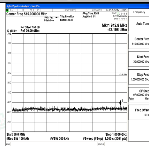
Band66_15MHz_16QAM_132597_1RB#0_30~1 000_30~1000
