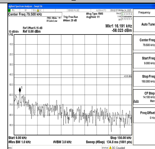
Band66_20MHz_QPSK_132072_1RB#0_0.009~ 0.15_0.009~0.15
