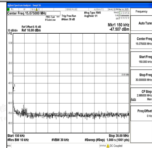
Band66_15MHz_16QAM_132322_1RB#0_0.15~ 30_0.15~30
