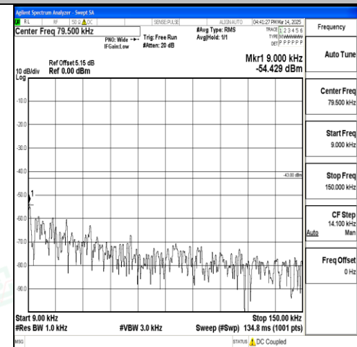
Band66_15MHz_16QAM_132322_1RB#0_0.009 ~0.15_0.009~0.15
