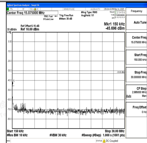
Band66_20MHz_16QAM_132322_1RB#0_0.15~30_0.15~30
