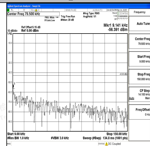
Band66_15MHz_QPSK_132322_1RB#0_0.009~ 0.15_0.009~0.15
