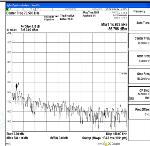
Band66_20MHz_16QAM_132322_1RB#0_0.009~0.15_0.009~0.15
