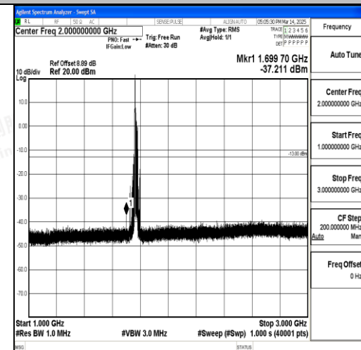
Band66_20MHz_QPSK_132572_1RB#0_1000~ 3000_1000~3000
