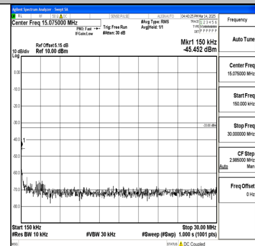
Band66_15MHz_16QAM_132047_1RB#0_0.15~ 30_0.15~30
