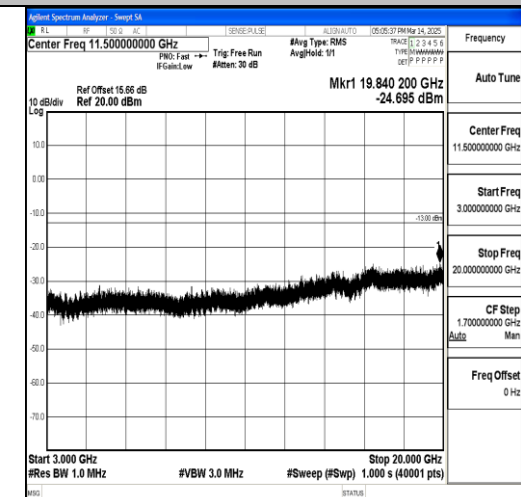
Band66_20MHz_QPSK_132572_1RB#0_3000~ 20000_3000~20000
