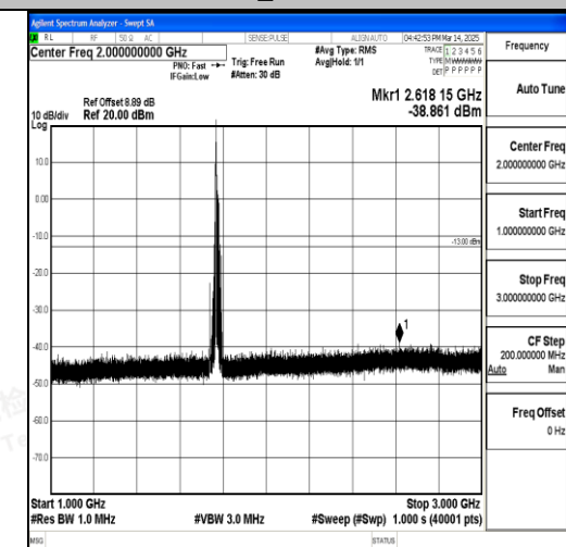
Band66_15MHz_16QAM_132597_1RB#0_1000 ~3000_1000~3000
