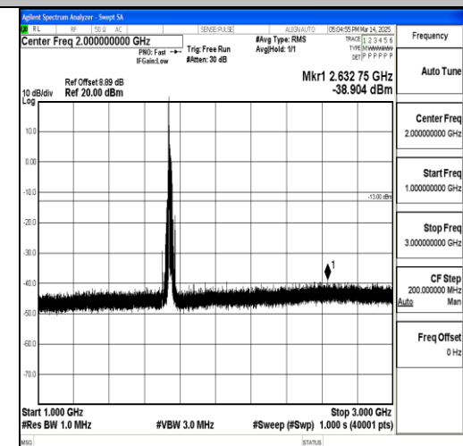
Band66_20MHz_16QAM_132322_1RB#0_1000~3000_1000~3000
