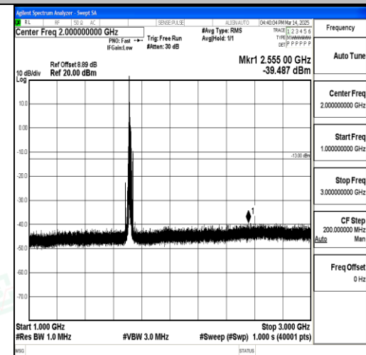
Band66_15MHz_QPSK_132047_1RB#0_1000~ 3000_1000~3000
