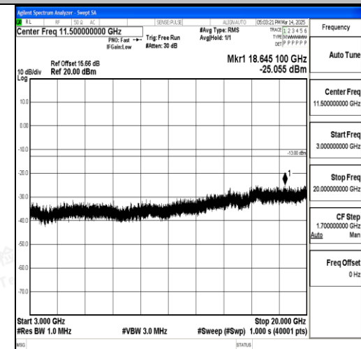
Band66_20MHz_QPSK_132072_1RB#0_3000~ 20000_3000~20000
