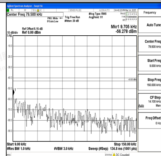
Band66_15MHz_16QAM_132047_1RB#0_0.009 ~0.15_0.009~0.15
