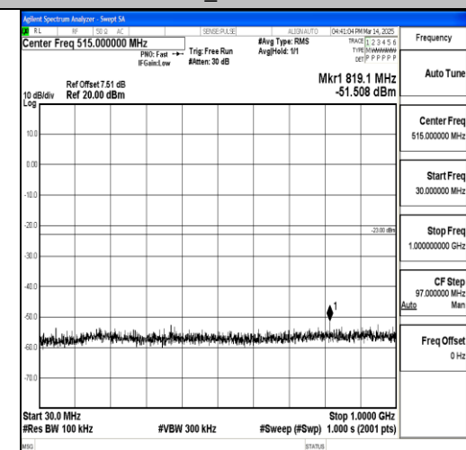
Band66_15MHz_QPSK_132322_1RB#0_30~10 00_30~1000
