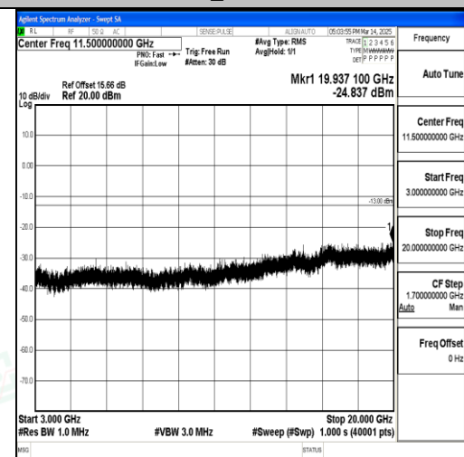
Band66_20MHz_16QAM_132072_1RB#0_3000 ~20000_3000~20000
