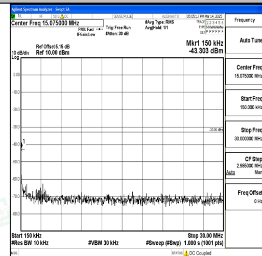
Band66_20MHz_QPSK_132572_1RB#0_0.15~3 0_0.15~30
