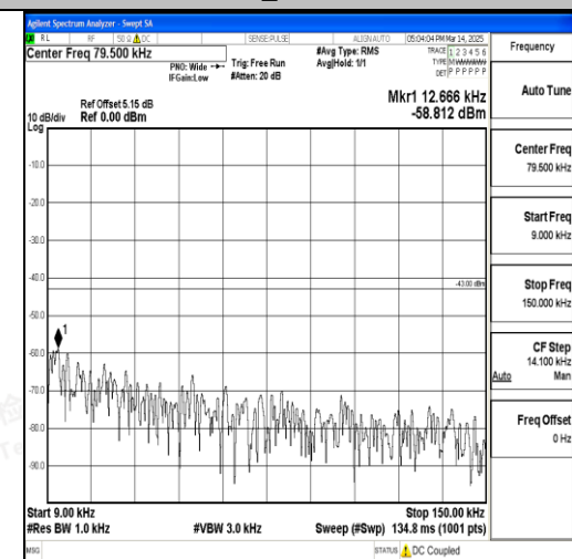
Band66_20MHz_QPSK_132322_1RB#0_0.009~ 0.15_0.009~0.15
