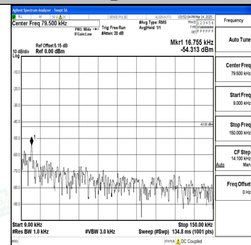
Band66_5MHz_QPSK_131997_1RB#0_0.009~0.15_0.009~0.15
