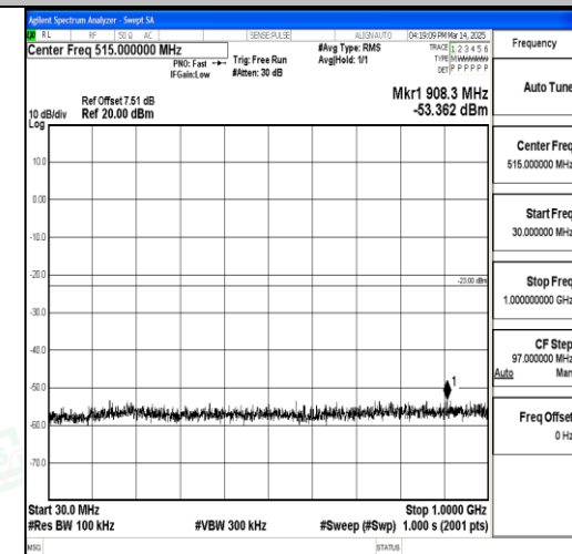
Band66_10MHz_16QAM_132622_1RB#0_30~1 000_30~1000
