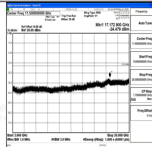
Band66_10MHz_QPSK_132022_1RB#0_3000~ 20000_3000~20000
