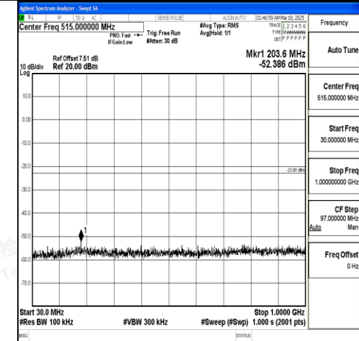
Band66_3MHz_QPSK_132657_1RB#0_30~100 0_30~1000
