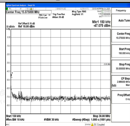
Band66_5MHz_16QAM_132322_1RB#0_0.15~3 0_0.15~30
