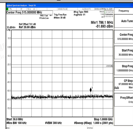
Band66_5MHz_QPSK_131997_1RB#0_30~100_0_30~1000
