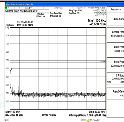
Band66_10MHz_QPSK_132622_1RB#0_0.15~3 0_0.15~30
