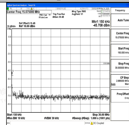
Band66_5MHz_QPSK_131997_1RB#0_0.15~30_0.15~30
