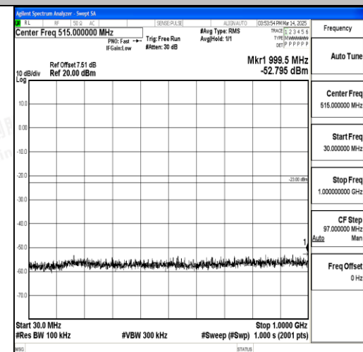
Band66_5MHz_16QAM_132322_1RB#0_30~10 00_30~1000
