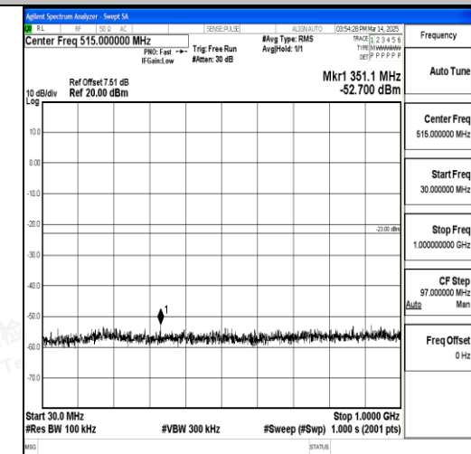
Band66_5MHz_QPSK_132647_1RB#0_30~100 0_30~1000
