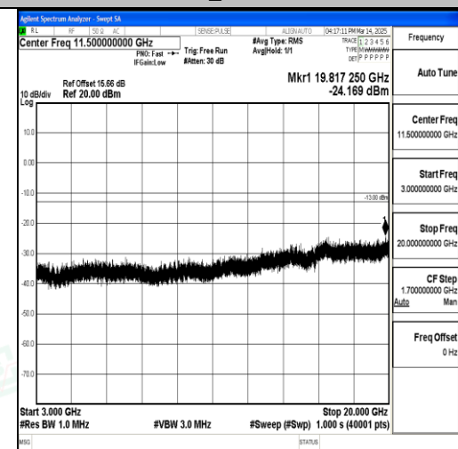
Band66_10MHz_16QAM_132022_1RB#0_3000 ~20000_3000~20000
