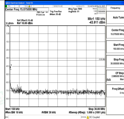
Band66_3MHz_QPSK_132657_1RB#0_0.15~30 _0.15~30
