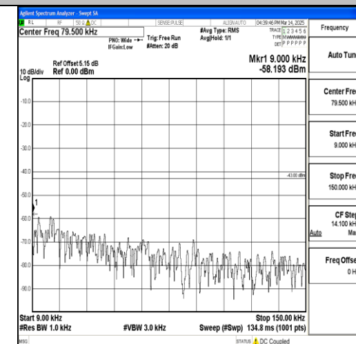
Band66_15MHz_QPSK_132047_1RB#0_0.009~ 0.15_0.009~0.15
