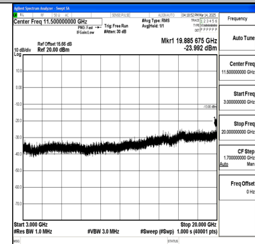
Band66_10MHz_QPSK_132622_1RB#0_3000~ 20000_3000~20000
