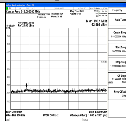
Band66_10MHz_QPSK_132322_1RB#0_30~10 00_30~1000
