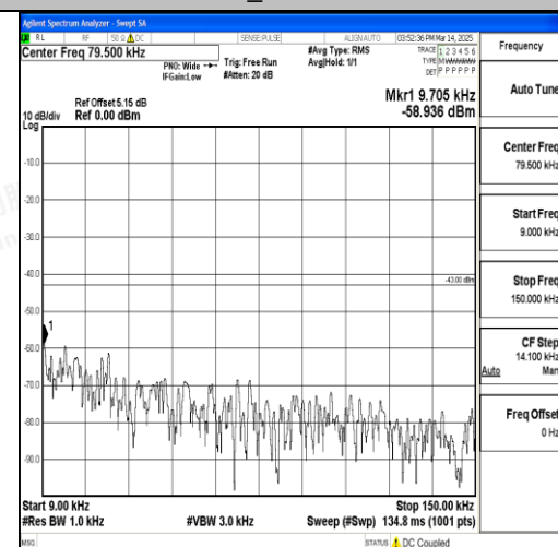
Band66_5MHz_16QAM_131997_1RB#0_0.009~ 0.15_0.009~0.15
