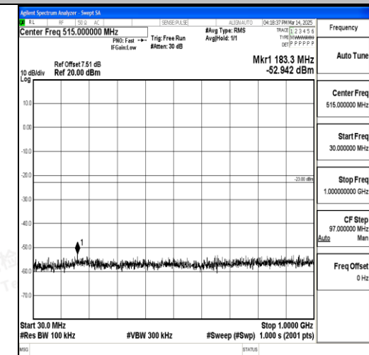
Band66_10MHz_QPSK_132622_1RB#0_30~10 00_30~1000
