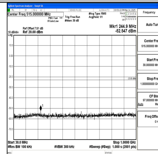
Band66_5MHz_QPSK_132322_1RB#0_30~1000 0_30~1000
