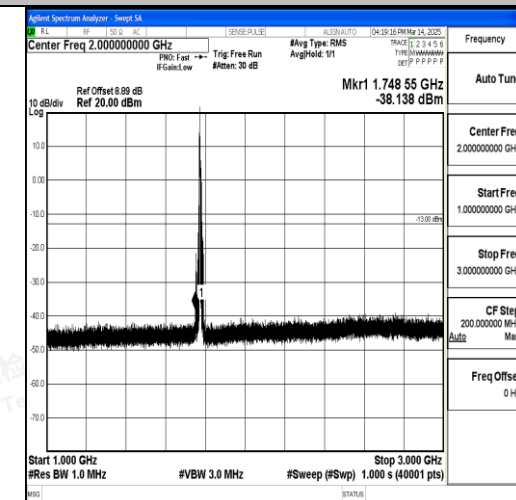
Band66_10MHz_16QAM_132622_1RB#0_1000 ~3000_1000~3000
