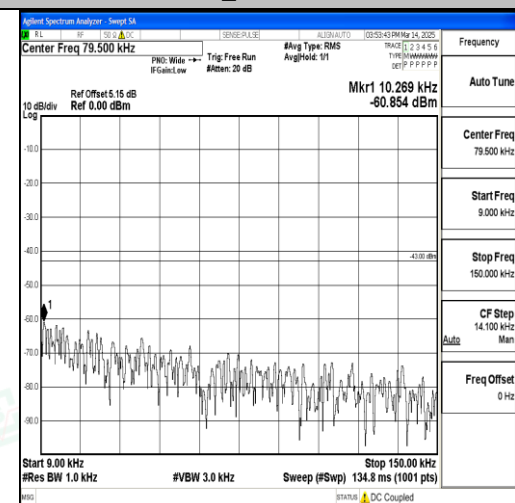
Band66_5MHz_16QAM_132322_1RB#0_0.009~ 0.15_0.009~0.15
