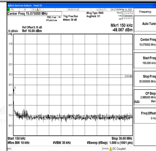
Band66_10MHz_16QAM_132322_1RB#0_0.15~ 30_0.15~30
