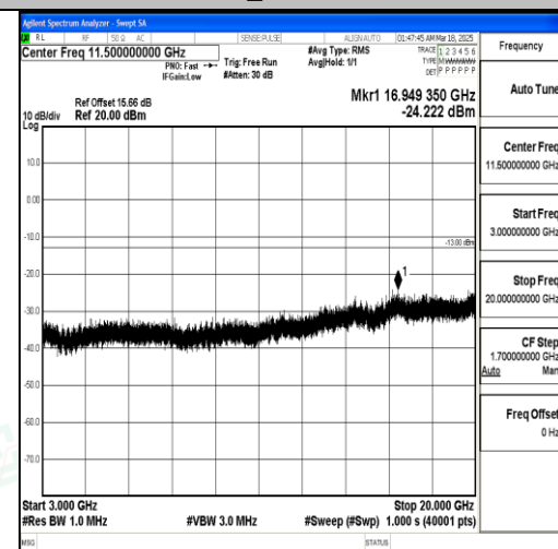
Band66_3MHz_16QAM_132657_1RB#0_3000~ 20000_3000~20000
