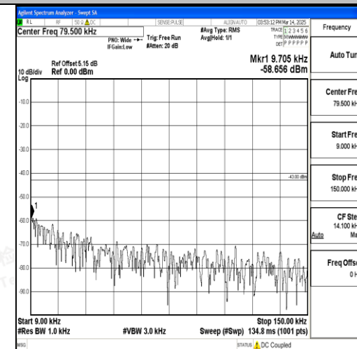
Band66_5MHz_QPSK_132322_1RB#0_0.009~0 .15_0.009~0.15
