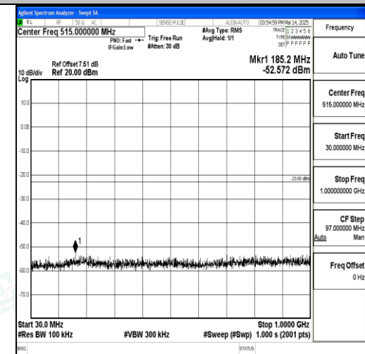
Band66_5MHz_16QAM_132647_1RB#0_30~10 00_30~1000
