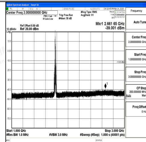
Band66_10MHz_QPSK_132622_1RB#0_1000~ 3000_1000~3000
