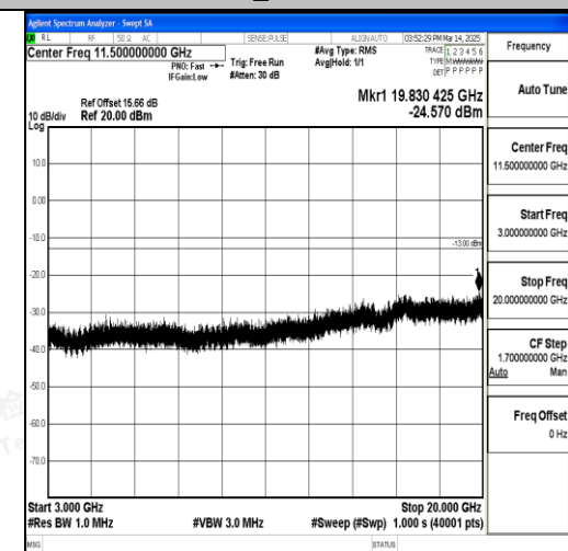
Band66_5MHz_QPSK_131997_1RB#0_3000~2 0000_3000~20000
