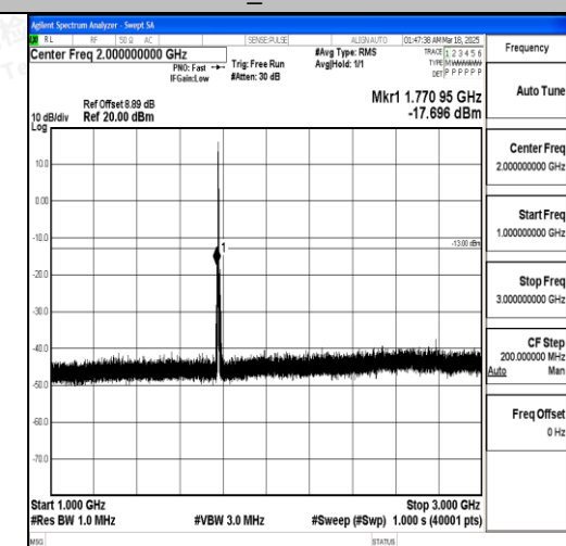
Band66_5MHz_QPSK_131997_1RB#0_1000~3000_000_1000~3000
