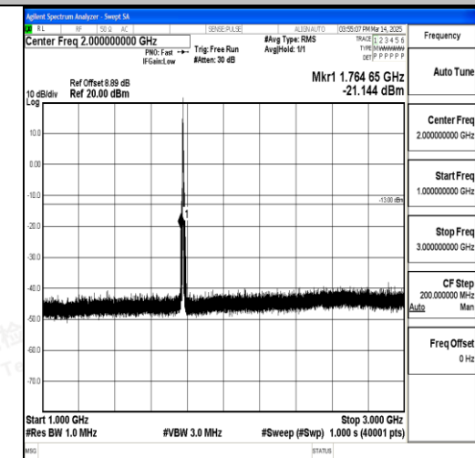
Band66_5MHz_16QAM_132647_1RB#0_1000~ 3000_1000~3000
