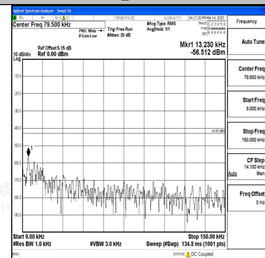
Band66_10MHz_QPSK_132322_1RB#0_0.009~ 0.15_0.009~0.15
