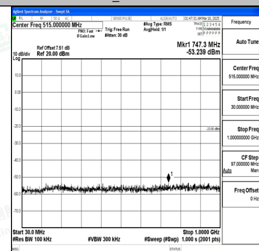
Band66_5MHz_QPSK_131997_1RB#0_30~100_0_30~1000
