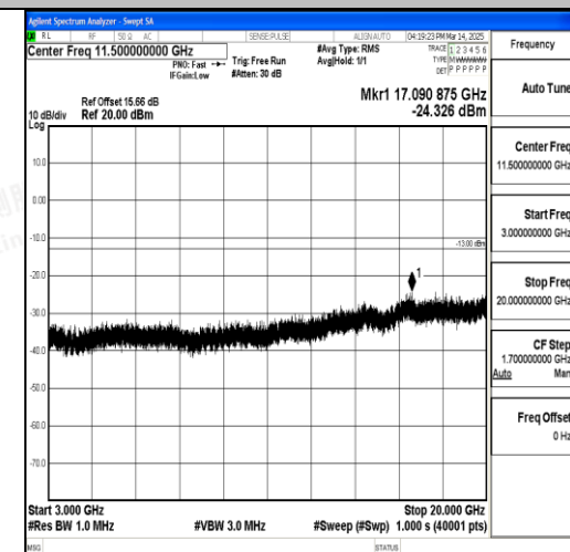
Band66_10MHz_16QAM_132622_1RB#0_3000 ~20000_3000~20000
