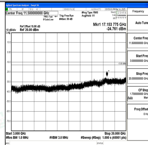
Band66_5MHz_16QAM_131997_1RB#0_3000~ 20000_3000~20000
