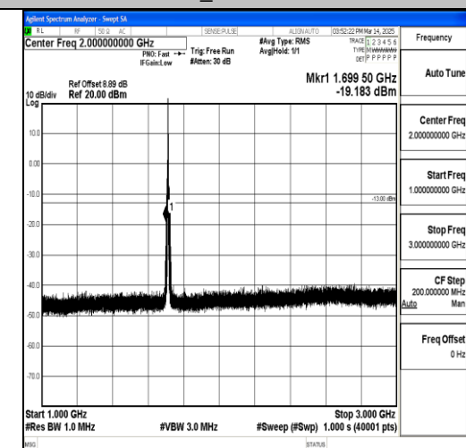
Band66_5MHz_QPSK_131997_1RB#0_1000~3000_000_1000~3000
