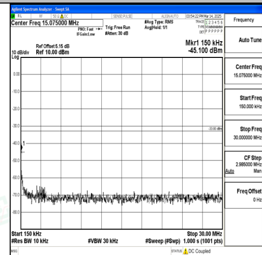
Band66_5MHz_QPSK_132647_1RB#0_0.15~30 _0.15~30
