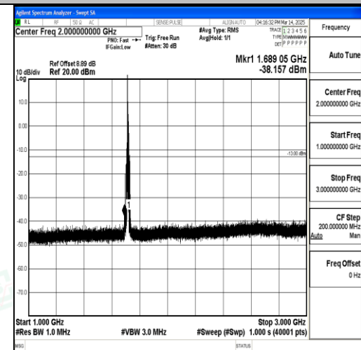
Band66_10MHz_QPSK_132022_1RB#0_1000~ 3000_1000~3000
