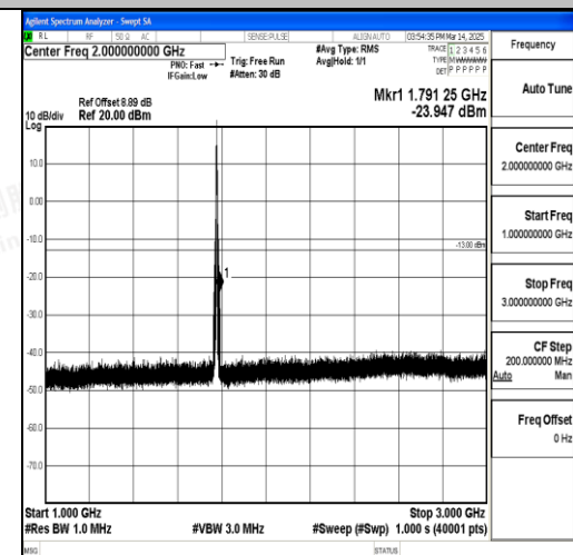
Band66_5MHz_QPSK_132647_1RB#0_1000~3 000_1000~3000
