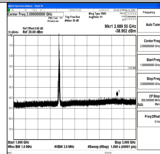
Band66_10MHz_16QAM_132322_1RB#0_1000 ~3000_1000~3000
