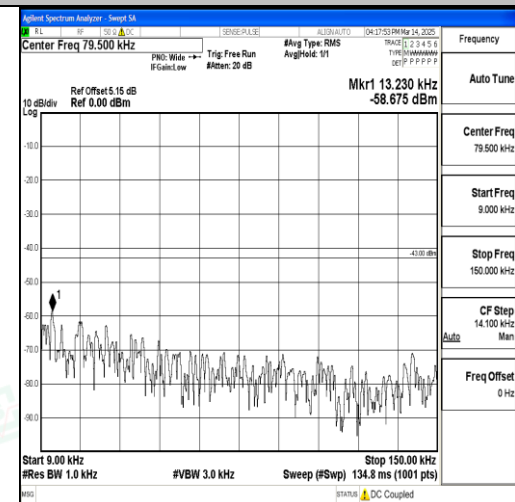
Band66_10MHz_16QAM_132322_1RB#0_0.009 ~0.15_0.009~0.15
