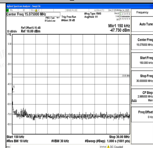
Band66_10MHz_QPSK_132322_1RB#0_0.15~3 0_0.15~30
