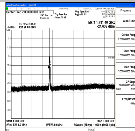
Band66_5MHz_16QAM_132322_1RB#0_1000~ 3000_1000~3000
