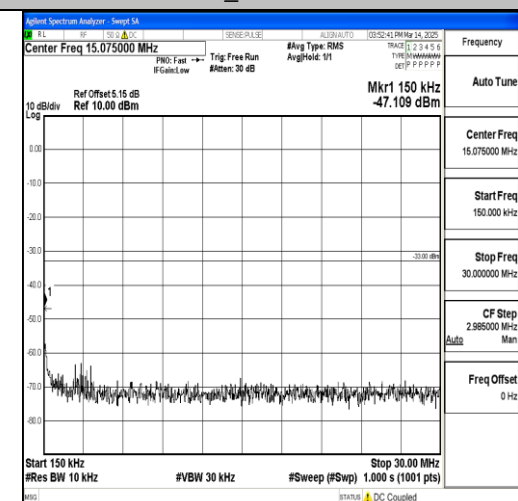
Band66_5MHz_16QAM_131997_1RB#0_0.15~3 0_0.15~30
