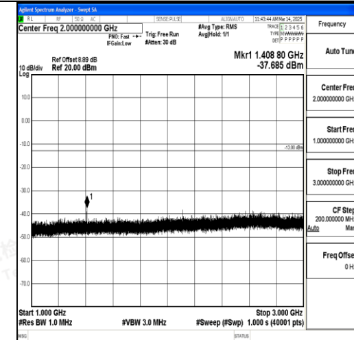
Band17_5MHz_QPSK_23755_1RB#0_1000~300 0_1000~3000
