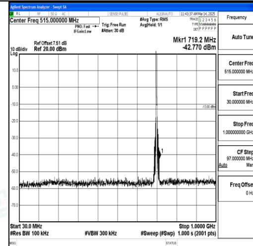
Band17_5MHz_QPSK_23755_1RB#0_30~1000 _30~1000
