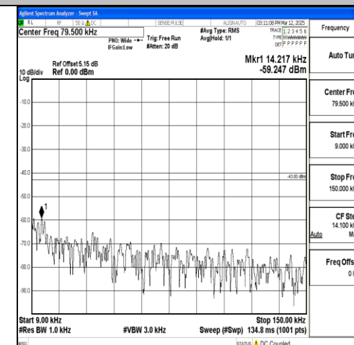
Band4_20MHz_16QAM_20050_1RB#0_0.009~0. 15_0.009~0.15
