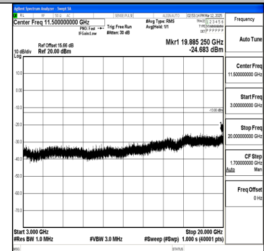
Band4_15MHz_16QAM_20325_1RB#0_3000~20 000_3000~20000
