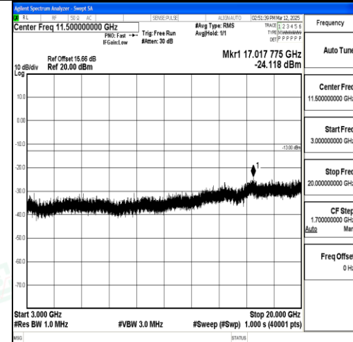
Band4_15MHz_QPSK_20175_1RB#0_3000~20 000_3000~20000
