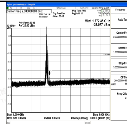
Band4_20MHz_QPSK_20050_1RB#0_1000~300 0_1000~3000
