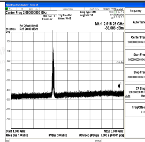
Band4_15MHz_16QAM_20325_1RB#0_1000~3 000_1000~3000
