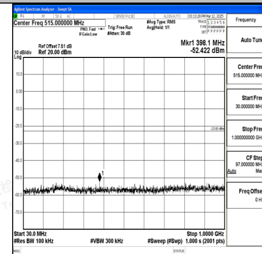
Band4_20MHz_16QAM_20300_1RB#0_30~1000_30~1000
