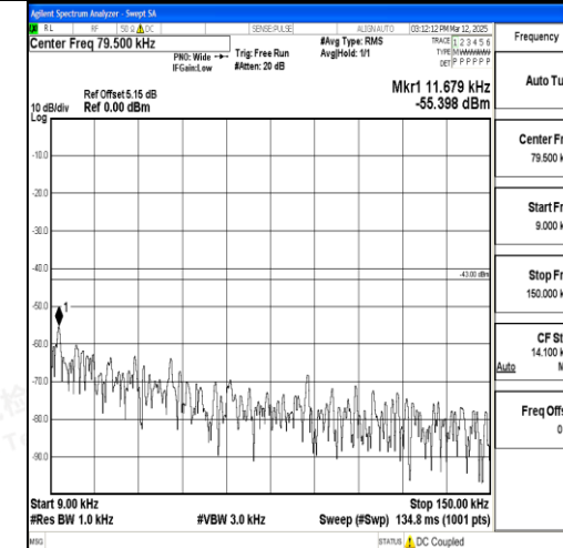
Band4_20MHz_16QAM_20175_1RB#0_0.009~0.15_15_0.009~0.15
