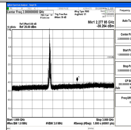
Band4_20MHz_QPSK_20300_1RB#0_1000~3000_0_1000~3000
