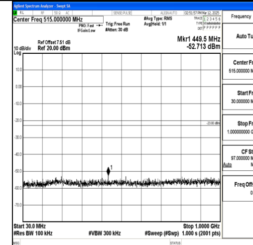
Band4_15MHz_16QAM_20175_1RB#0_30~1000 _30~1000
