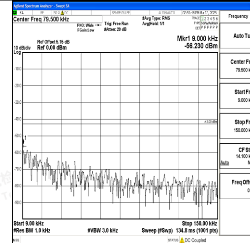
Band4_15MHz_16QAM_20175_1RB#0_0.009~0. 15_0.009~0.15
