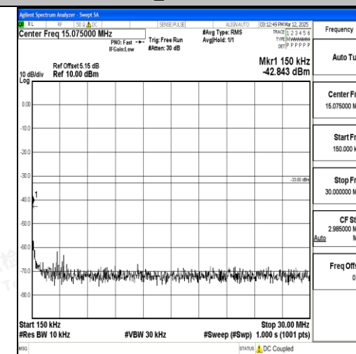
Band4_20MHz_QPSK_20300_1RB#0_0.15~30_0.15~30
