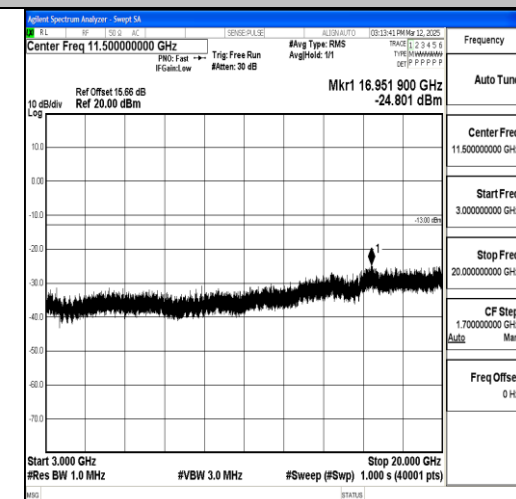
Band4_20MHz_16QAM_20300_1RB#0_3000~20000_000_3000~20000
