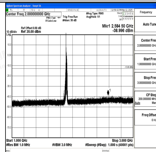
Band2_20MHz_16QAM_19100_1RB#0_1000~3000_000_1000~3000
