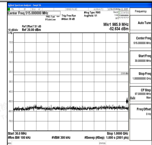
Band2_20MHz_16QAM_19100_1RB#0_30~1000_30~1000
