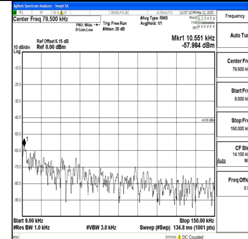
Band2_20MHz_16QAM_18700_1RB#0_0.009~0. 15_0.009~0.15
