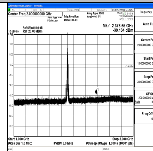
Band2_15MHz_QPSK_19125_1RB#0_1000~3000_0_1000~3000
