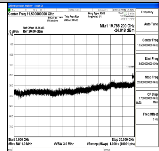
Band2_20MHz_16QAM_19100_1RB#0_3000~20000_000_3000~20000
