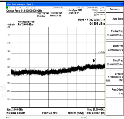
Band2_15MHz_16QAM_18675_1RB#0_3000~20 000_3000~20000
