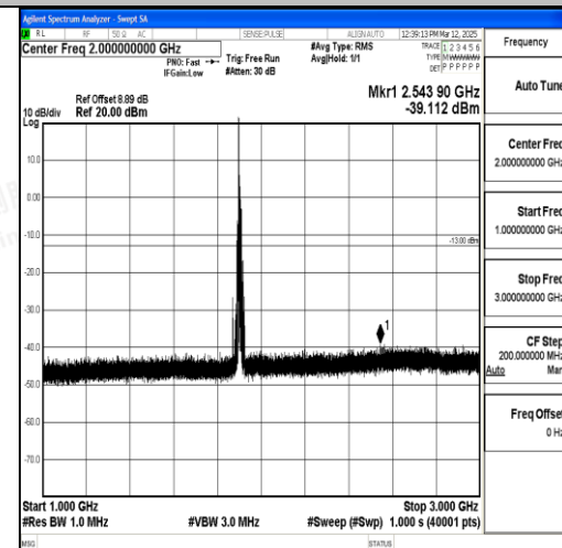
Band2_15MHz_16QAM_19125_1RB#0_1000~3 000_1000~3000
