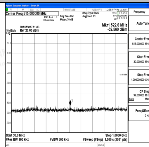
Band2_15MHz_QPSK_19125_1RB#0_30~1000_30~1000
