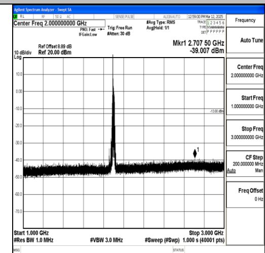
Band2_20MHz_QPSK_19100_1RB#0_1000~3000_0_1000~3000
