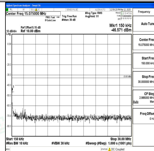
Band2_20MHz_16QAM_19100_1RB#0_0.15~30_0.15~30
