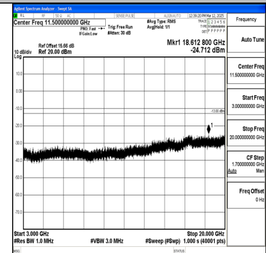
Band2_15MHz_16QAM_19125_1RB#0_3000~20 000_3000~20000
