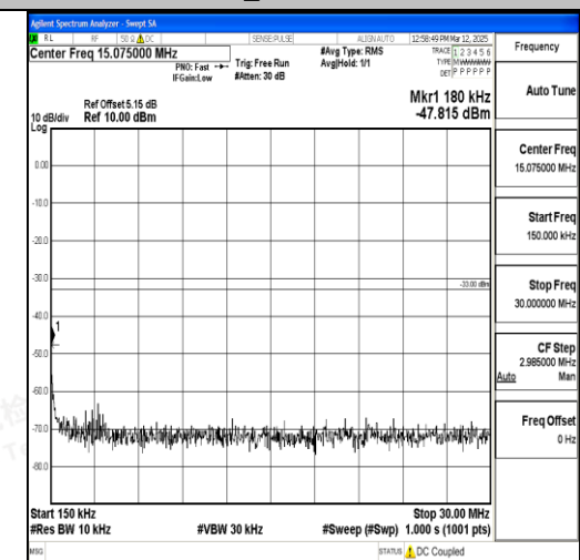
Band2_20MHz_QPSK_19100_1RB#0_0.15~30_0.15~30
