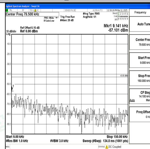
Band2_15MHz_QPSK_19125_1RB#0_0.009~0.15_0.009~0.15
