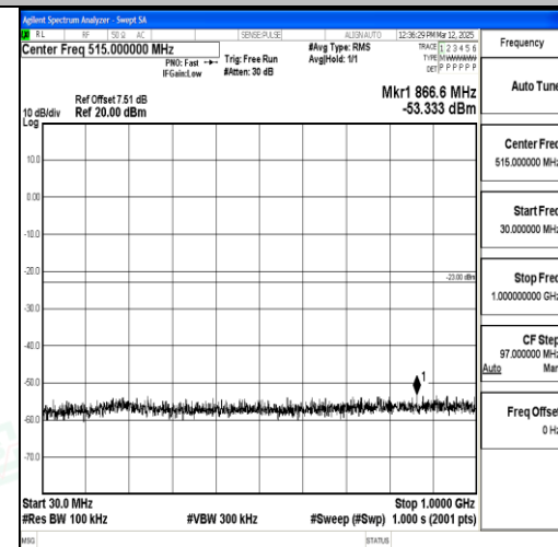
Band2_15MHz_QPSK_18675_1RB#0_30~1000 _30~1000
