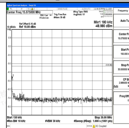
Band2_15MHz_QPSK_19125_1RB#0_0.15~30_0.15~30
