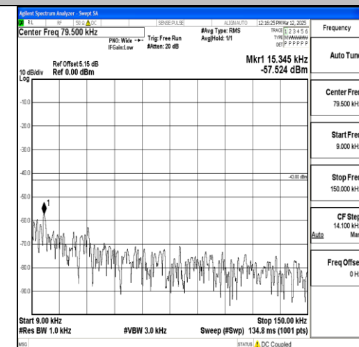
Band2_10MHz_16QAM_18650_1RB#0_0.009~0. 15_0.009~0.15
