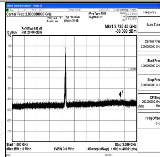
Band2_10MHz_16QAM_18650_1RB#0_1000~3 000_1000~3000
