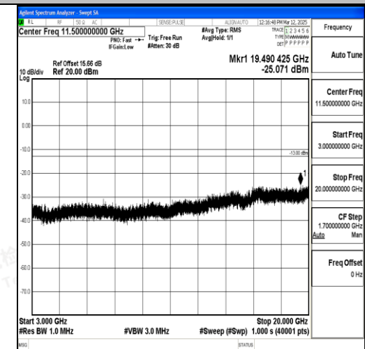
Band2_10MHz_16QAM_18650_1RB#0_3000~20 000_3000~20000
