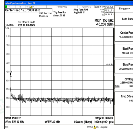
Band2_5MHz_16QAM_19175_1RB#0_0.15~30 _0.15~30
