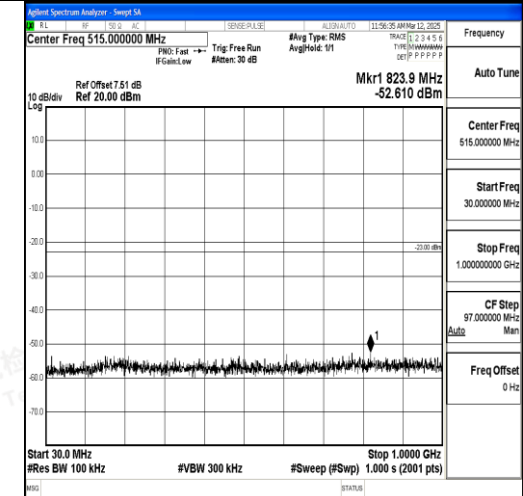
Band2_5MHz_16QAM_19175_1RB#0_30~1000 30~1000
