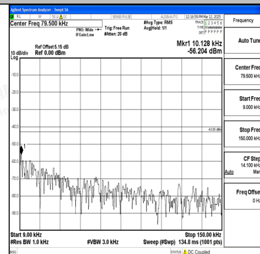
Band2_10MHz_QPSK_18900_1RB#0_0.009~0. 15_0.009~0.15
