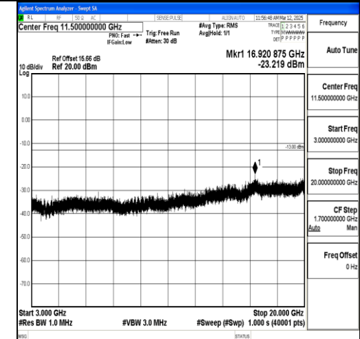
Band2_5MHz_16QAM_19175_1RB#0_3000~200 00_3000~20000
