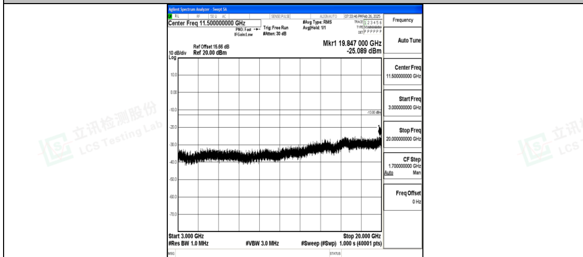
Band4_20MHz_16QAM_20300_1RB#0_3000~20000_3000~20000
