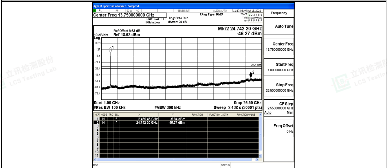
11N20SISO_Ant_2412_0~Reference
