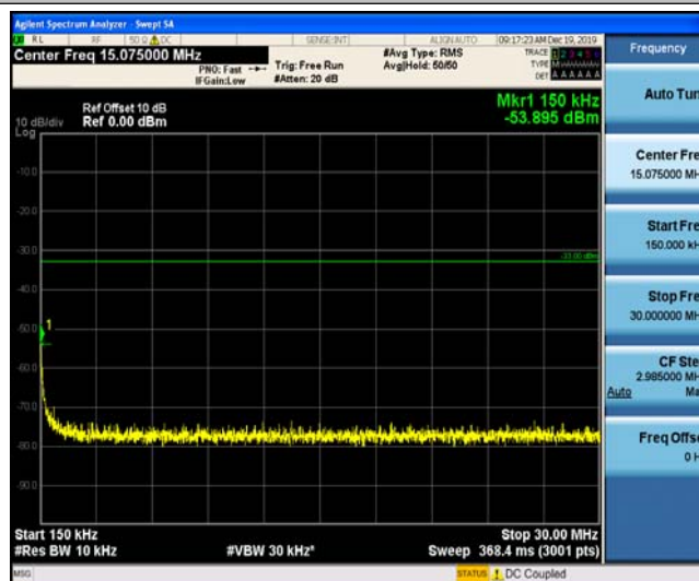
Band25_3MHz_QPSK_24055_1RB#0
