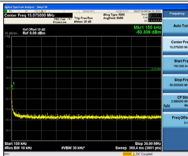
Band25_1.4MHz_QPSK_26365_1RB#0
