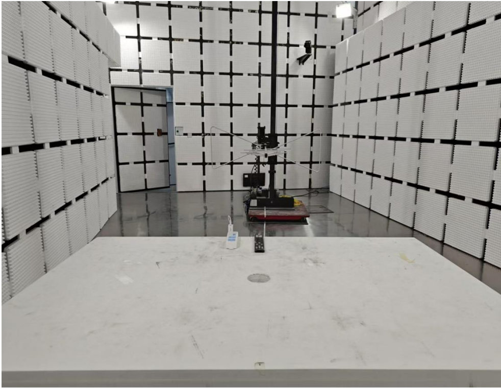
Radiated Emissions Test Photo
