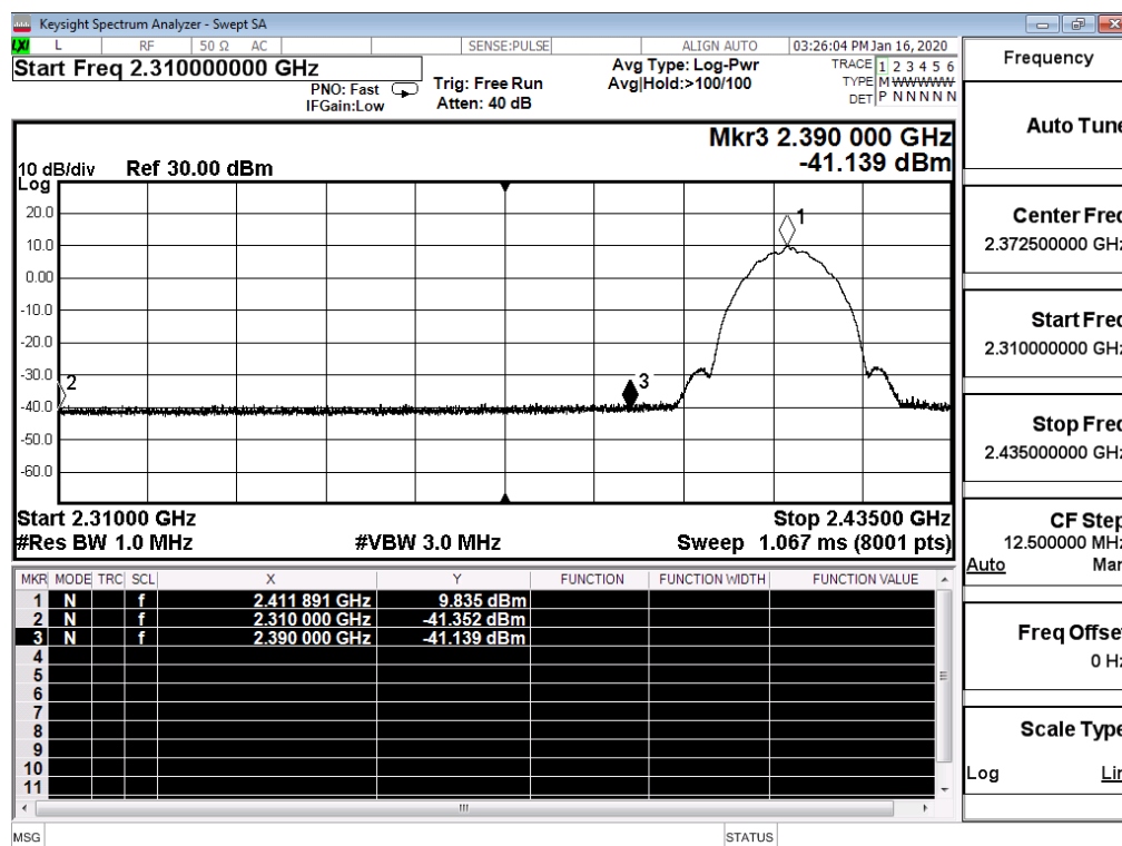
Restrict-band band-edge measurements_11B_2412_Ant1_PEAK
