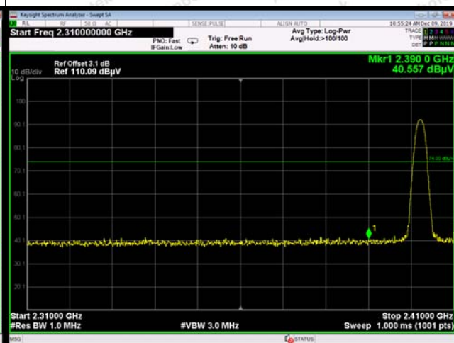
Peak Value(Horizontal)
