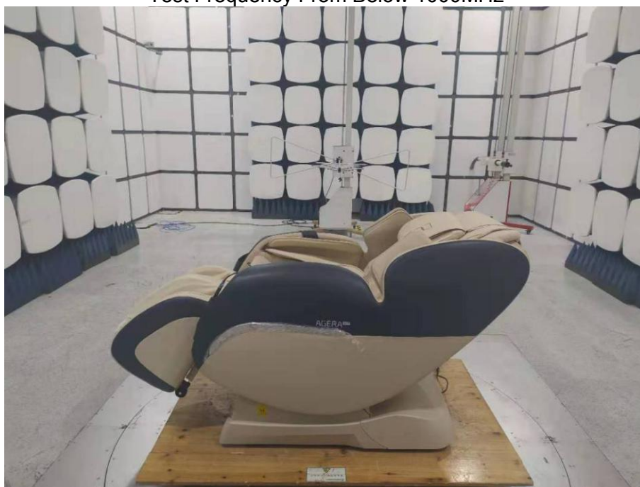
Radiated Spurious Emissions Test Frequency From Below 1000MHz
