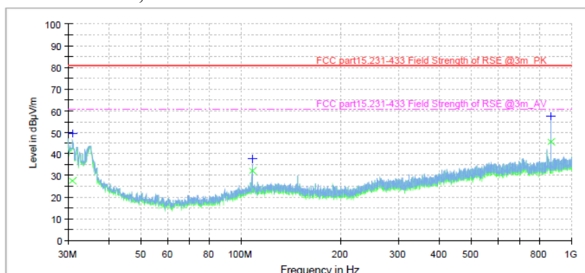
Figure 4: Spectral Diagrams, Radiated Spurious Emission
