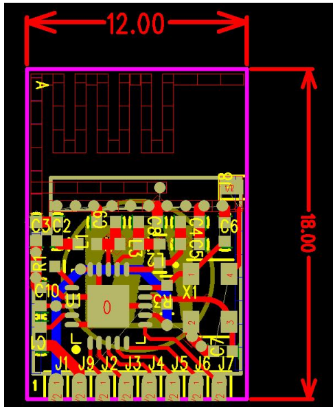
PCB Antenna
