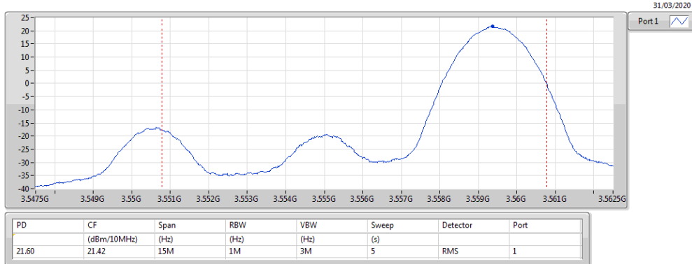
Band 48_LTE_10MHz_Nss1,16QAM_1TX 3555MHz_16QAM_RB 1,#RB H
