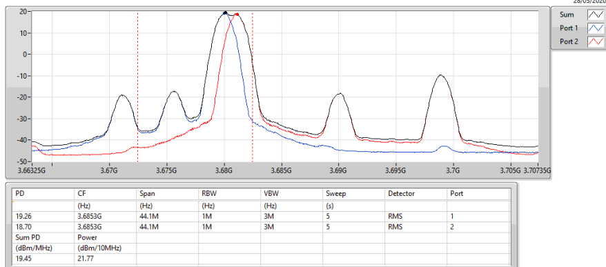
Band 48_LTE_10MHz+20MHz_Nss1,16QAM_2TX P#3675.6MHz,#3690MHz_16QAM_P_1@H+S_1@L
