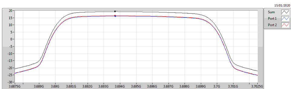
Band 48_LTE_10MHz_Nss1,QPSK_2TX 3695MHz_QPSK_RB 50,#RB 0
