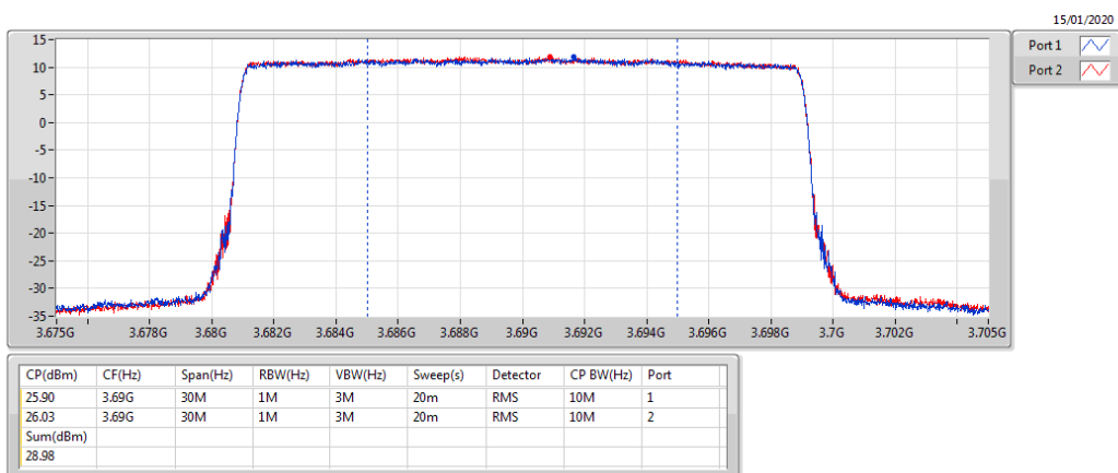
Band 48_LTE_20MHz_Nss1,64QAM_2TX 3690MHz_64QAM_RB 100,#RB 0
