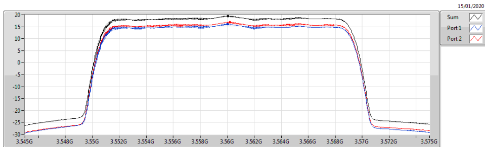
Band 48_LTE_20MHz_Nss1,16QAM_2TX 3560MHz_16QAM_RB 100,#RB 0
