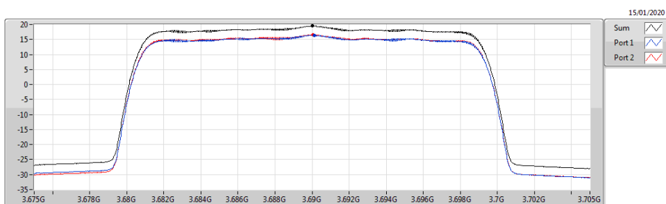
Band 48_LTE_20MHz_Nss1,16QAM_2TX 3690MHz_16QAM_RB 100,#RB 0
