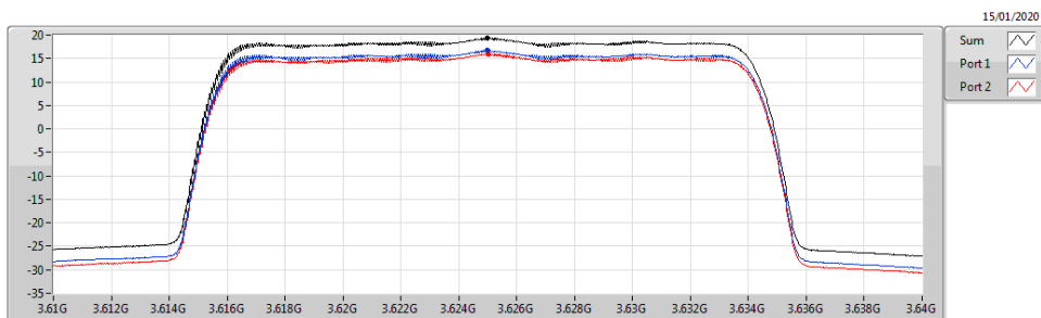
Band 48_LTE_20MHz_Nss1,16QAM_2TX 3625MHz_16QAM_RB 100,#RB 0
