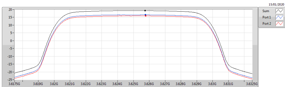
Band 48_LTE_10MHz_Nss1,QPSK_2TX 3625MHz_QPSK_RB 50,#RB 0
