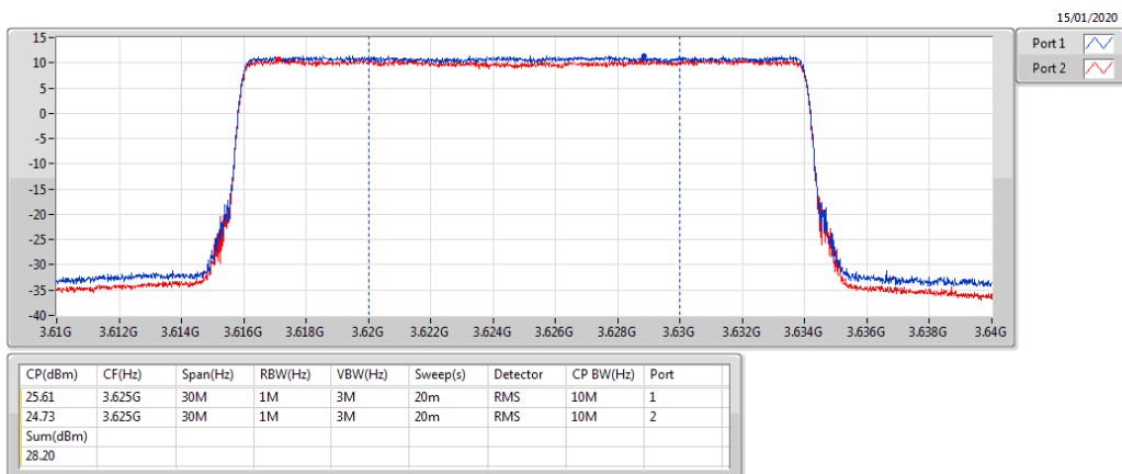
Band 48_LTE_20MHz_Nss1,64QAM_2TX 3625MHz_64QAM_RB 100,#RB 0
