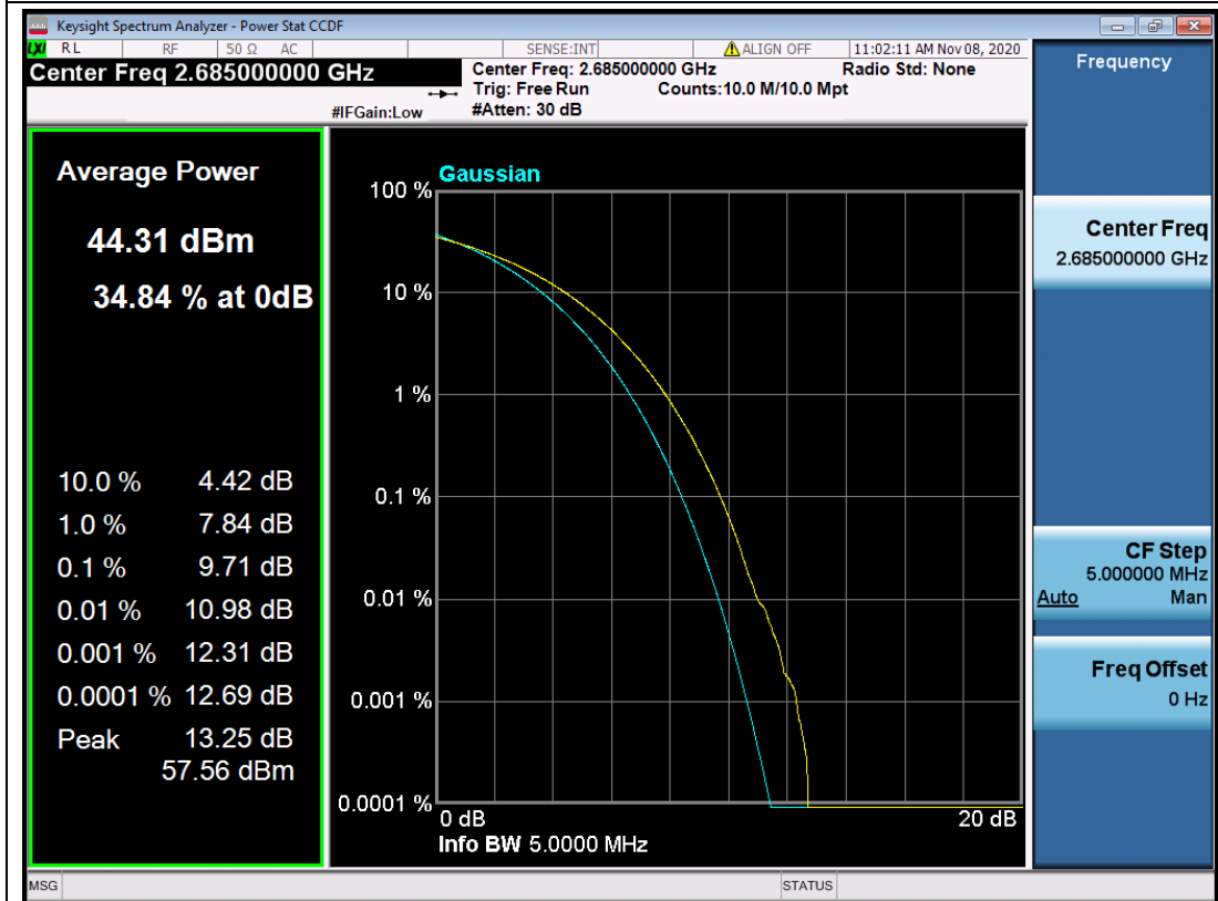
B41-10-PAPR-Q64-H.png
