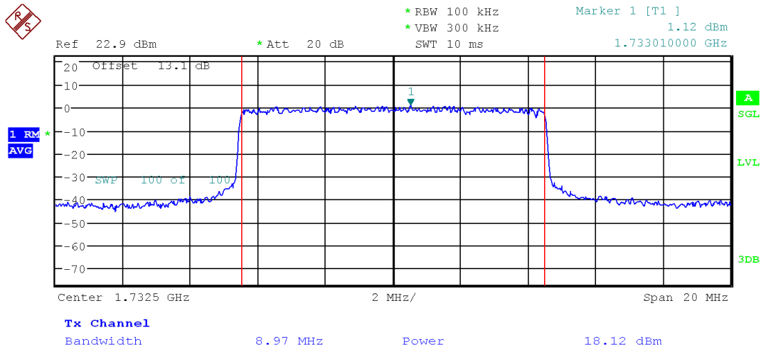
Figure 3: Average Power, Band 4 QPSK
