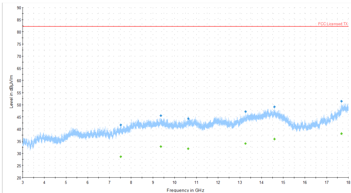
Figure 18: Radiated Spurious Emission 3GHz-18GHz – LTE Mid Channel band 66
