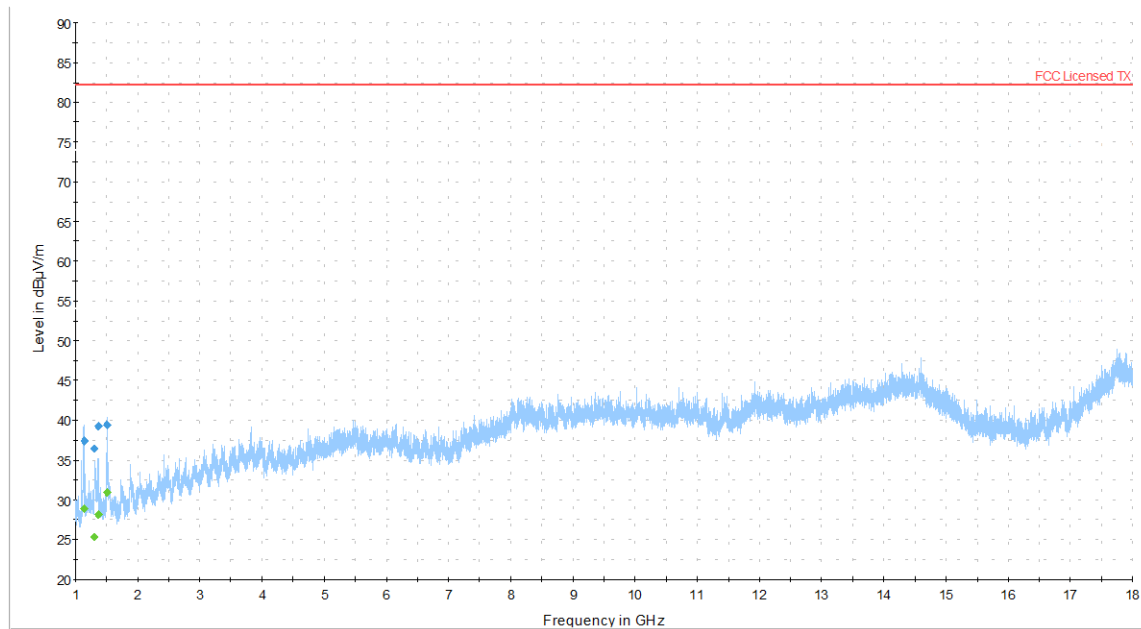
Figure 23: Radiated Spurious Emission 1GHz-18GHz – LTE Mid Channel band 71
