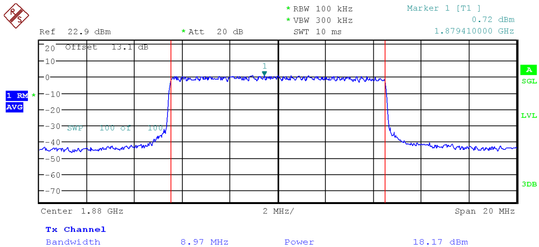
Figure 2: Average Power, Band 2 QPSK
