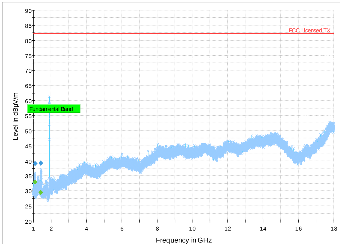
Figure 19: Radiated Spurious Emission 1GHz-18GHz – LTE Mid Channel band 2
