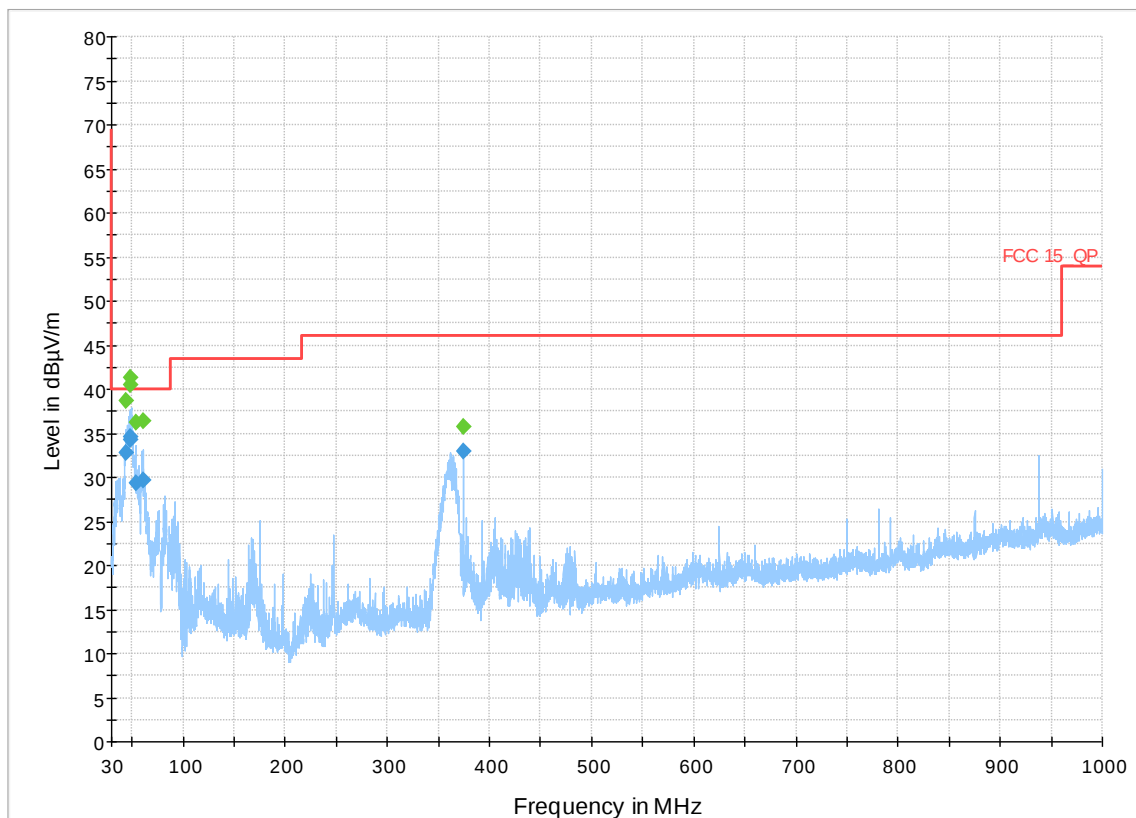
Figure 8: Radiated Spurious Emission 30MHz-1GHz – LTE Mid Channel band 2
