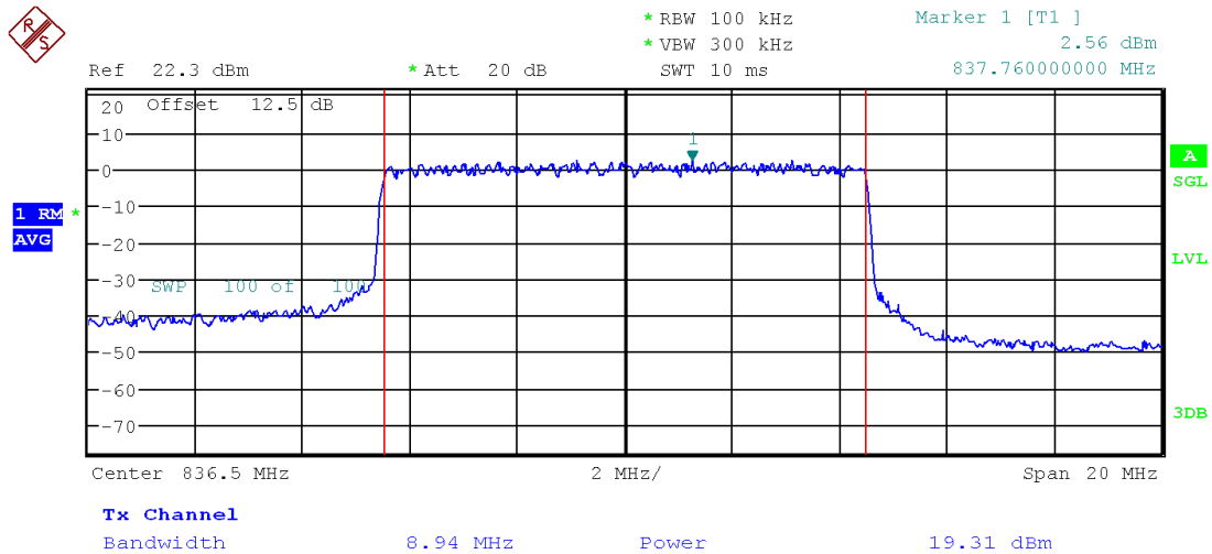
Figure 1: Average Power, Band 5 QPSK
