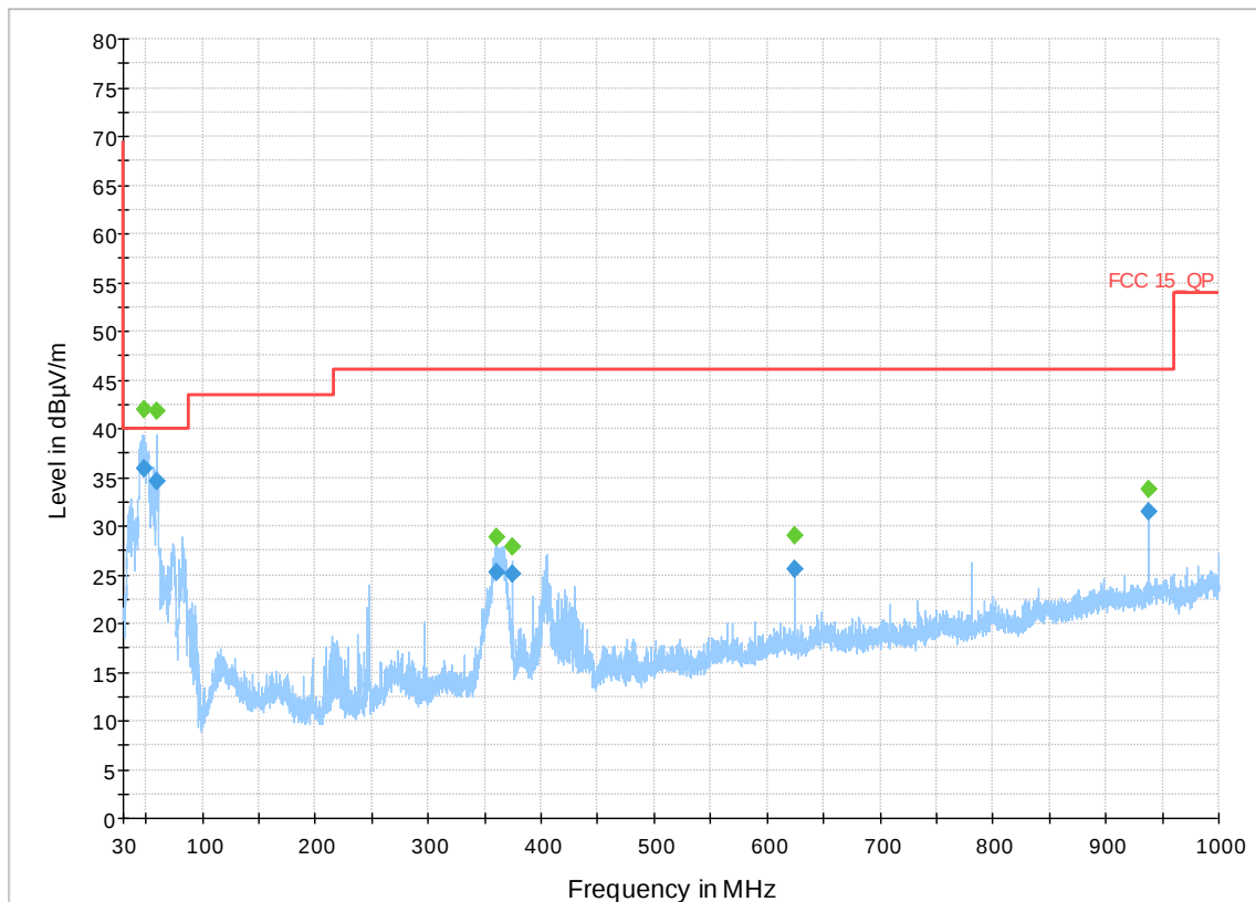
Figure 13: Radiated Spurious Emission 30MHz-1GHz – LTE Mid Channel band 66
