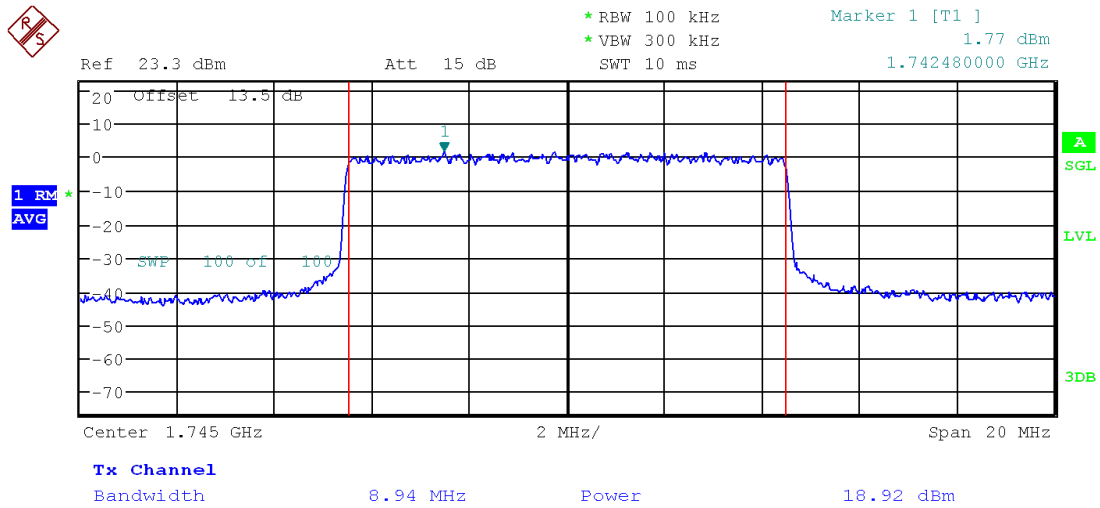
Figure 5: Average Power, Band 66 QPSK
