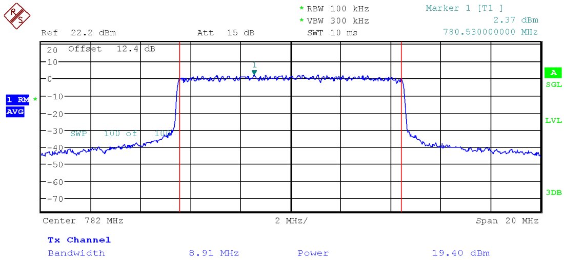
Figure 7: Average Power, Band 13 QPSK
