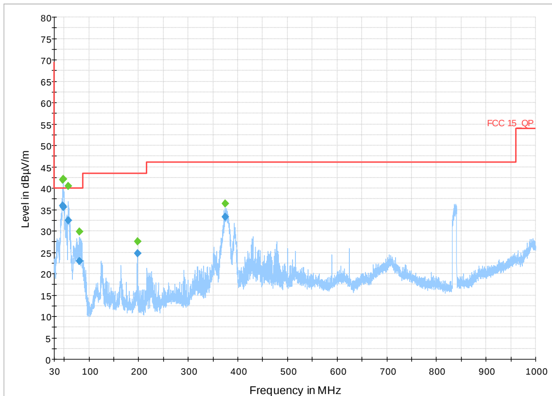
Figure 10: Radiated Spurious Emission 30MHz-1GHz – LTE Mid Channel band 5
