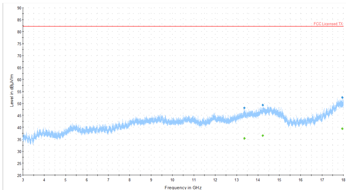
Figure 17: Radiated Spurious Emission 3GHz-18GHz – LTE Mid Channel band 4
