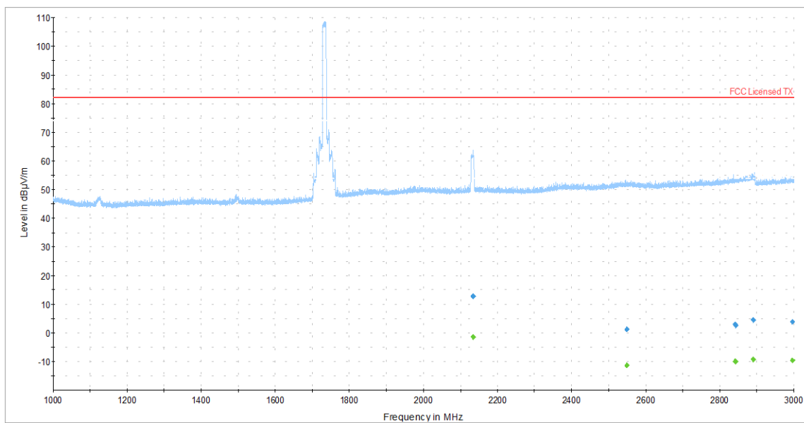
Figure 15: Radiated Spurious Emission 1GHz-3GHz – LTE Mid Channel band 4
