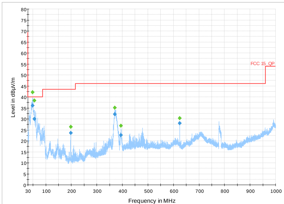
Figure 12: Radiated Spurious Emission 30MHz-1GHz – LTE Mid Channel band 13
