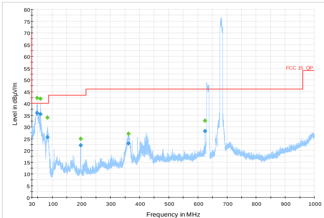
Figure 14: Radiated Spurious Emission 30MHz-1GHz – LTE Mid Channel band 71
