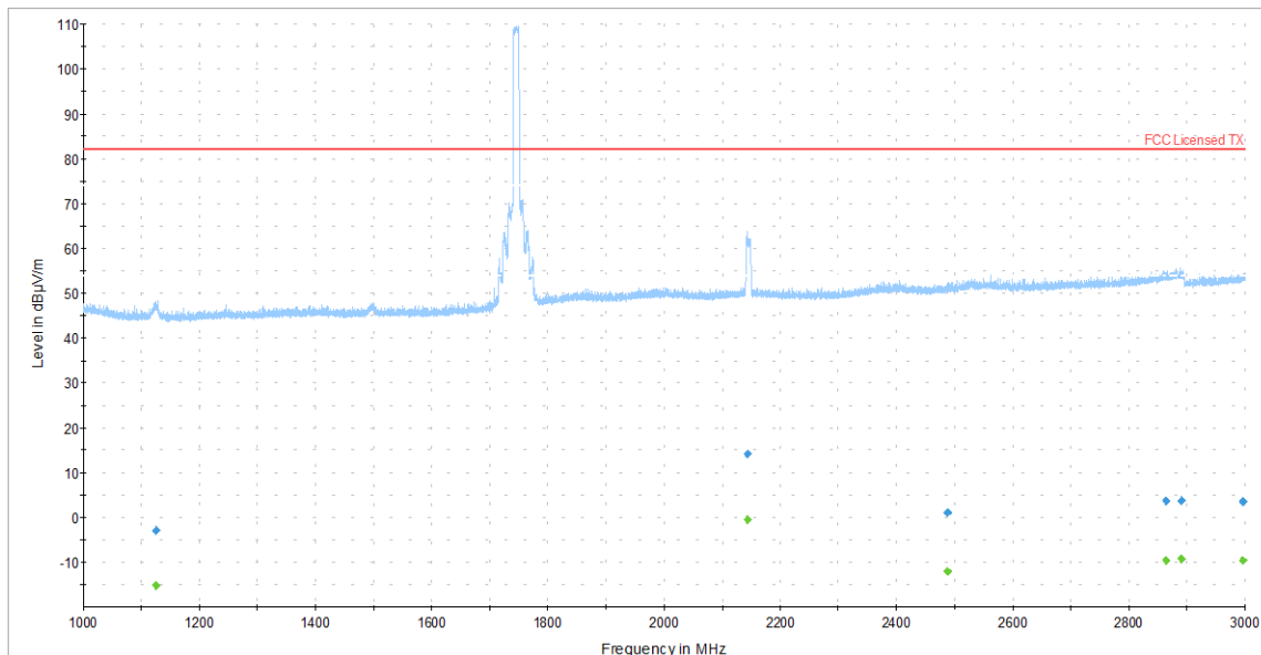
Figure 16: Radiated Spurious Emission 1GHz-3GHz – LTE Mid Channel band 66
