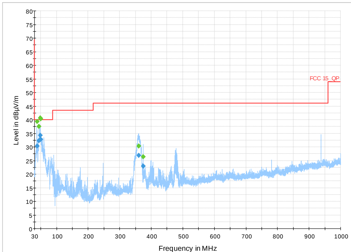
Figure 9: Radiated Spurious Emission 30MHz-1GHz – LTE Mid Channel band 4
