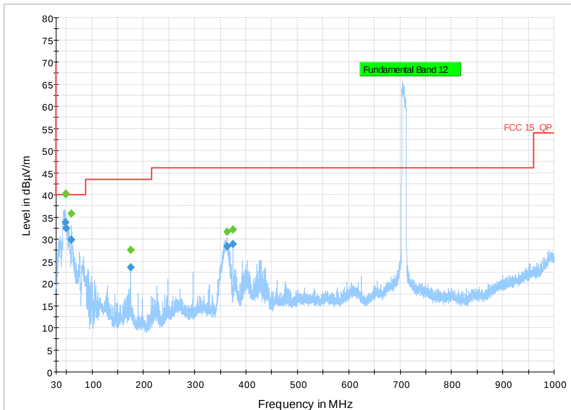
Figure 11: Radiated Spurious Emission 30MHz-1GHz – LTE Mid Channel band 12
