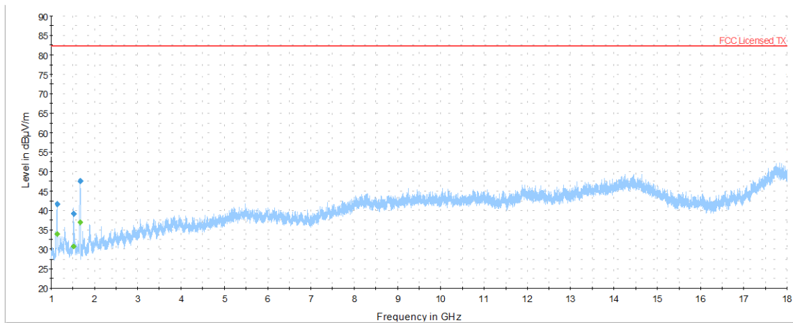
Figure 20: Radiated Spurious Emission 1GHz-18GHz – LTE Mid Channel band 5
