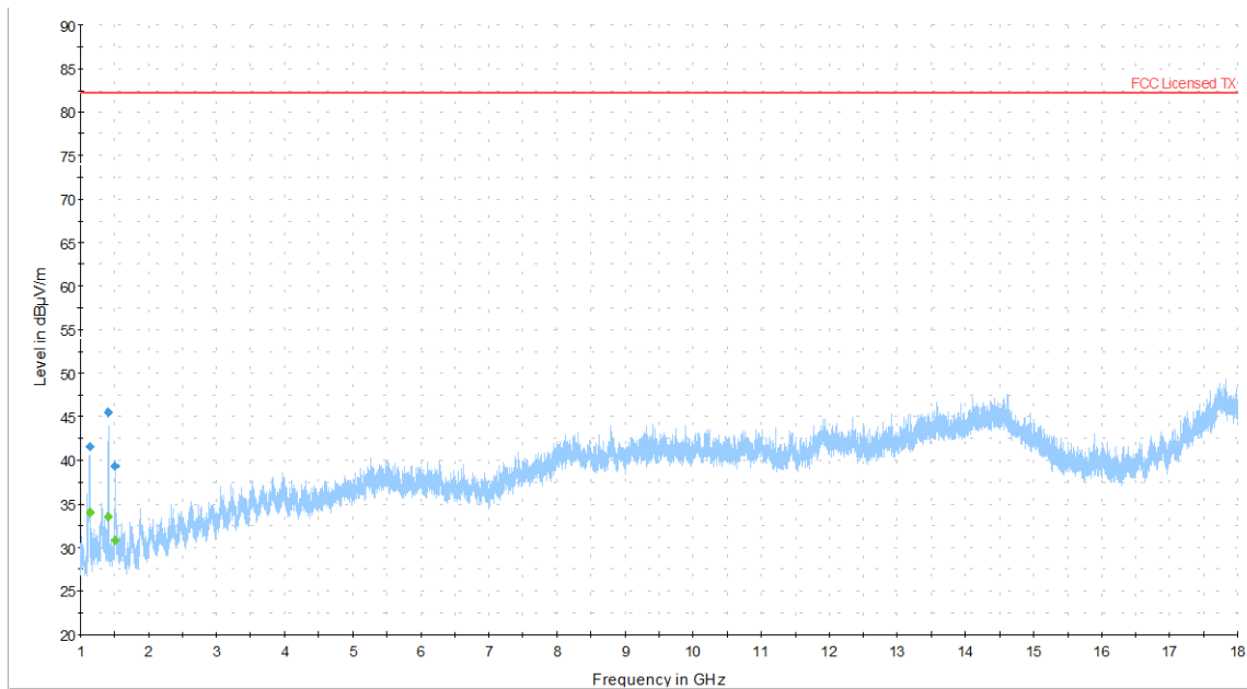
Figure 21: Radiated Spurious Emission 1GHz-18GHz – LTE Mid Channel band 12
