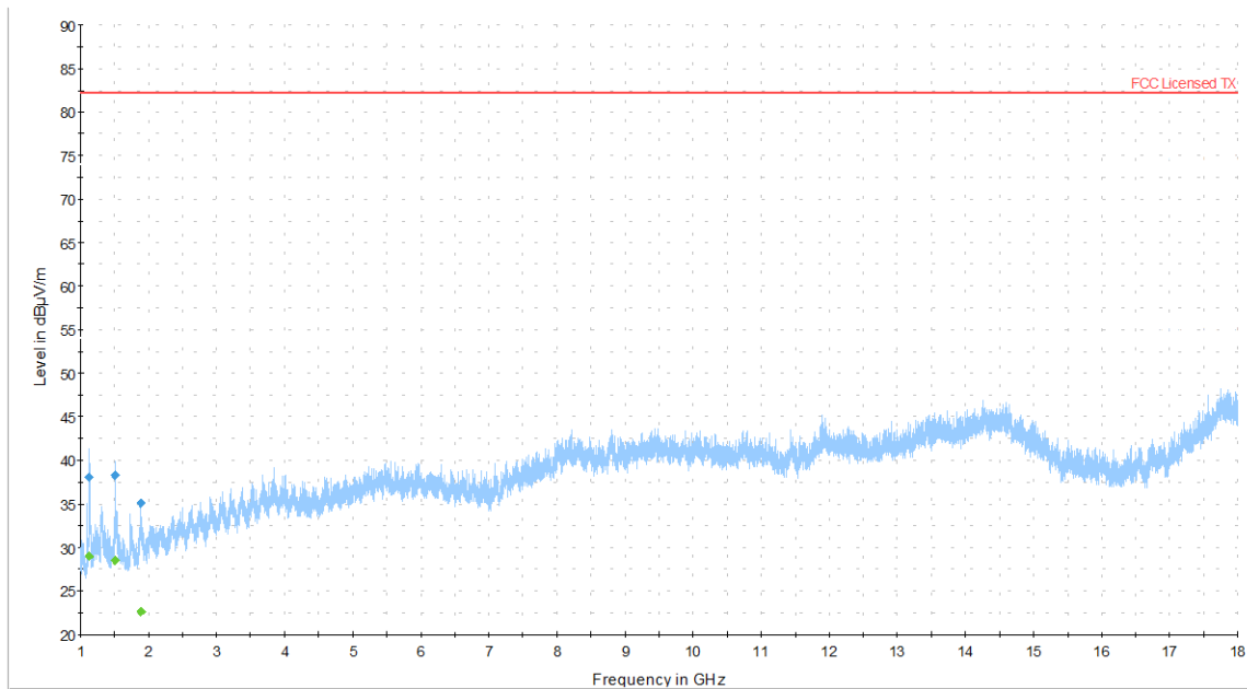
Figure 22: Radiated Spurious Emission 1GHz-18GHz – LTE Mid Channel band 13
