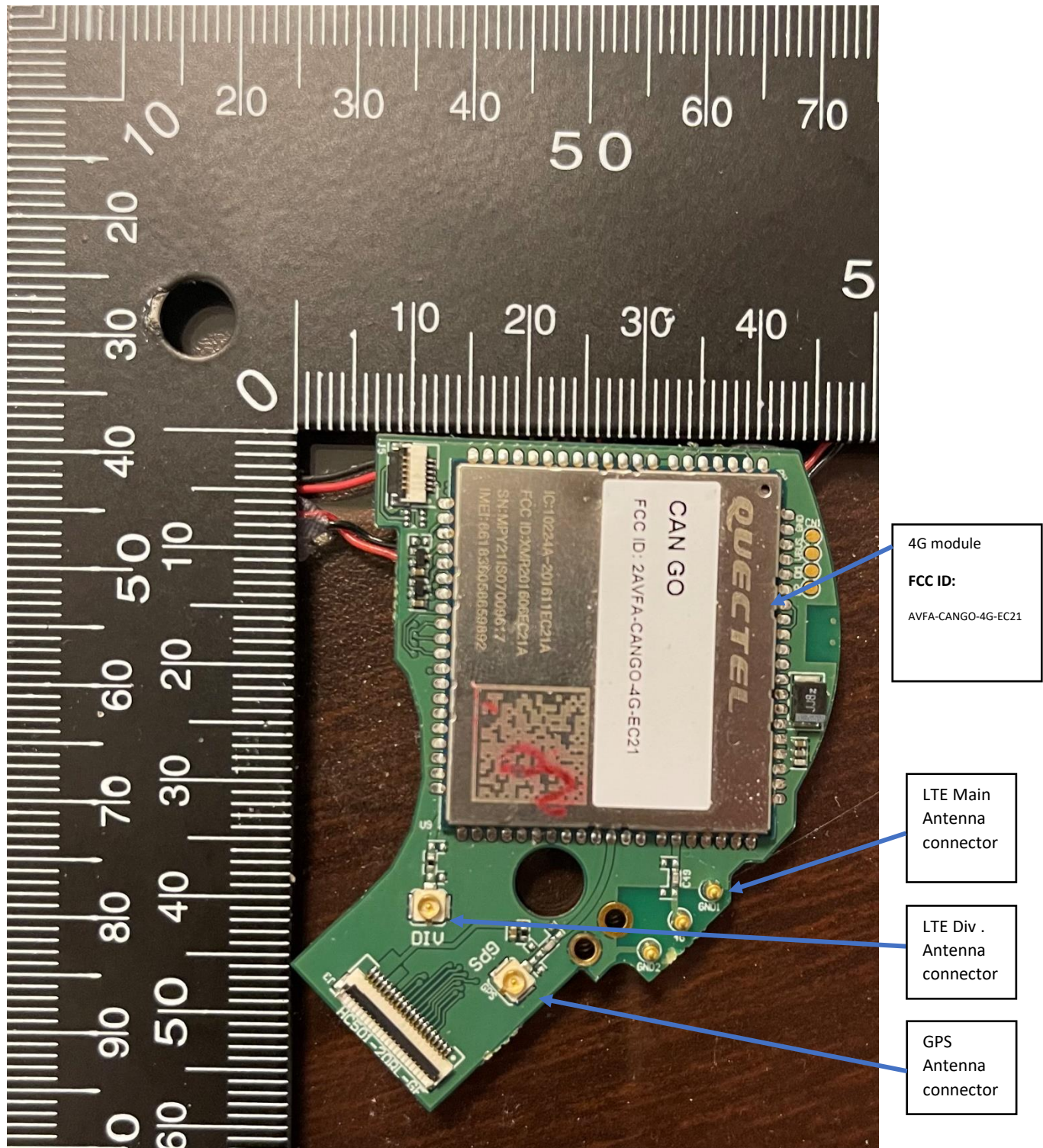
Fig 3: Main PCB - front (Zoom in)
