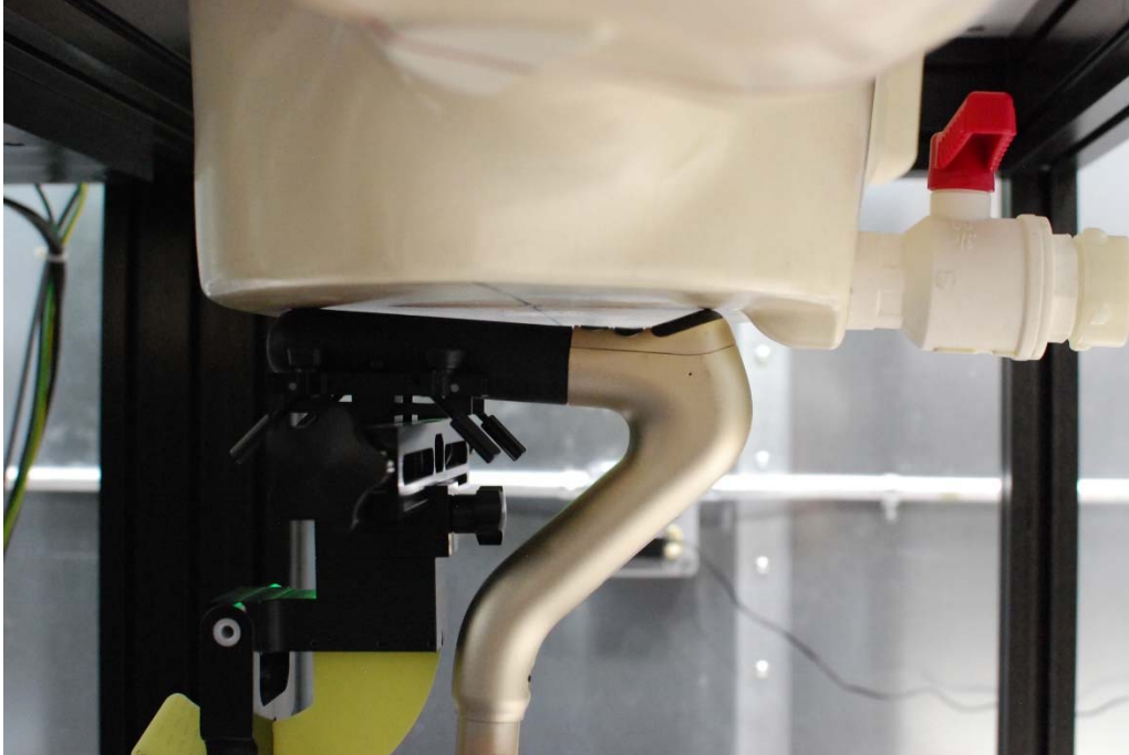
SAR Test Setup Photo 2 – Body, Top Side at 0mm
