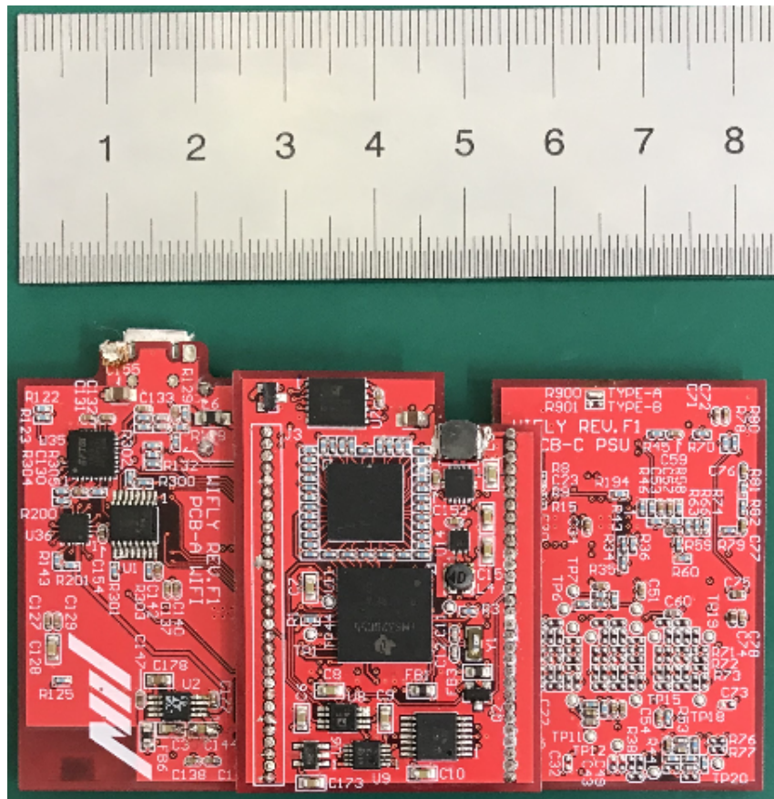
1 st Board
