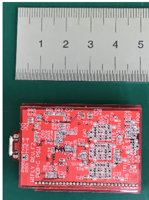
PCB_3: Bottom
