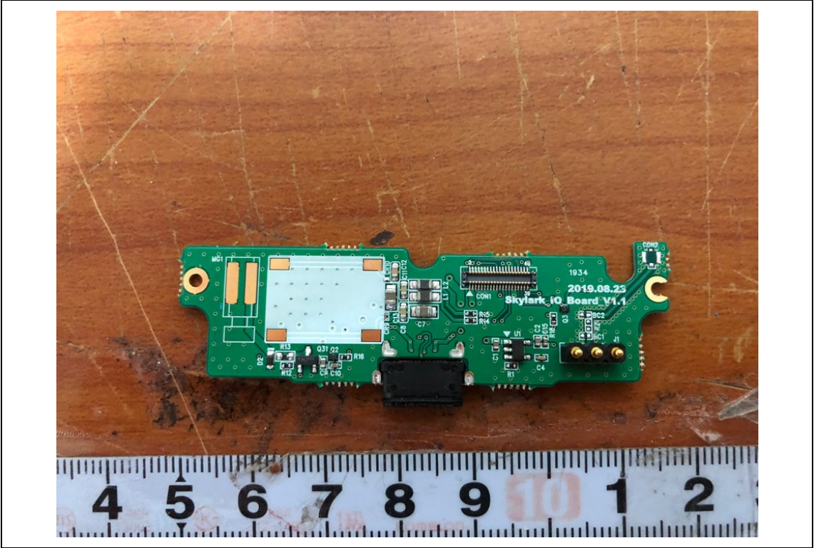
Module Board–Rear
