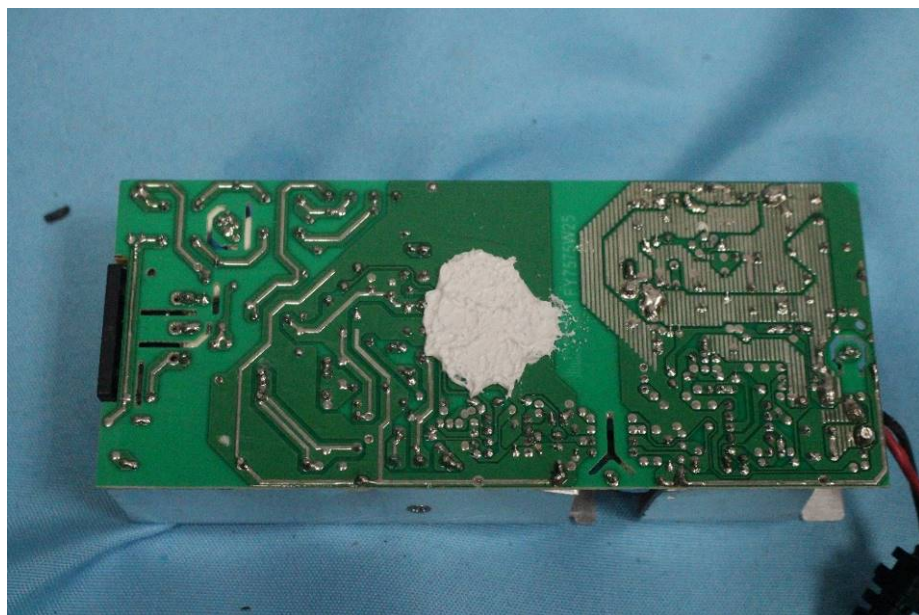
GH-A02 with of control PCB (Rev 1.5)
