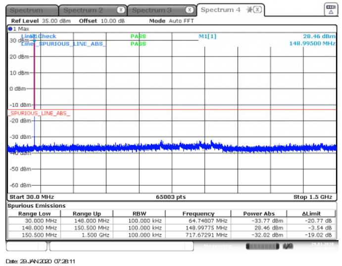
Figure 7.3.1.2-8: Conducted Spurious Emissions
