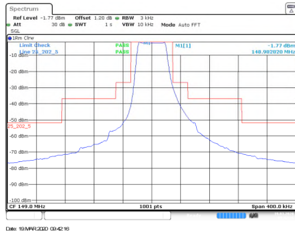
Figure 7.3.1.2-6: Emission Mask – BW5 (41.7kHz)
