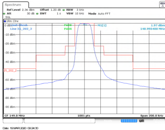
Figure 7.3.1.2-3: Emission Mask – BW2 (15.6kHz)
