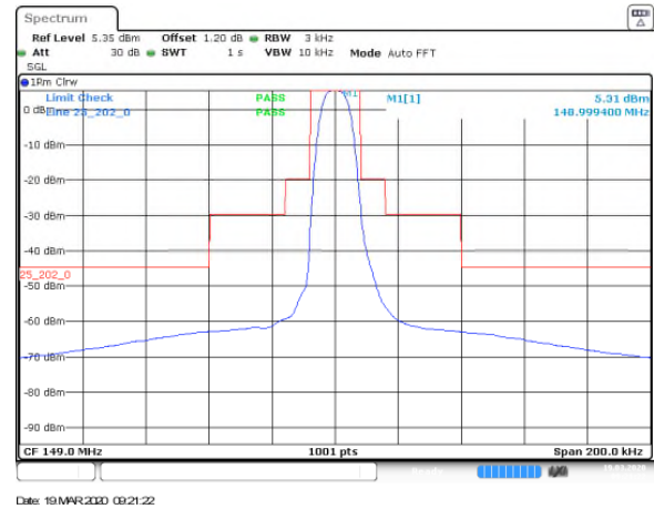
Figure 7.3.1.2-2: Emission Mask – BW1 (10.4kHz)
