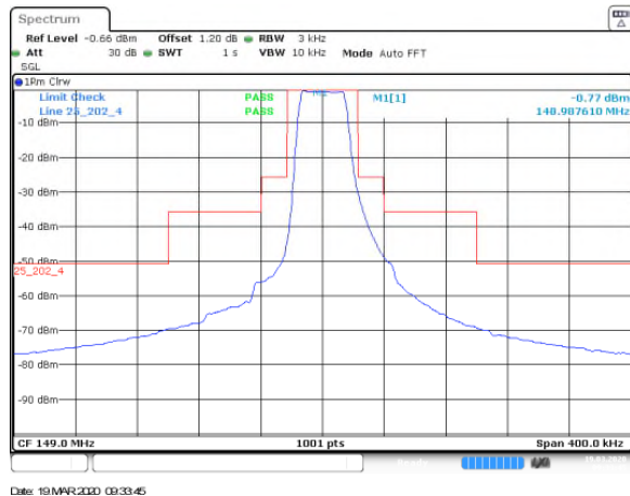
Figure 7.3.1.2-5: Emission Mask – BW4 (31.3kHz)
