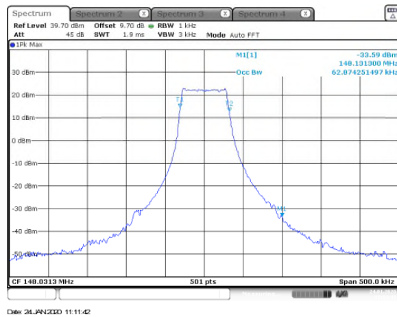
Figure 7.1.2-2: Sample Plot - 99% OBW (Highest BW Setting)
