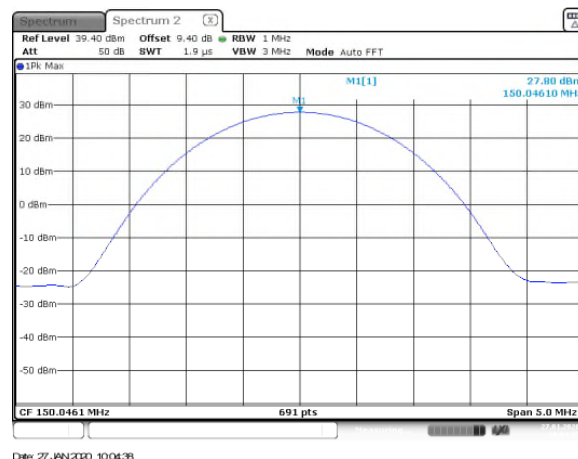
Figure 7.2.2-1: Conducted Output Power – Sample Plot
