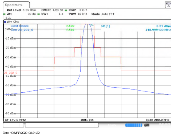
Figure 7.3.1.2-1: Emission Mask – BW0 (7.8kHz)
