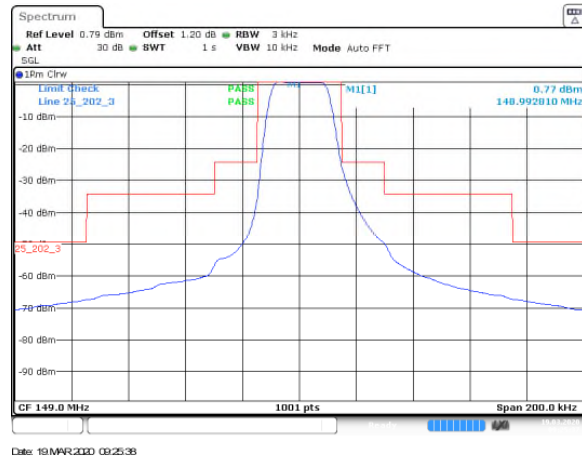
Figure 7.3.1.2-4: Emission Mask – BW3 (20.8kHz)
