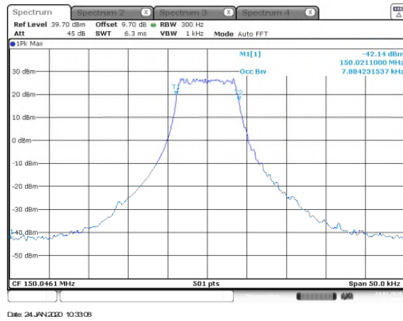
Figure 7.1.2-1: Sample Plot - 99% OBW (Lowest BW Setting)
