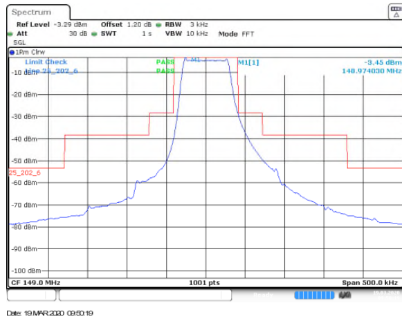
Figure 7.3.1.2-7: Emission Mask – BW6 (62.5kHz)
