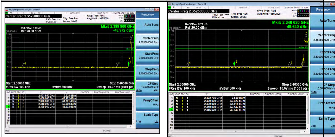
Channel 0 / 2402 MHz – Non-Hopping
