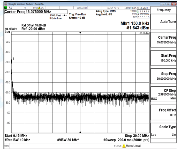
Band12-5MHz-16QAM-23155-1-0-High-0.15-30-0.15--51.64-28.64--23-PASS
