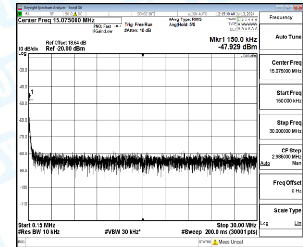
Band12-10MHz-QPSK-23130-1-0-High-0.15-30-0.15--47.93-24.93--23-PASS
