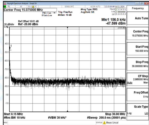
Band12-10MHz-16QAM-23095-1-0-Low-0.15-30-0.16--47.6-24.6--23-PASS
