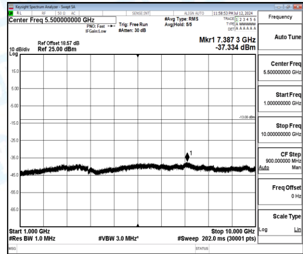
Band12-5MHz-16QAM-23035-1-0-Low-1000-10000-7387.3--37.33-24.33--13-PASS
