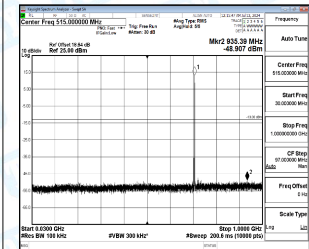
Band12-10MHz-QPSK-23130-1-0-High-30-1000-935.39--48.91-35.91--13-PASS
