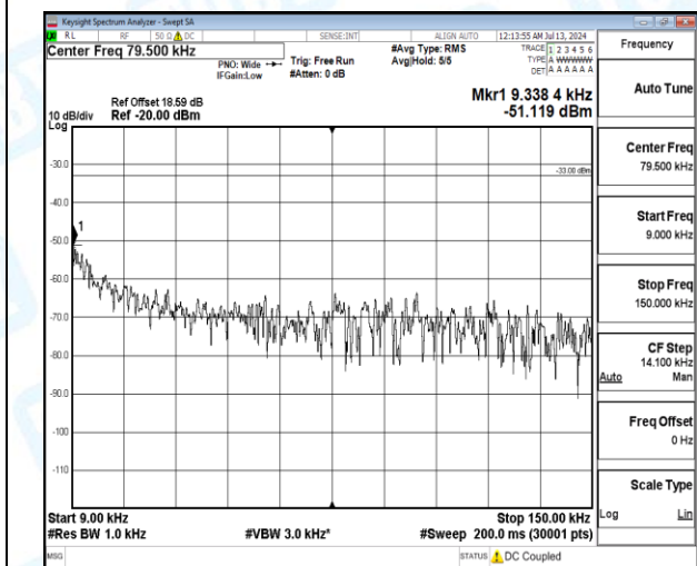
Band12-10MHz-16QAM-23060-1-0-Low-0.009-0.15-0.01--51.12-18.12--33-PASS
