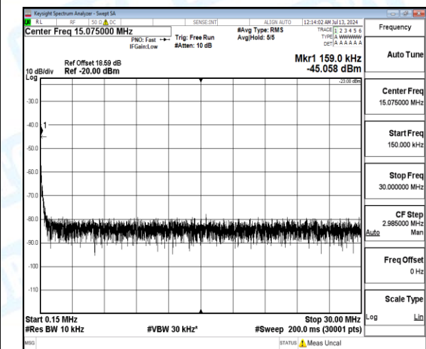
Band12-10MHz-16QAM-23060-1-0-Low-0.15-30-0.16--45.06-22.06--23-PASS
