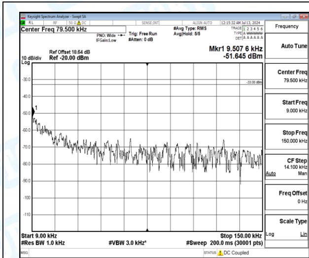
Band12-10MHz-QPSK-23130-1-0-High-0.009-0.15-0.01--51.65-18.65--33-PASS
