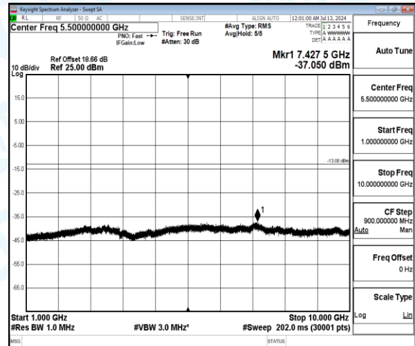
Band12-5MHz-16QAM-23155-1-0-High-1000-10000-7427.5--37.05-24.05--13-PASS
