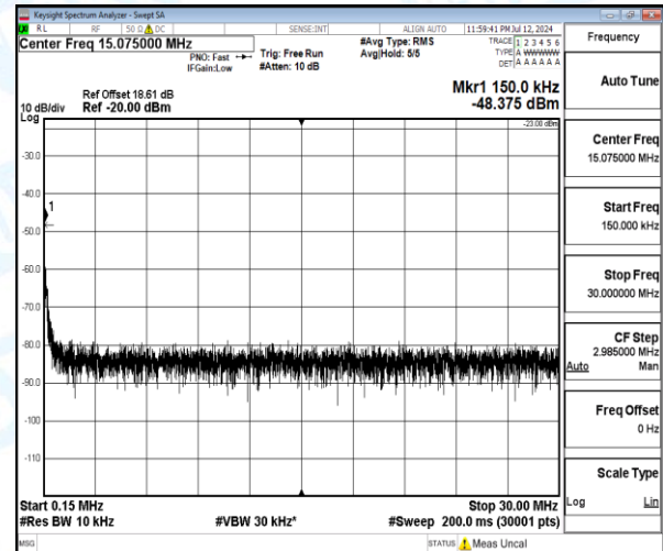
Band12-5MHz-16QAM-23095-1-0-Low-0.15-30-0.15--48.38-25.38--23-PASS
