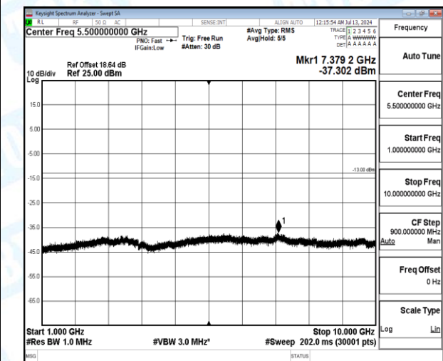
Band12-10MHz-QPSK-23130-1-0-High-1000-10000-7379.2--37.3-24.3--13-PASS
