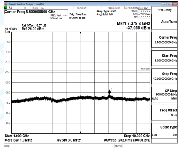
Band12-3MHz-QPSK-23165-1-0-High-1000-10000-7379.8--37.06-24.06--13-PASS
