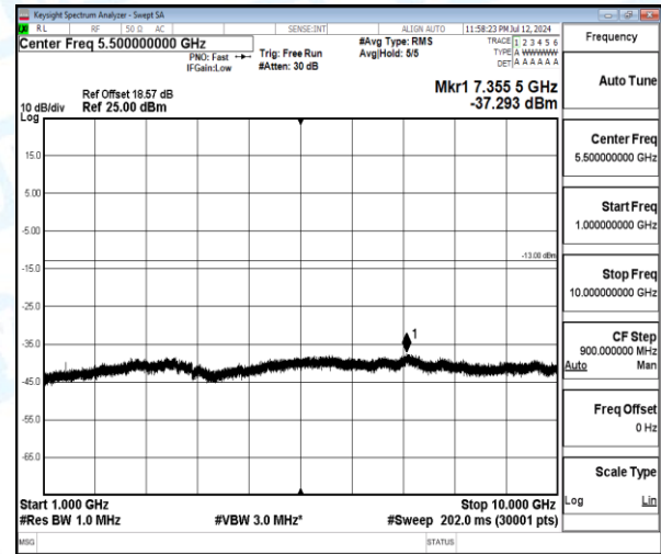
Band12-5MHz-QPSK-23035-1-0-Low-1000-10000-7355.5--37.29-24.29--13-PASS
