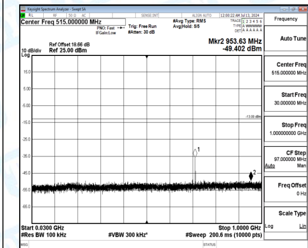
Band12-5MHz-QPSK-23155-1-0-High-30-1000-953.63--49.4-36.4--13-PASS
