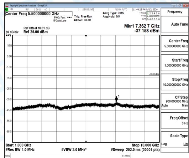
Band12-3MHz-16QAM-23095-1-0-Low-1000-10000-7362.7--37.16-24.16--13-PASS
