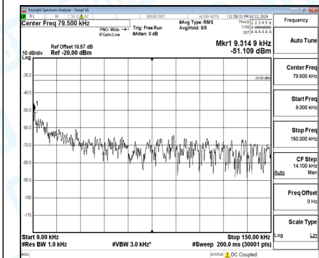
Band12-5MHz-16QAM-23035-1-0-Low-0.009-0.15-0.01--51.11-18.11--33-PASS
