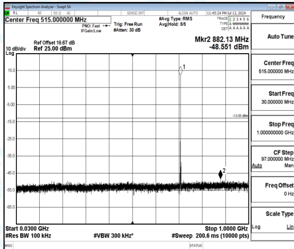
Band12-3MHz-16QAM-23165-1-0-High-30-1000-882.13--48.55-35.55--13-PASS
