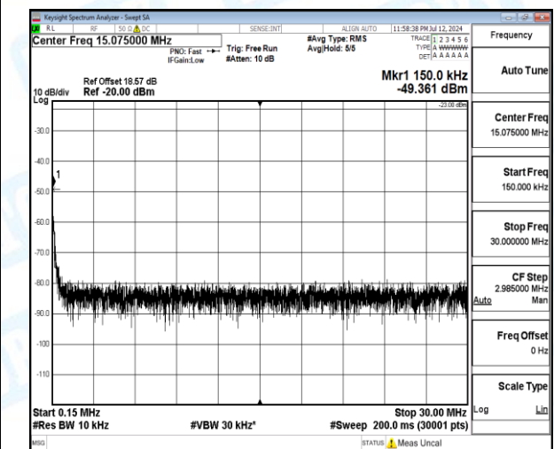
Band12-5MHz-16QAM-23035-1-0-Low-0.15-30-0.15--49.36-26.36--23-PASS
