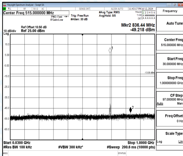
Band12-3MHz-16QAM-23025-1-0-Low-30-1000-836.44--49.22-36.22--13-PASS
