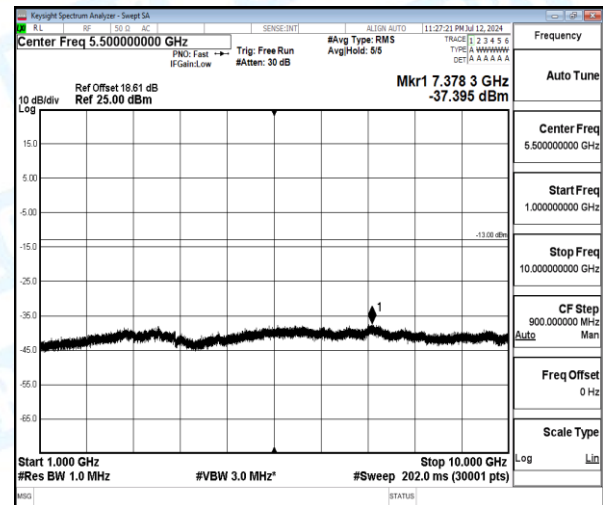
Band12-1.4MHz-QPSK-23095-1-0-Low-1000-10000-7378.3--37.4-24.4--13-PASS
