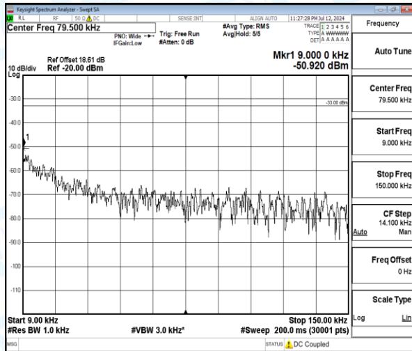
Band12-1.4MHz-16QAM-23095-1-0-Low-0.009-0.15-0.01--50.92-17.92--33-PASS
