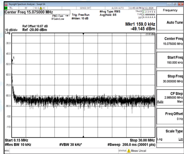
Band12-3MHz-16QAM-23165-1-0-High-0.15-30-0.16--49.15-26.15--23-PASS
