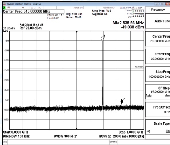
Band12-1.4MHz-16QAM-23017-1-0-Low-30-1000-839.93--49.04-36.04--13-PASS
