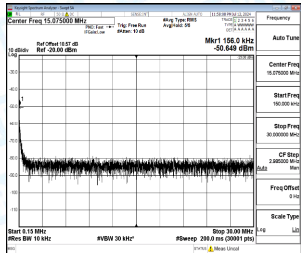
Band12-5MHz-QPSK-23035-1-0-Low-0.15-30-0.16--50.65-27.65--23-PASS
