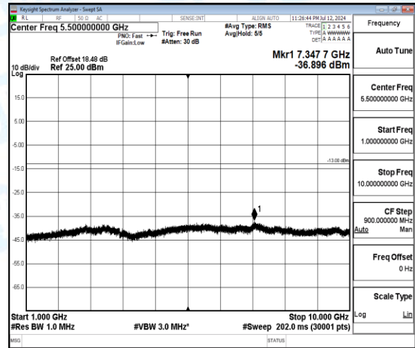
Band12-1.4MHz-16QAM-23017-1-0-Low-1000-10000-7347.7--36.9-23.9--13-PASS
