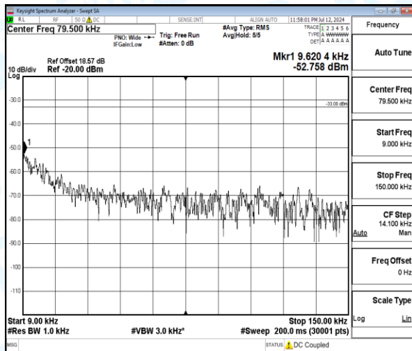
Band12-5MHz-QPSK-23035-1-0-Low-0.009-0.15-0.01--52.76-19.76--33-PASS
