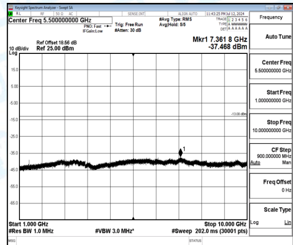
Band12-3MHz-16QAM-23025-1-0-Low-1000-10000-7361.8--37.47-24.47--13-PASS
