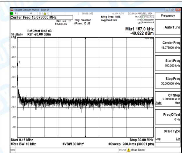
Band12-5MHz-QPSK-23155-1-0-High-0.15-30-0.16--49.82-26.82--23-PASS
