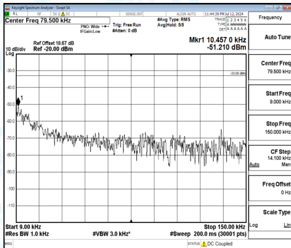
Band12-3MHz-QPSK-23165-1-0-High-0.009-0.15-0.01--51.21-18.21--33-PASS
