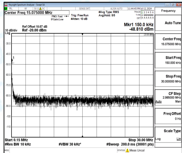
Band12-3MHz-QPSK-23165-1-0-High-0.15-30-0.15--48.81-25.81--23-PASS
