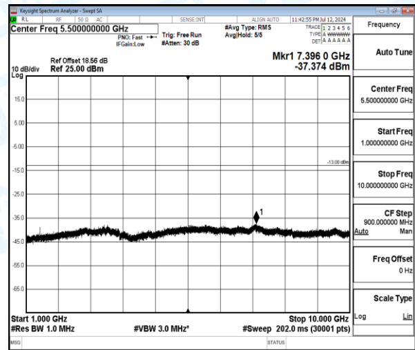
Band12-3MHz-QPSK-23025-1-0-Low-1000-10000-7396--37.37-24.37--13-PASS
