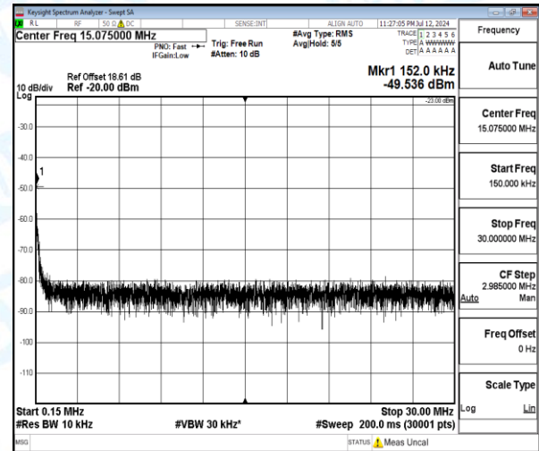
Band12-1.4MHz-QPSK-23095-1-0-Low-0.15-30-0.15--49.54-26.54--23-PASS
