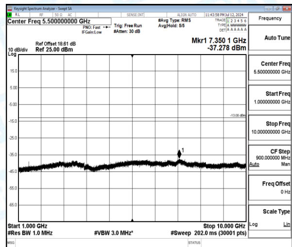
Band12-3MHz-QPSK-23095-1-0-Low-1000-10000-7350.1--37.28-24.28--13-PASS
