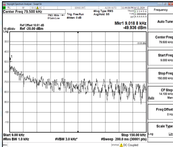
Band12-3MHz-16QAM-23095-1-0-Low-0.009-0.15-0.01--49.94-16.94--33-PASS
