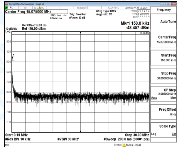
Band12-3MHz-16QAM-23095-1-0-Low-0.15-30-0.15--48.46-25.46--23-PASS
