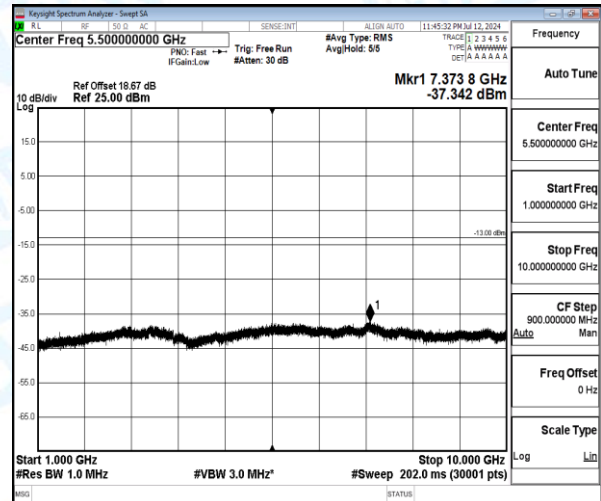
Band12-3MHz-16QAM-23165-1-0-High-1000-10000-7373.8--37.34-24.34--13-PASS
