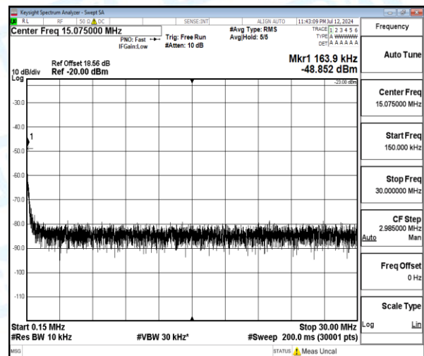
Band12-3MHz-16QAM-23025-1-0-Low-0.15-30-0.16--48.85-25.85--23-PASS
