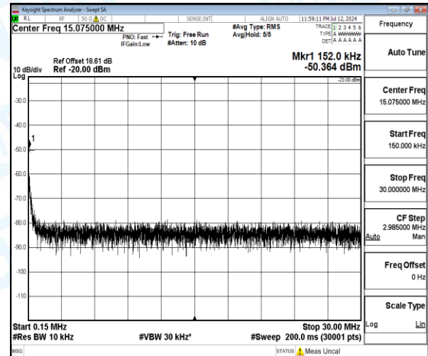
Band12-5MHz-QPSK-23095-1-0-Low-0.15-30-0.15--50.36-27.36--23-PASS
