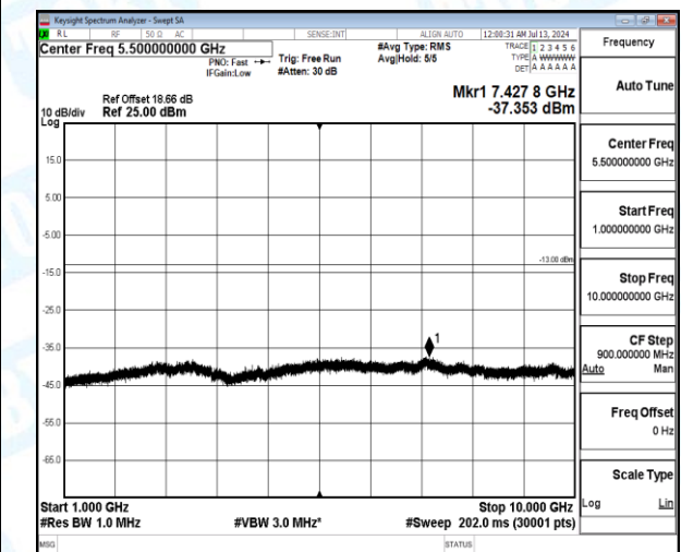
Band12-5MHz-QPSK-23155-1-0-High-1000-10000-7427.8--37.35-24.35--13-PASS
