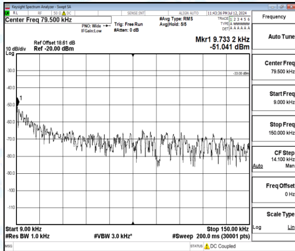
Band12-3MHz-QPSK-23095-1-0-Low-0.009-0.15-0.01--51.04-18.04--33-PASS
