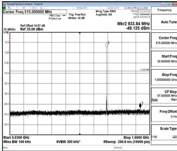
Band12-5MHz-QPSK-23035-1-0-Low-30-1000-933.84--49.13-36.13--13-PASS
