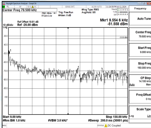
Band12-1.4MHz-QPSK-23095-1-0-Low-0.009-0.15-0.01--51.56-18.56--33-PASS
