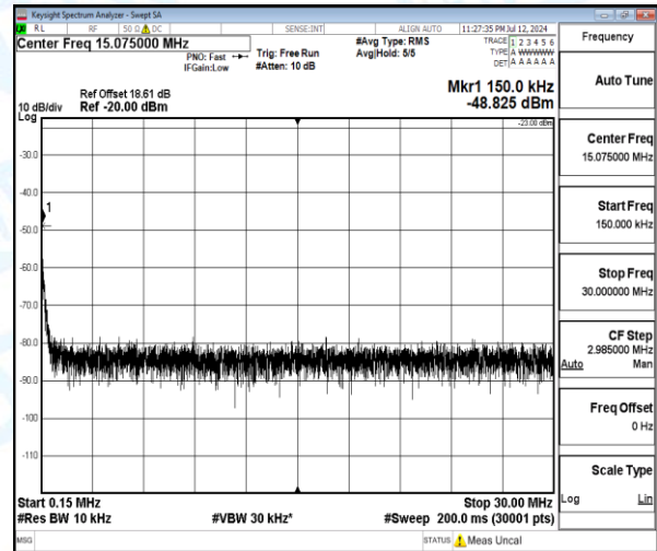
Band12-1.4MHz-16QAM-23095-1-0-Low-0.15-30-0.15--48.83-25.83--23-PASS
