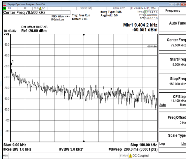
Band12-3MHz-16QAM-23165-1-0-High-0.009-0.15-0.01--50.55-17.55--33-PASS
