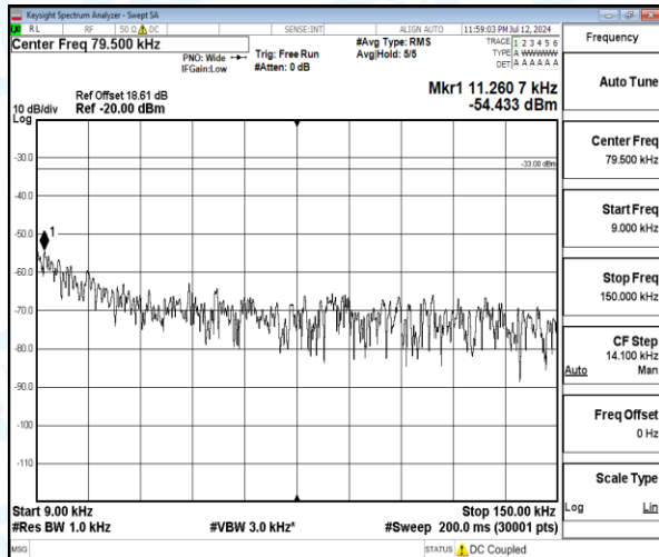
Band12-5MHz-QPSK-23095-1-0-Low-0.009-0.15-0.01--54.43-21.43--33-PASS
