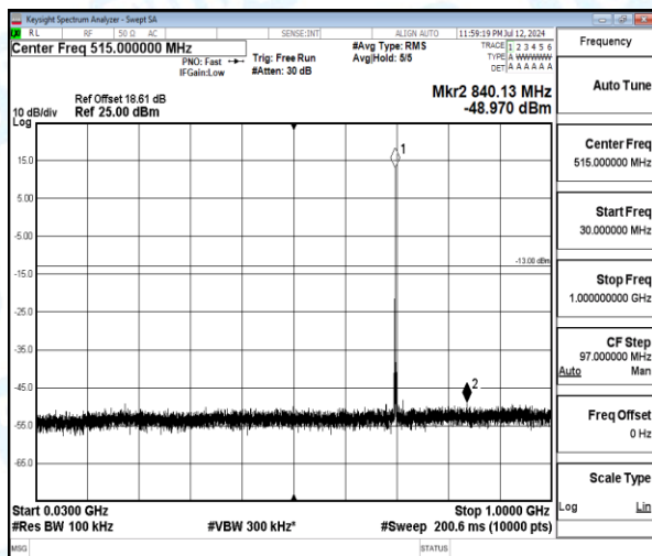
Band12-5MHz-QPSK-23095-1-0-Low-30-1000-840.13--48.97-35.97--13-PASS
