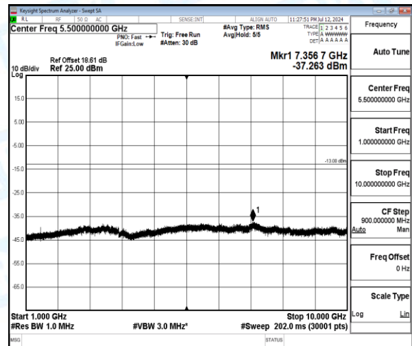
Band12-1.4MHz-16QAM-23095-1-0-Low-1000-10000-7356.7--37.26-24.26--13-PASS
