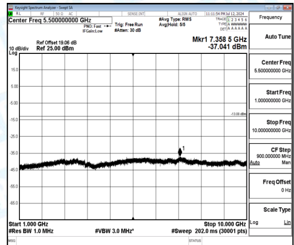
Band5-10MHz-16QAM-20525-1-0-Low-1000-10000-7358.5--37.04-24.04--13-PASS
