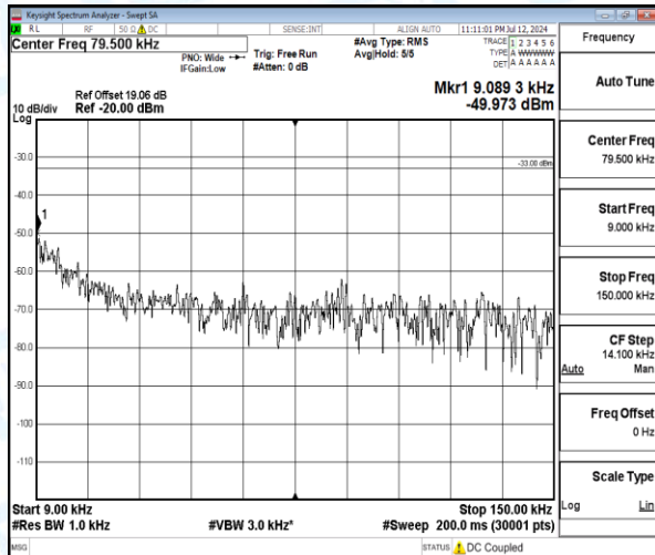
Band5-10MHz-QPSK-20525-1-0-Low-0.009-0.15-0.01--49.97-16.97--33-PASS
