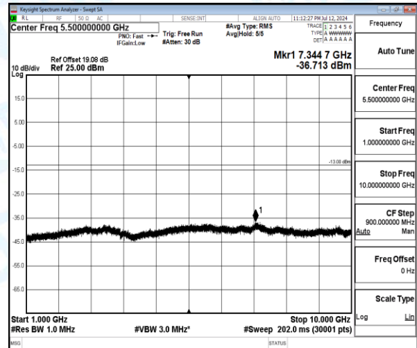
Band5-10MHz-QPSK-20600-1-0-High-1000-10000-7344.7--36.71-23.71--13-PASS
