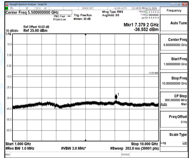
Band5-10MHz-16QAM-20450-1-0-Low-1000-10000-7379.2--36.55-23.55--13-PASS
