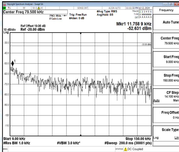
Band5-10MHz-16QAM-20525-1-0-Low-0.009-0.15-0.01--52.63-19.63--33-PASS
