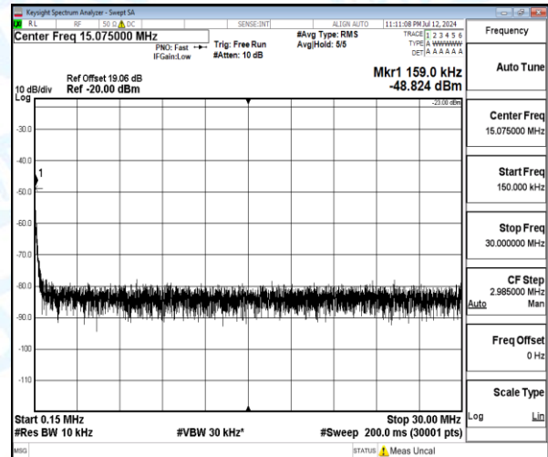
Band5-10MHz-QPSK-20525-1-0-Low-0.15-30-0.16--48.82-25.82--23-PASS
