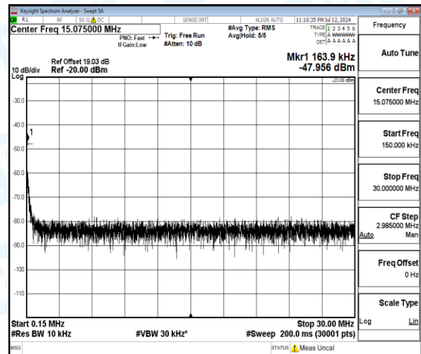
Band5-10MHz-16QAM-20450-1-0-Low-0.15-30-0.16--47.96-24.96--23-PASS
