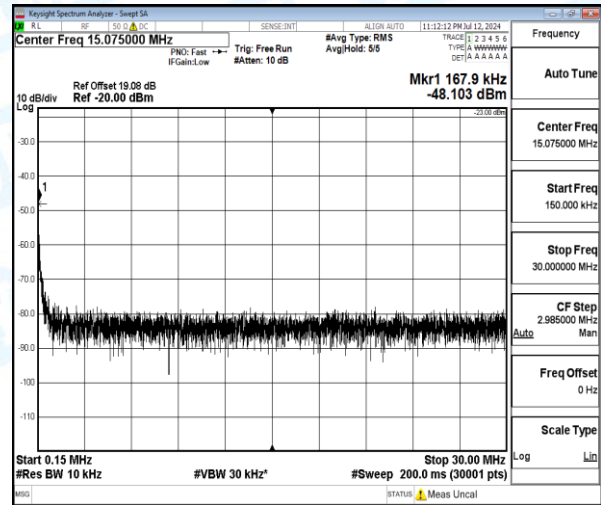
Band5-10MHz-QPSK-20600-1-0-High-0.15-30-0.17--48.1-25.1--23-PASS
