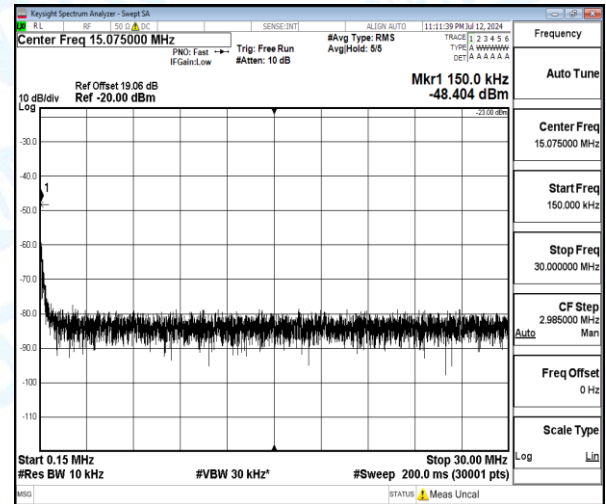
Band5-10MHz-16QAM-20525-1-0-Low-0.15-30-0.15--48.4-25.4--23-PASS
