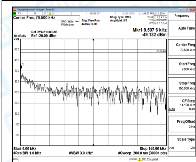
Band5-10MHz-QPSK-20450-1-0-Low-0.009-0.15-0.01--49.13-16.13--33-PASS
