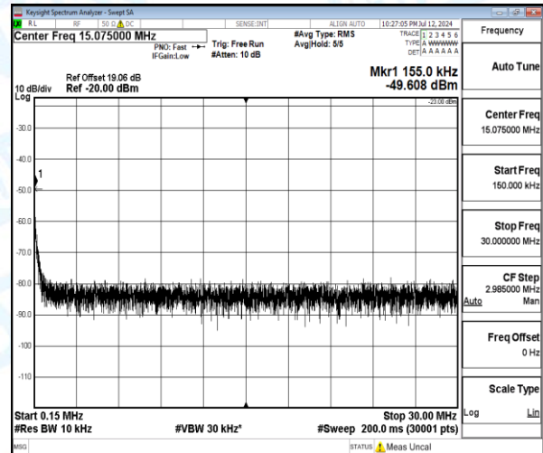
Band5-1.4MHz-16QAM-20525-1-0-Low-0.15-30-0.15--49.61-26.61--23-PASS
