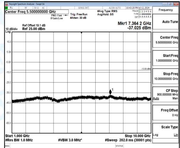
Band5-3MHz-16QAM-20635-1-0-High-1000-10000-7364.2--37.03-24.03--13-PASS
