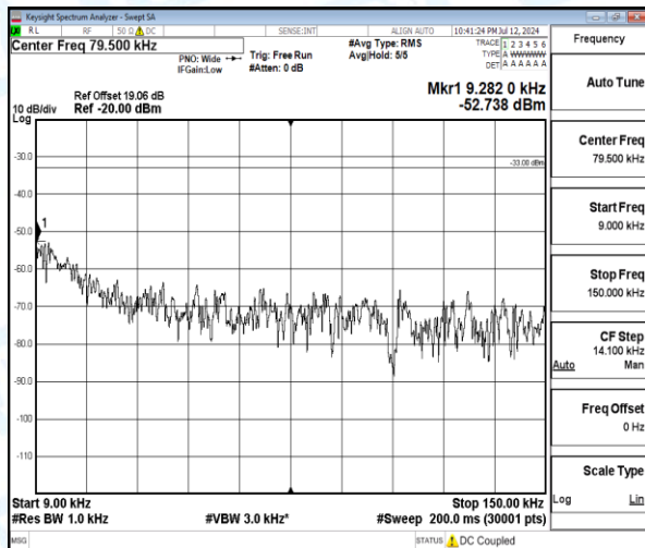
Band5-3MHz-QPSK-20525-1-0-Low-0.009-0.15-0.01--52.74-19.74--33-PASS
