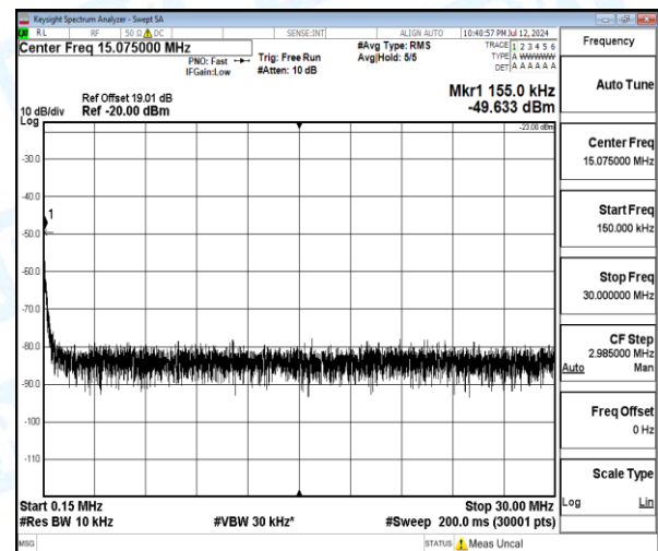
Band5-3MHz-16QAM-20415-1-0-Low-0.15-30-0.15--49.63-26.63--23-PASS
