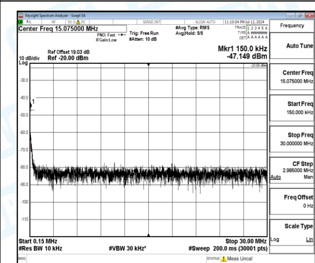
Band5-10MHz-QPSK-20450-1-0-Low-0.15-30-0.15--47.15-24.15--23-PASS
