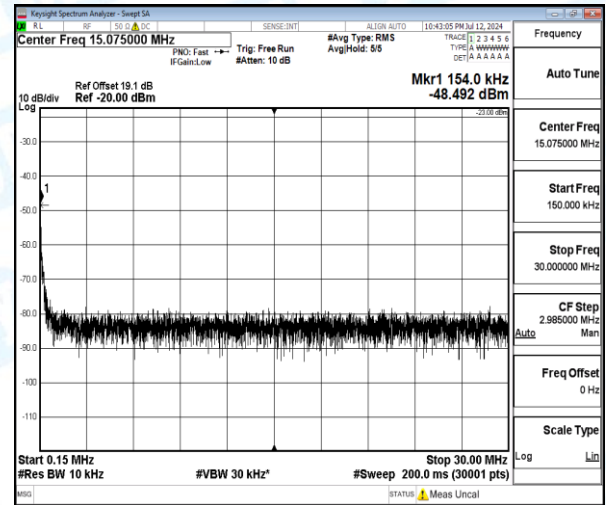
Band5-3MHz-16QAM-20635-1-0-High-0.15-30-0.15--48.49-25.49--23-PASS
