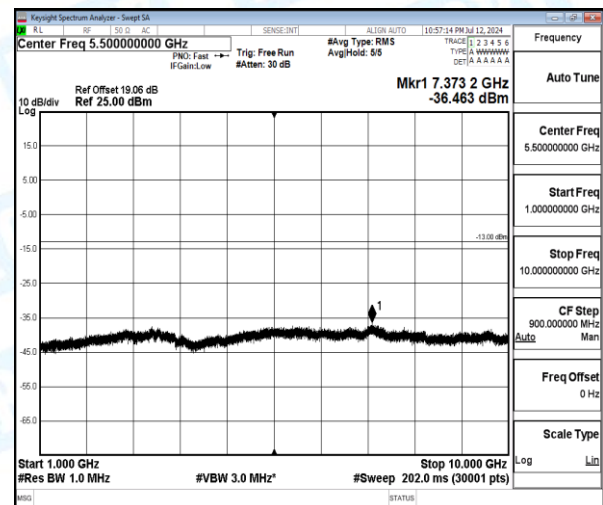
Band5-5MHz-16QAM-20525-1-0-Low-1000-10000-7373.2--36.46-23.46--13-PASS
