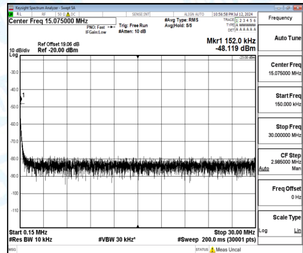
Band5-5MHz-16QAM-20525-1-0-Low-0.15-30-0.15--48.12-25.12--23-PASS
