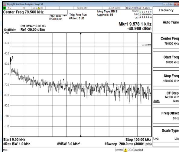
Band5-1.4MHz-16QAM-20525-1-0-Low-0.009-0.15-0.01--48.97-15.97--33-PASS
