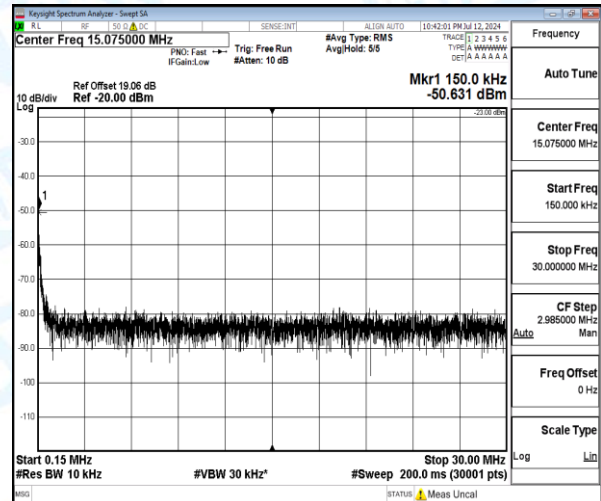
Band5-3MHz-16QAM-20525-1-0-Low-0.15-30-0.15--50.63-27.63--23-PASS
