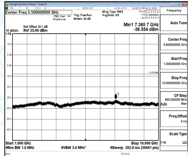
Band5-3MHz-QPSK-20635-1-0-High-1000-10000-7365.7--36.55-23.55--13-PASS
