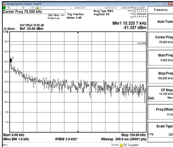
Band5-3MHz-16QAM-20525-1-0-Low-0.009-0.15-0.01--51.36-18.36--33-PASS
