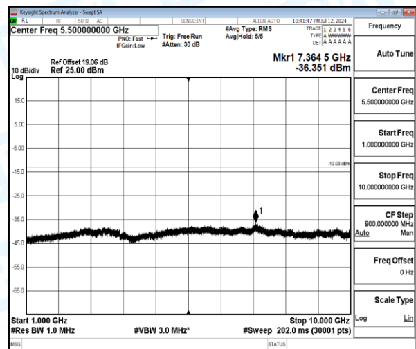
Band5-3MHz-QPSK-20525-1-0-Low-1000-10000-7364.5--36.35-23.35--13-PASS
