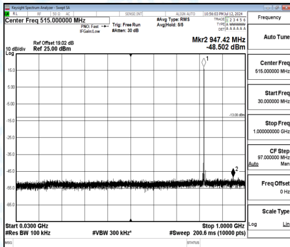
Band5-5MHz-16QAM-20425-1-0-Low-30-1000-947.42--48.5-35.5--13-PASS
