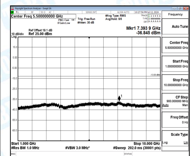
Band5-1.4MHz-QPSK-20643-1-0-High-1000-10000-7393.9--36.85-23.85--13-PASS
