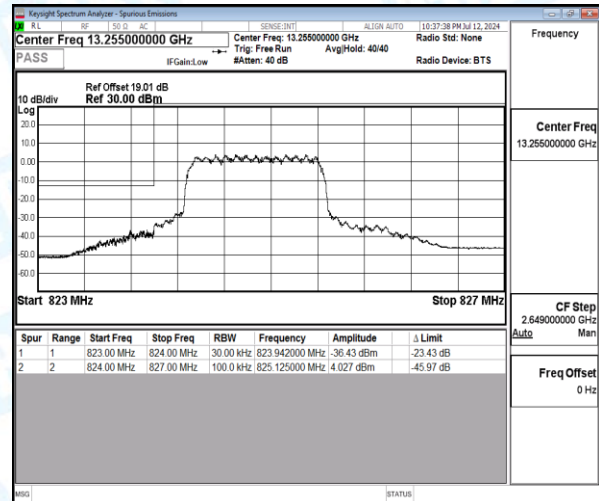
Band5-3MHz-16QAM-20415-6-0-Low-823.94--36.43-23.43-PASS
