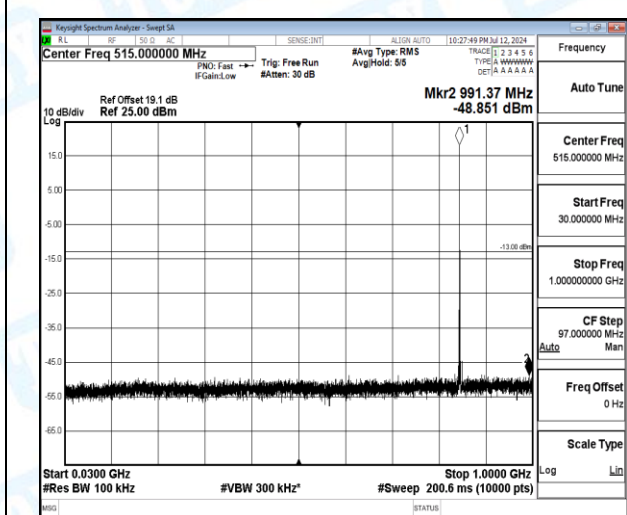
Band5-1.4MHz-QPSK-20643-1-0-High-30-1000-991.37--48.85-35.85--13-PASS
