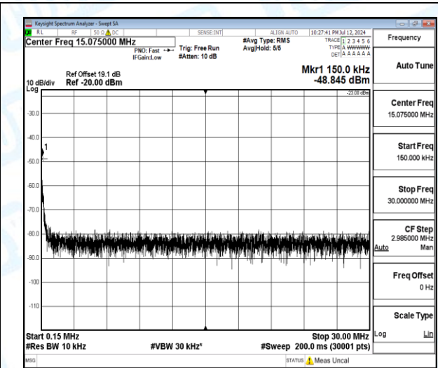
Band5-1.4MHz-QPSK-20643-1-0-High-0.15-30-0.15--48.85-25.85--23-PASS
