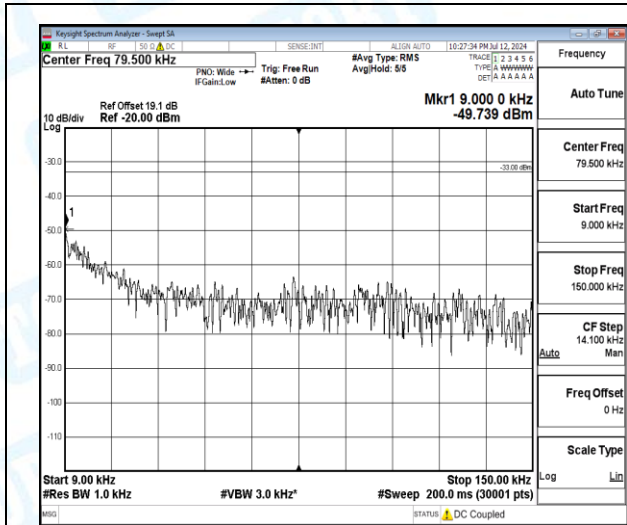
Band5-1.4MHz-QPSK-20643-1-0-High-0.009-0.15-0.01--49.74-16.74--33-PASS
