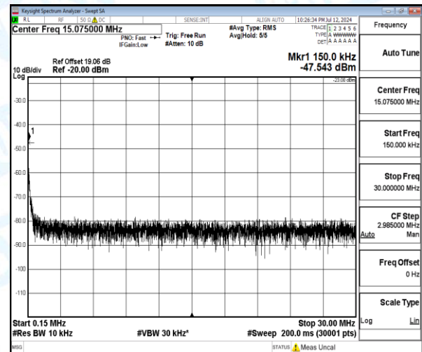
Band5-1.4MHz-QPSK-20525-1-0-Low-0.15-30-0.15--47.54-24.54--23-PASS
