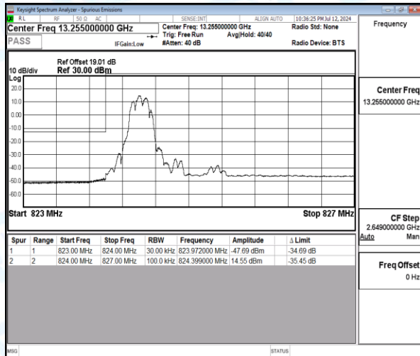
Band5-3MHz-16QAM-20415-1-0-Low-823.97--47.69-34.69-PASS
