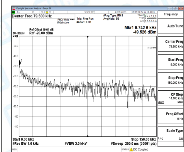
Band5-1.4MHz-16QAM-20407-1-0-Low-0.009-0.15-0.01--49.53-16.53--33-PASS
