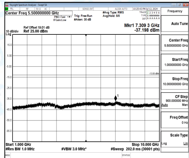
Band5-1.4MHz-QPSK-20407-1-0-Low-1000-10000-7309.3--37.2-24.2--13-PASS
