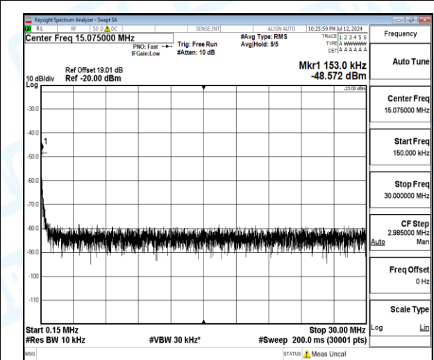
Band5-1.4MHz-16QAM-20407-1-0-Low-0.15-30-0.15--48.57-25.57--23-PASS
