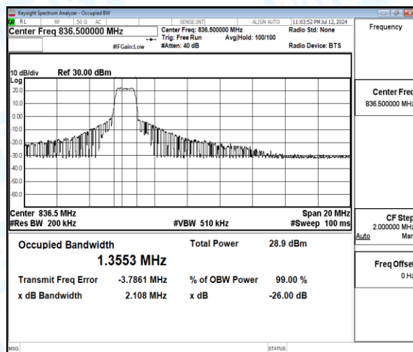
Band5-10MHz-QPSK-20525-6-0-Low-1.3553-2.108-PASS
