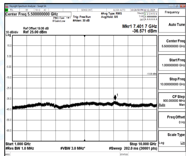
Band5-1.4MHz-QPSK-20525-1-0-Low-1000-10000-7401.7--36.57-23.57--13-PASS
