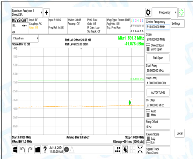
Band4-3MHz-QPSK-20385-1-0-High-30-1000-891.25--41.08-28.08--13-PASS
