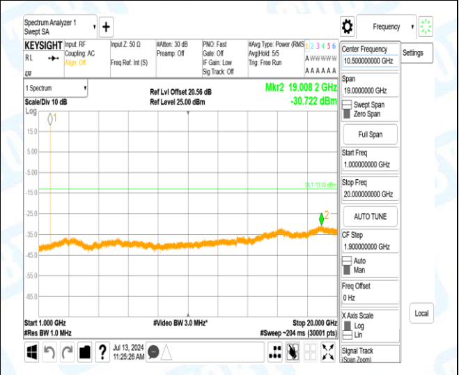
Band4-3MHz-QPSK-20175-1-0-Low-1000-20000-19008.2--30.72-17.72--13-PASS
