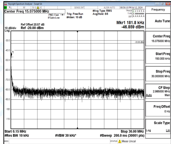
Band4-5MHz-16QAM-19975-1-0-Low-0.15-30-0.18--46.86-13.86--33-PASS
