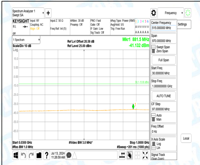
Band4-3MHz-16QAM-20385-1-0-High-30-1000-881.54--41.13-28.13--13-PASS
