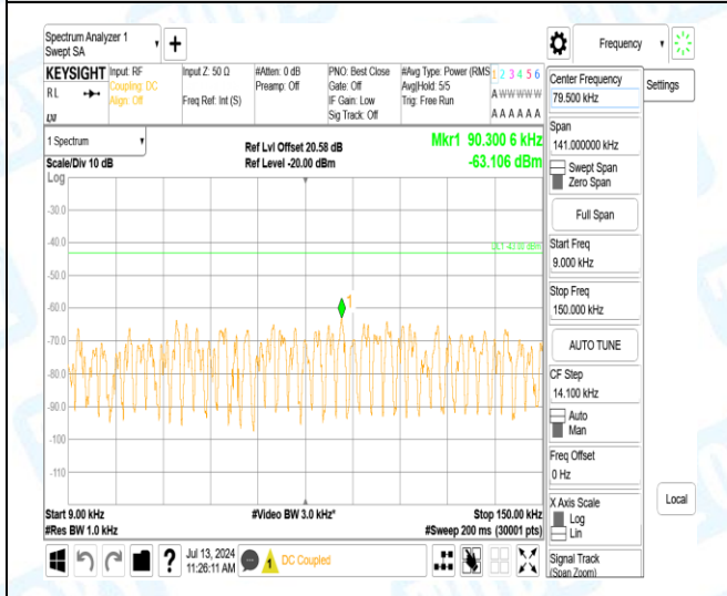
Band4-3MHz-QPSK-20385-1-0-High-0.009-0.15-0.09--63.11-20.11--43-PASS
