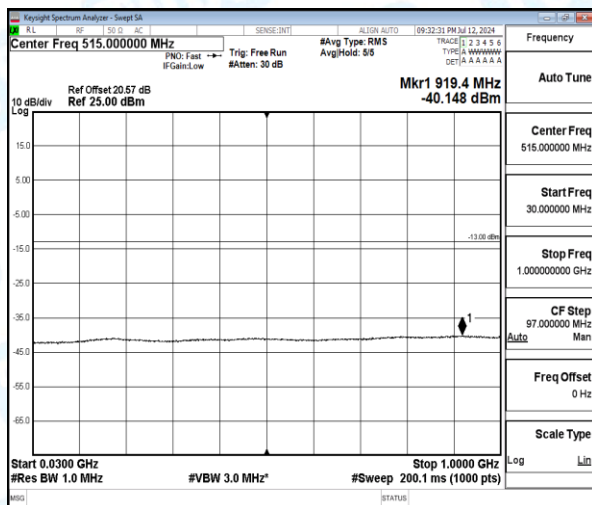
Band4-10MHz-16QAM-20000-1-0-Low-30-1000-919.41--40.15-27.15--13-PASS
