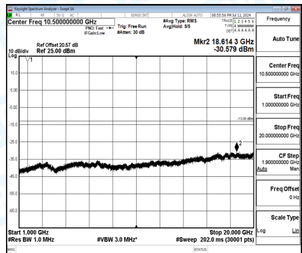
Band4-5MHz-QPSK-19975-1-0-Low-1000-20000-18614.27--30.58-17.58--13-PASS
