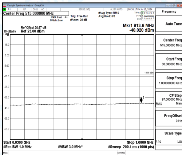
Band4-5MHz-16QAM-19975-1-0-Low-30-1000-913.58--40.02-27.02--13-PASS
