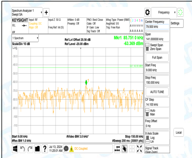
Band4-3MHz-QPSK-20175-1-0-Low-0.009-0.15-0.09--63.37-20.37--43-PASS
