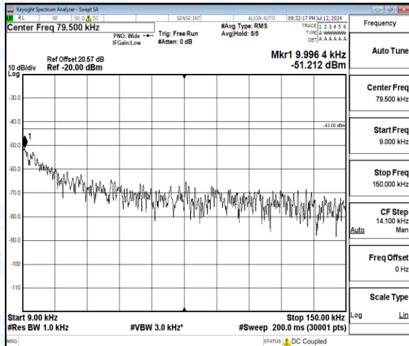
Band4-10MHz-16QAM-20000-1-0-Low-0.009-0.15-0.01--51.21-8.21--43-PASS
