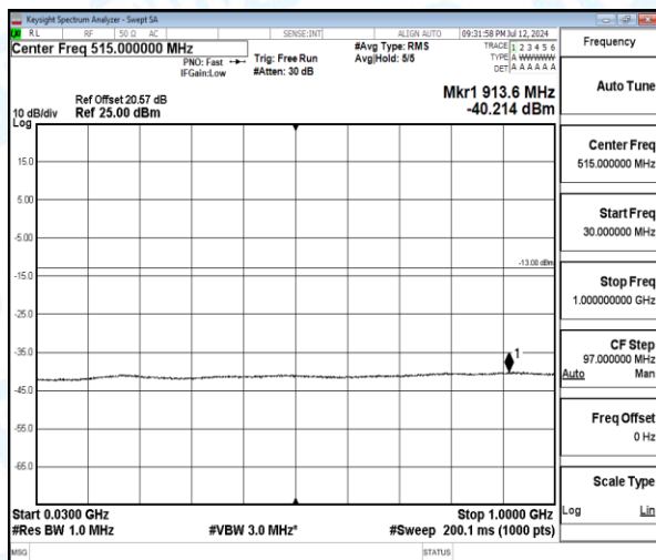
Band4-10MHz-QPSK-20000-1-0-Low-30-1000-913.58--40.21-27.21--13-PASS
