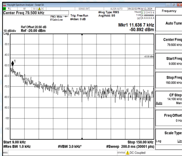
Band4-10MHz-QPSK-20175-1-0-Low-0.009-0.15-0.01--50.89-7.89--43-PASS
