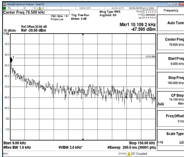
Band4-5MHz-QPSK-20175-1-0-Low-0.009-0.15-0.01--47.6-4.6--43-PASS
