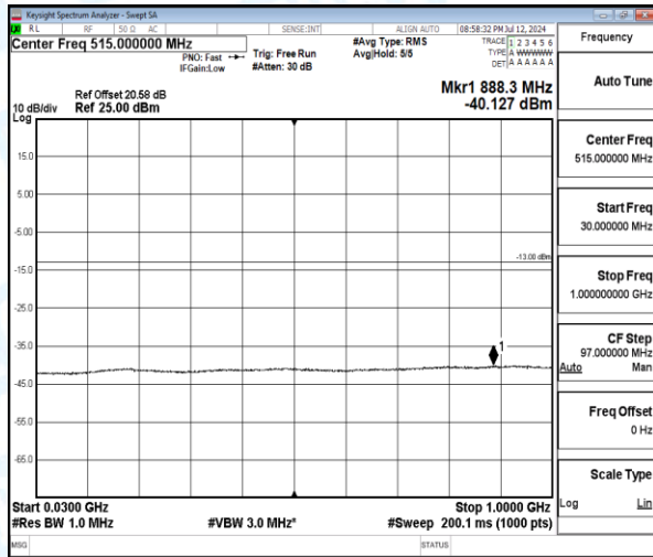
Band4-5MHz-16QAM-20375-1-0-High-30-1000-888.34--40.13-27.13--13-PASS
