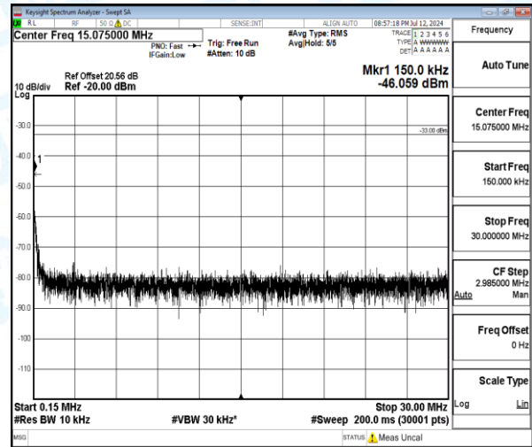
Band4-5MHz-16QAM-20175-1-0-Low-0.15-30-0.15--46.06-13.06--33-PASS
