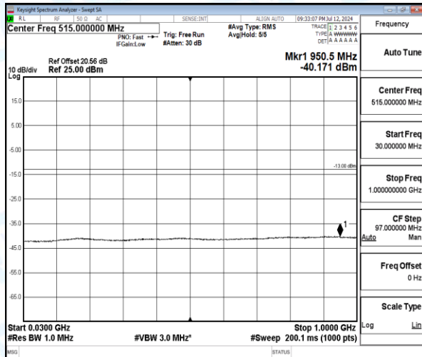
Band4-10MHz-QPSK-20175-1-0-Low-30-1000-950.48--40.17-27.17--13-PASS
