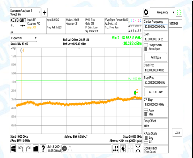
Band4-3MHz-16QAM-20385-1-0-High-1000-20000-18983.5--30.36-17.36--13-PASS
