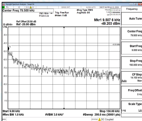
Band4-5MHz-QPSK-20375-1-0-High-0.009-0.15-0.01--49.2-6.2--43-PASS
