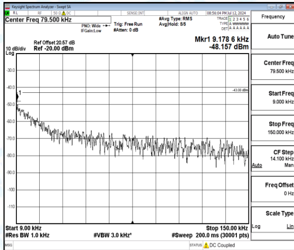
Band4-5MHz-16QAM-19975-1-0-Low-0.009-0.15-0.01--48.16-5.16--43-PASS
