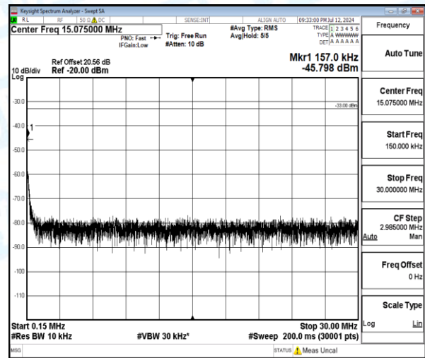
Band4-10MHz-QPSK-20175-1-0-Low-0.15-30-0.16--45.8-12.8--33-PASS
