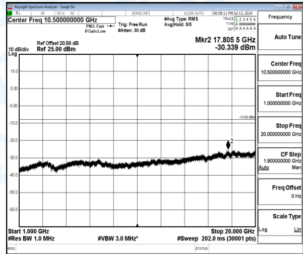
Band4-5MHz-QPSK-20375-1-0-High-1000-20000-17805.5--30.34-17.34--13-PASS
