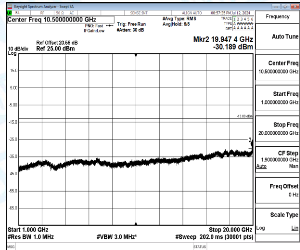
Band4-5MHz-16QAM-20175-1-0-Low-1000-20000-19947.43--30.19-17.19--13-PASS
