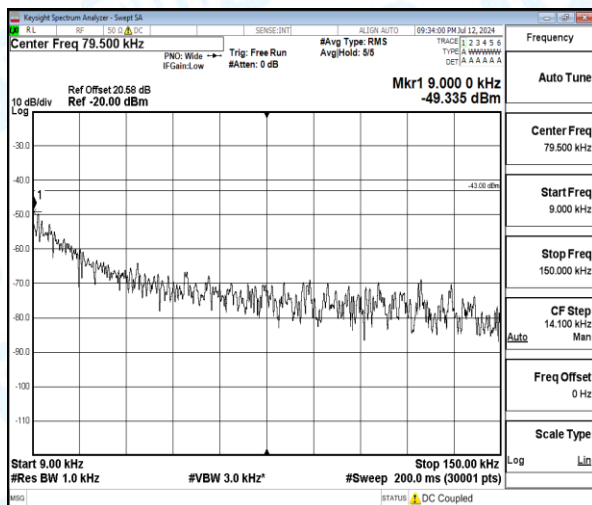
Band4-10MHz-QPSK-20350-1-0-High-0.009-0.15-0.01--49.34-6.34--43-PASS
