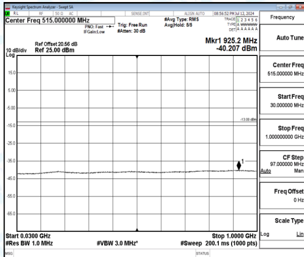
Band4-5MHz-QPSK-20175-1-0-Low-30-1000-925.24--40.21-27.21--13-PASS
