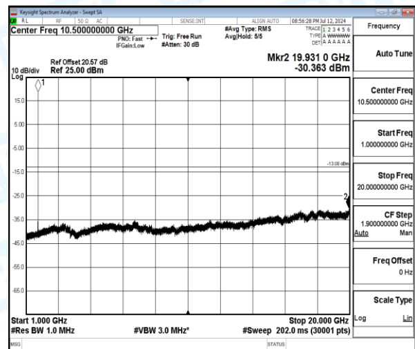
Band4-5MHz-16QAM-19975-1-0-Low-1000-20000-19930.97--30.36-17.36--13-PASS
