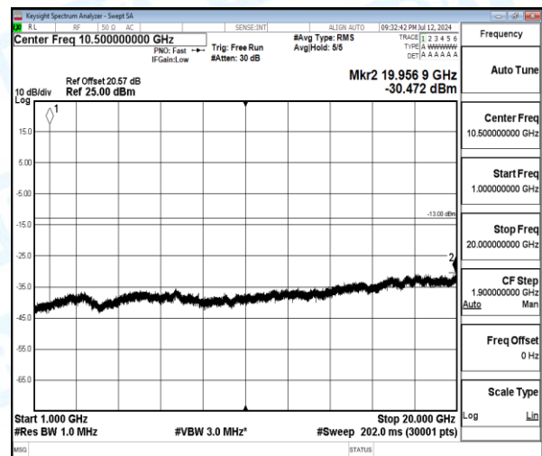
Band4-10MHz-16QAM-20000-1-0-Low-1000-19956.93--30.47-17.47--13-PASS
