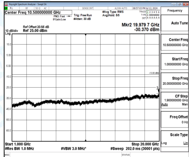
Band4-5MHz-QPSK-20175-1-0-Low-1000-20000-19979.73--30.37-17.37--13-PASS
