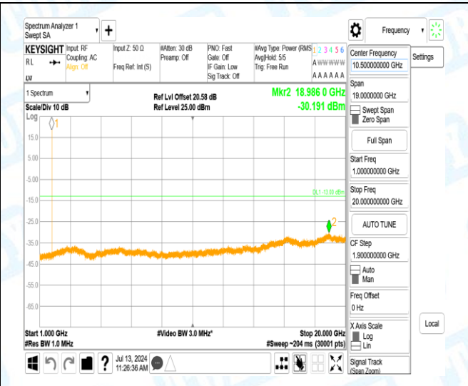
Band4-3MHz-QPSK-20385-1-0-High-1000-20000-18986.03--30.19-17.19--13-PASS
