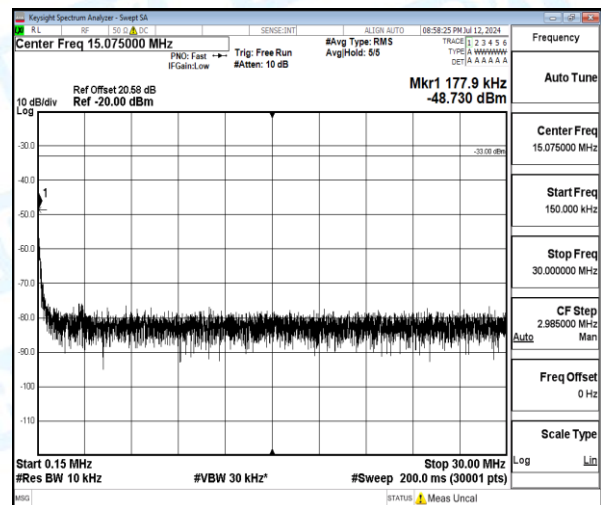
Band4-5MHz-16QAM-20375-1-0-High-0.15-30-0.18--48.73-15.73--33-PASS
