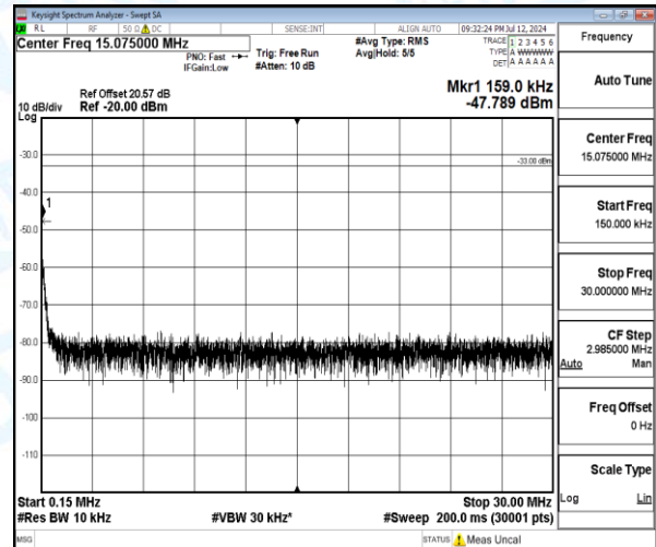
Band4-10MHz-16QAM-20000-1-0-Low-0.15-30-0.16--47.79-14.79--33-PASS
