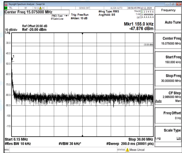
Band4-5MHz-QPSK-20175-1-0-Low-0.15-30-0.15--47.88-14.88--33-PASS
