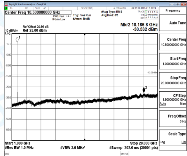
Band4-10MHz-QPSK-20175-1-0-Low-1000-20000-18186.77--30.53-17.53--13-PASS
