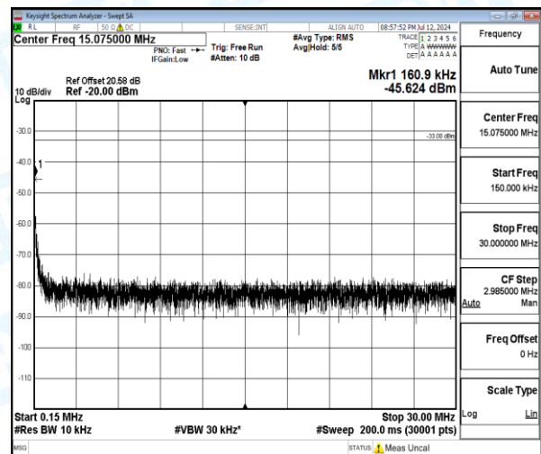
Band4-5MHz-QPSK-20375-1-0-High-0.15-30-0.16--45.62-12.62--33-PASS
