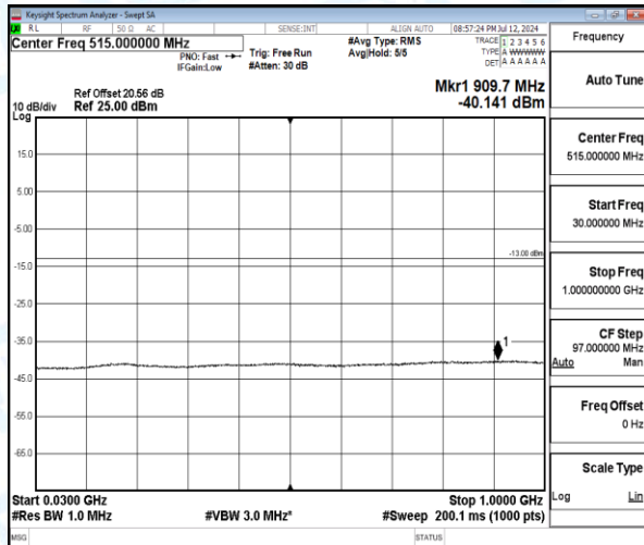
Band4-5MHz-16QAM-20175-1-0-Low-30-1000-909.7--40.14-27.14--13-PASS
