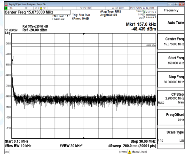
Band4-10MHz-QPSK-20000-1-0-Low-0.15-30-0.16--48.44-15.44--33-PASS
