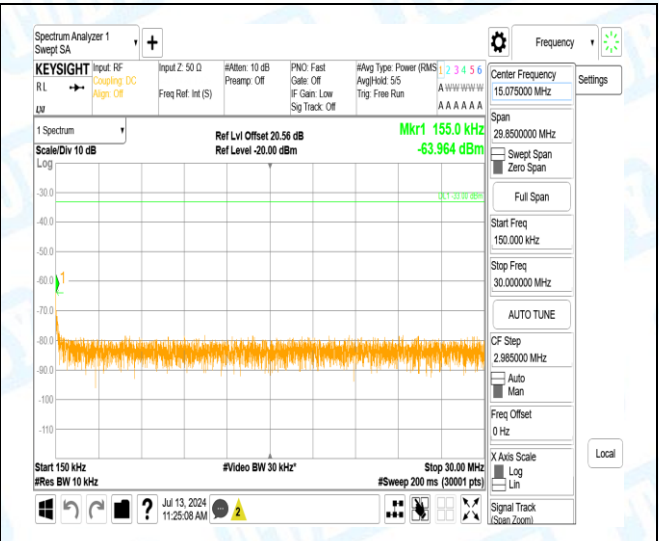
Band4-3MHz-QPSK-20175-1-0-Low-0.15-30-0.15--63.96-30.96--33-PASS
