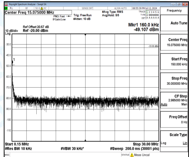
Band4-5MHz-QPSK-19975-1-0-Low-0.15-30-0.16--49.11-16.11--33-PASS
