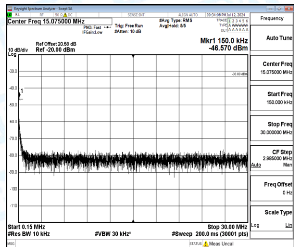
Band4-10MHz-QPSK-20350-1-0-High-0.15-30-0.15--46.57-13.57--33-PASS
