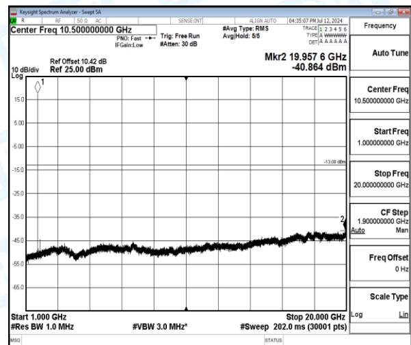
Band4-3MHz-16QAM-19965-1-0-Low-1000-20000-19957.57--40.86-27.86--13-PASS
