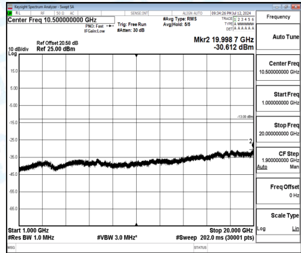
Band4-10MHz-QPSK-20350-1-0-High-1000-19998.73--30.61-17.61--13-PASS
