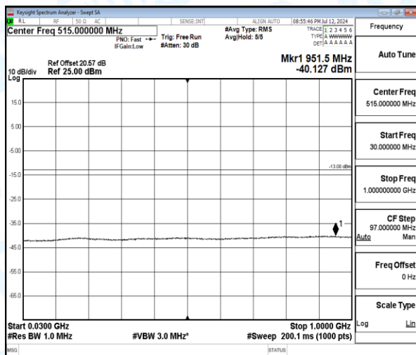
Band4-5MHz-QPSK-19975-1-0-Low-30-1000-951.45--40.13-27.13--13-PASS
