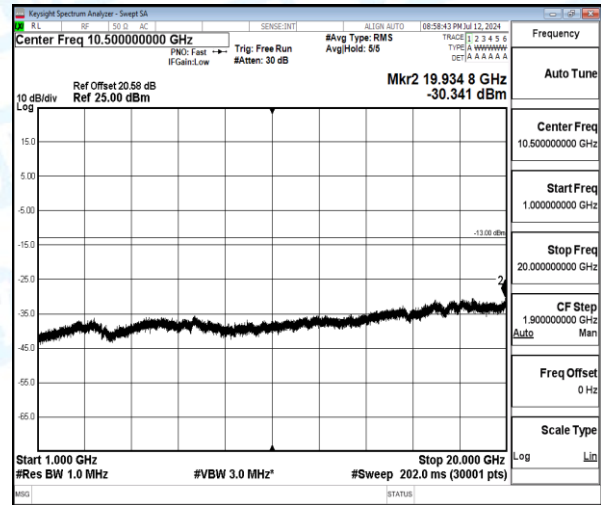
Band4-5MHz-16QAM-20375-1-0-High-1000-20000-19934.77--30.34-17.34--13-PASS
