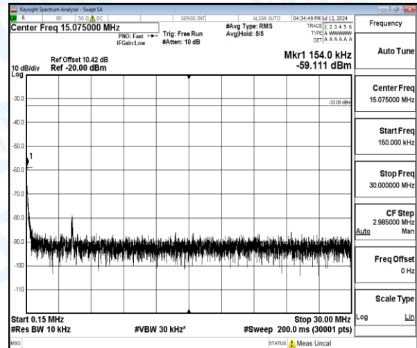
Band4-3MHz-16QAM-19965-1-0-Low-0.15-30-0.15--59.11-26.11--33-PASS
