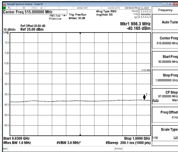
Band4-5MHz-QPSK-20375-1-0-High-30-1000-956.31--40.17-27.17--13-PASS
