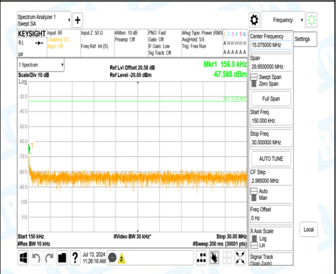
Band4-3MHz-QPSK-20385-1-0-High-0.15-30-0.16--67.59-34.59--33-PASS
