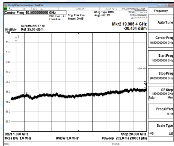
Band4-10MHz-QPSK-20000-1-0-Low-1000-20000-19985.43--30.43-17.43--13-PASS
