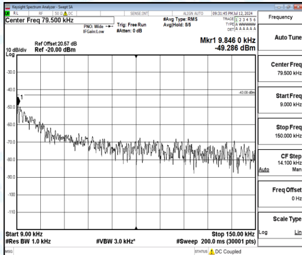
Band4-10MHz-QPSK-20000-1-0-Low-0.009-0.15-0.01--49.29-6.29--43-PASS
