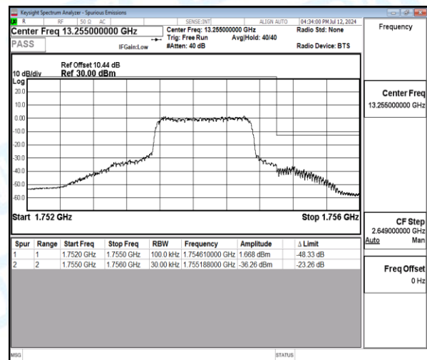
Band4-3MHz-16QAM-20385-6-0-High-1755.19--36.26-23.26-PASS
