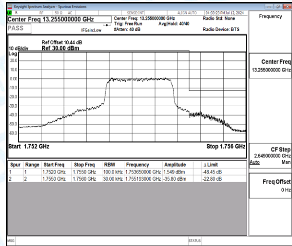
Band4-3MHz-QPSK-20385-6-0-High-1755.19--35.80-22.80-PASS
