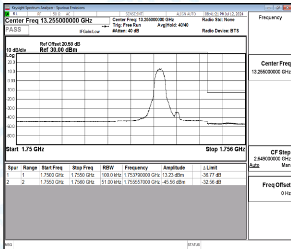
Band4-5MHz-16QAM-20375-1-0-High-1755.56--45.56-32.56-PASS
