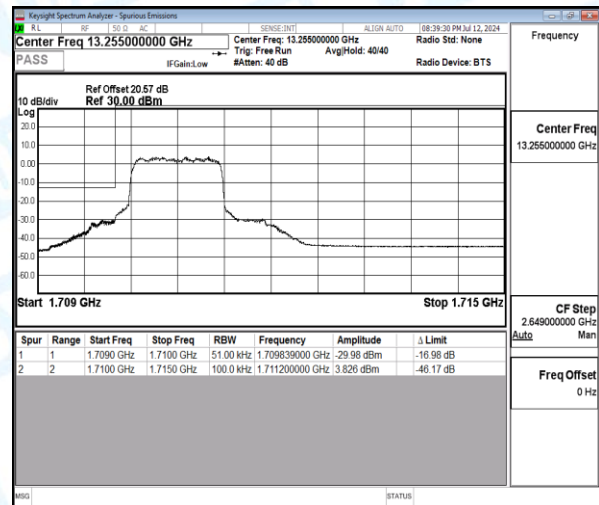
Band4-5MHz-QPSK-19975-6-0-Low-1709.84--29.98-16.98-PASS
