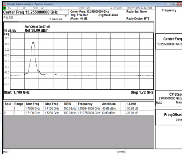
Band4-10MHz-QPSK-20000-1-0-Low-1709.94--43.68-30.68-PASS
