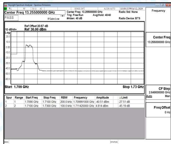
Band4-20MHz-16QAM-20050-6-0-Low-1709.99--40.51-27.51-PASS
