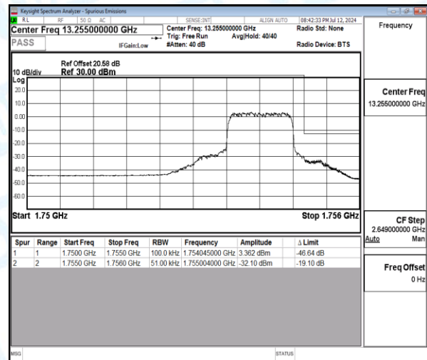
Band4-5MHz-16QAM-20375-6-0-High-1755.00--32.10-19.10-PASS
