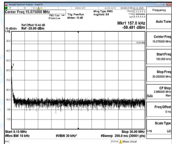
Band4-1.4MHz-QPSK-20393-1-0-High-0.15-30-0.16--59.49-26.49--33-PASS
