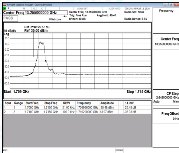
Band4-5MHz-QPSK-19975-1-0-Low-1710.00--38.48-25.48-PASS
