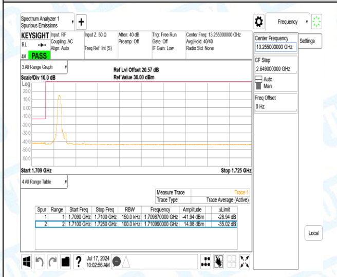
Band4-15MHz-16QAM-20025-1-0-Low-1709.87--41.94-28.94-PASS
