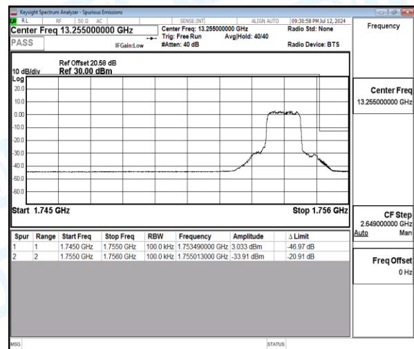
Band4-10MHz-QPSK-20350-6-0-High-1755.01--33.91-20.91-PASS
