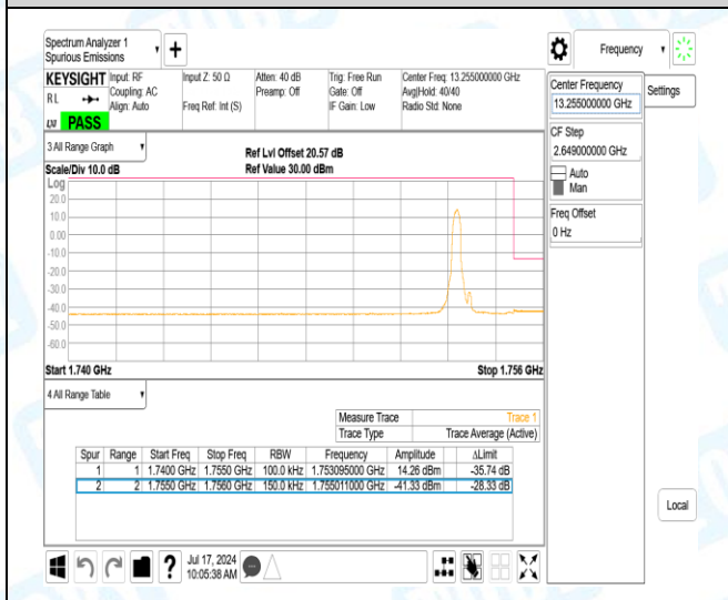
Band4-15MHz-16QAM-20325-1-0-High-1755.01--41.33-28.33-PASS
