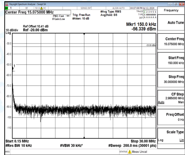
Band4-1.4MHz-QPSK-20175-1-0-Low-0.15-30-0.15--56.34-23.34--33-PASS
