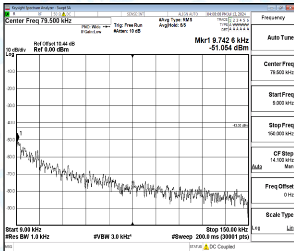
Band4-1.4MHz-QPSK-20393-1-0-High-0.009-0.15-0.01--51.05-8.05--43-PASS
