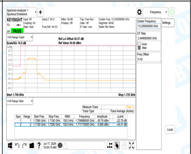
Band4-15MHz-16QAM-20025-6-0-Low-1709.99--35.78-22.78-PASS
