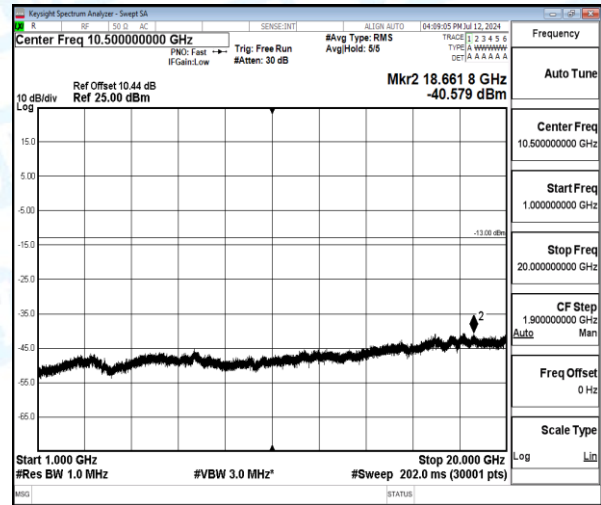
Band4-1.4MHz-16QAM-20393-1-0-High-1000-20000-18661.77--40.58-27.58--13-PASS
