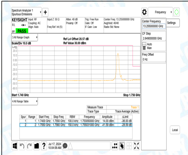
Band4-15MHz-QPSK-20325-1-0-High-1755.03--41.59-28.59-PASS
