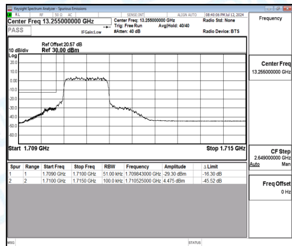
Band4-5MHz-16QAM-19975-6-0-Low-1709.84--29.30-16.30-PASS
