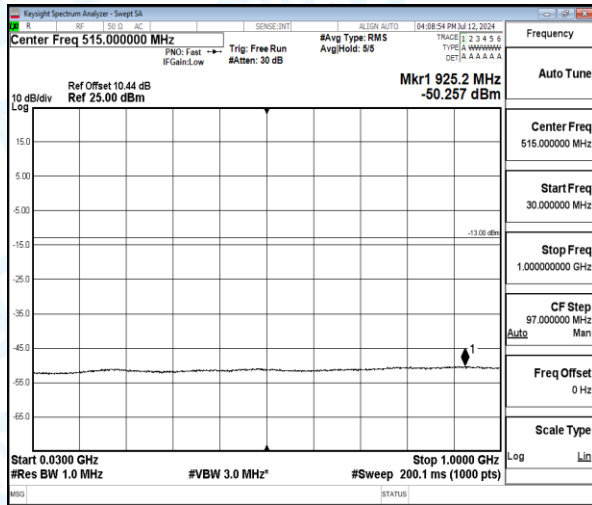
Band4-1.4MHz-16QAM-20393-1-0-High-30-1000-925.24--50.26-37.26--13-PASS
