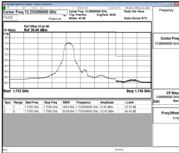
Band4-3MHz-QPSK-20385-1-0-High-1755.43--53.43-40.43-PASS
