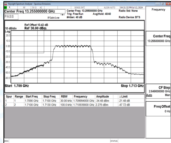
Band4-3MHz-16QAM-19965-6-0-Low-1709.99--34.48-21.48-PASS
