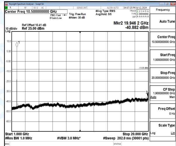
Band4-1.4MHz-QPSK-20175-1-0-Low-1000-20000-19946.17--40.88-27.88--13-PASS
