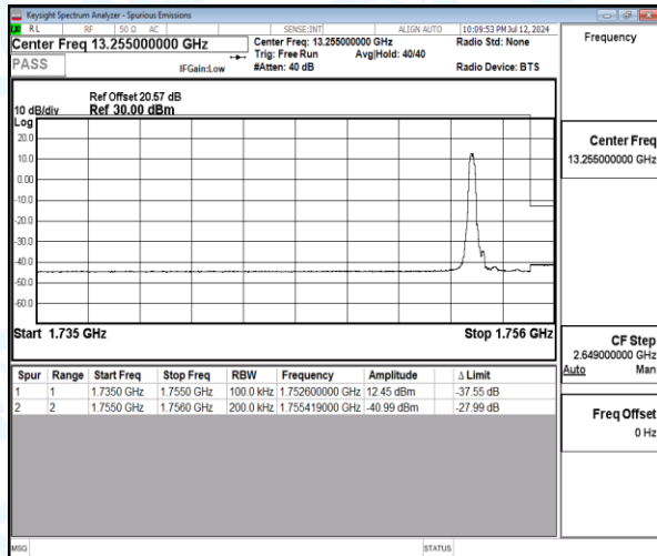
Band4-20MHz-QPSK-20300-1-0-High-1755.42--40.99-27.99-PASS
