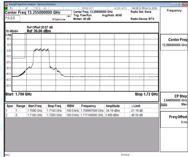
Band4-10MHz-QPSK-20000-6-0-Low-1710.00--34.19-21.19-PASS
