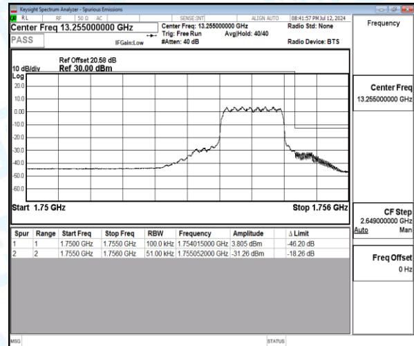
Band4-5MHz-QPSK-20375-6-0-High-1755.05--31.26-18.26-PASS
