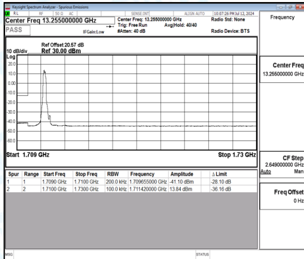
Band4-20MHz-QPSK-20050-1-0-Low-1709.66--41.10-28.10-PASS
