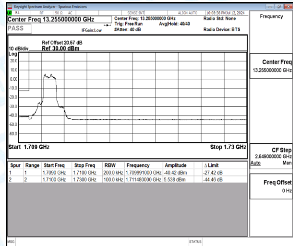
Band4-20MHz-QPSK-20050-6-0-Low-1709.99--40.42-27.42-PASS
