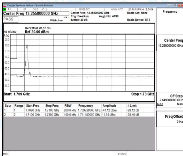
Band4-20MHz-16QAM-20050-1-0-Low-1709.73--41.12-28.12-PASS
