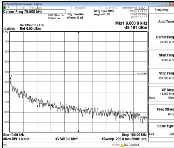
Band4-1.4MHz-QPSK-20175-1-0-Low-0.009-0.15-0.01--49.19-6.19--43-PASS
