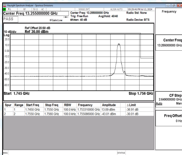
Band4-10MHz-QPSK-20350-1-0-High-1755.09--43.01-30.01-PASS
