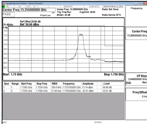
Band4-5MHz-QPSK-20375-1-0-High-1755.56--45.61-32.61-PASS
