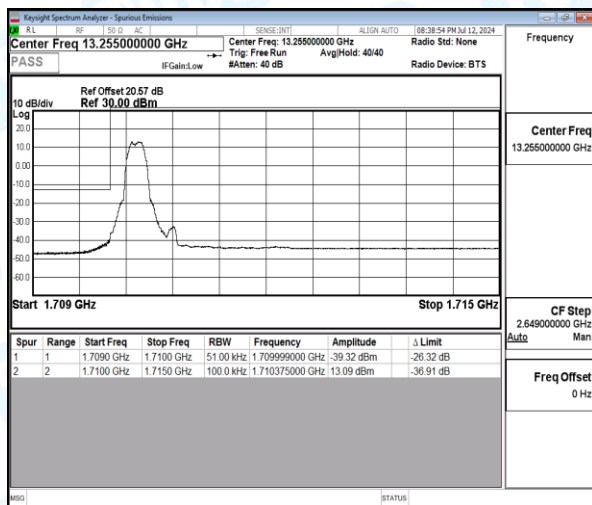
Band4-5MHz-16QAM-19975-1-0-Low-1710.00--39.32-26.32-PASS
