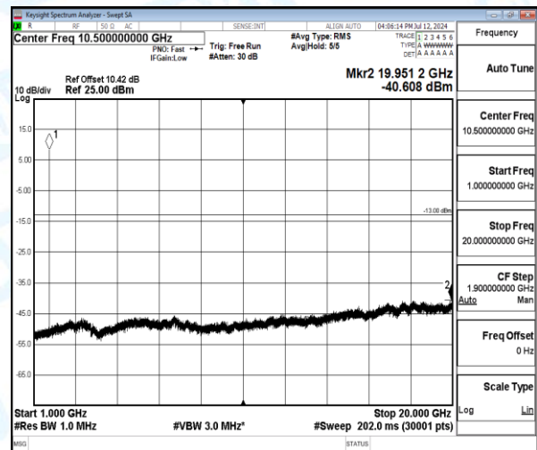
Band4-1.4MHz-QPSK-19957-1-0-Low-1000-20000-19951.23--40.61-27.61--13-PASS
