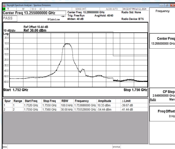
Band4-3MHz-16QAM-20385-1-0-High-1755.53--54.44-41.44-PASS
