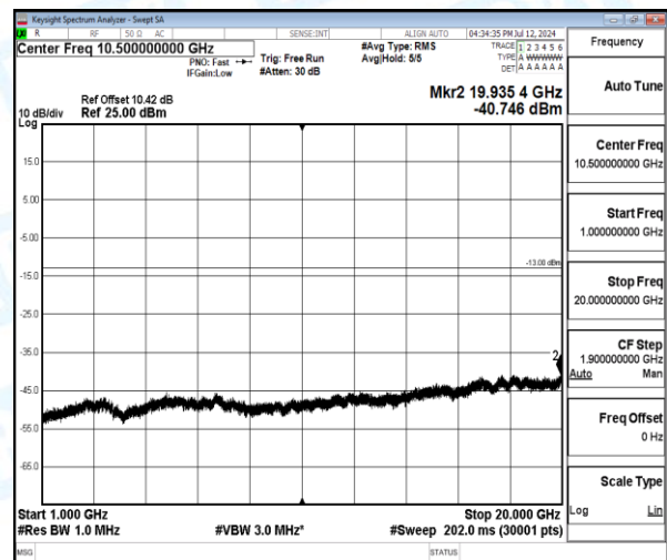
Band4-3MHz-QPSK-19965-1-0-Low-1000-20000-19935.4--40.75-27.75--13-PASS
