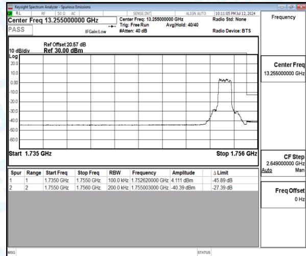
Band4-20MHz-QPSK-20300-6-0-High-1755.00--40.39-27.39-PASS
