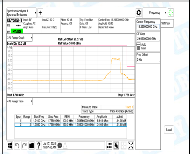
Band4-15MHz-16QAM-20325-6-0-High-1755.00--34.65-21.65-PASS
