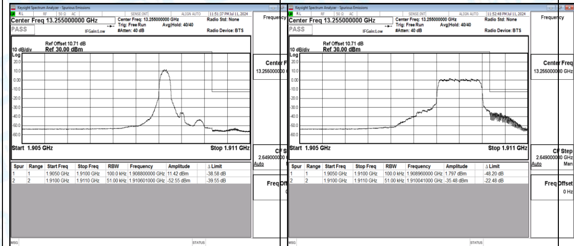
Band2-5MHz-16QAM-19175-1-0-High-1910.60--52.55-39.55-PASS
