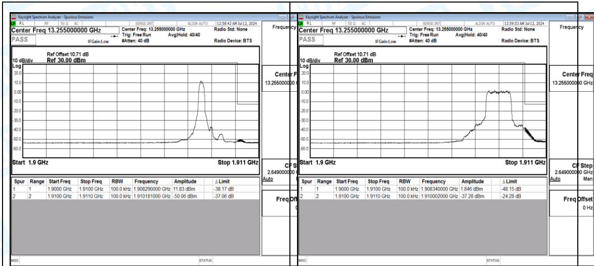
Band2-10MHz-QPSK-19150-1-0-High-1910.18--50.06-37.06-PASS
