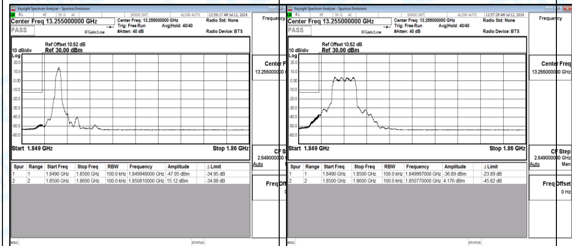
Band2-10MHz-QPSK-18650-1-0-Low-1849.95--47.95-34.95-PASS
