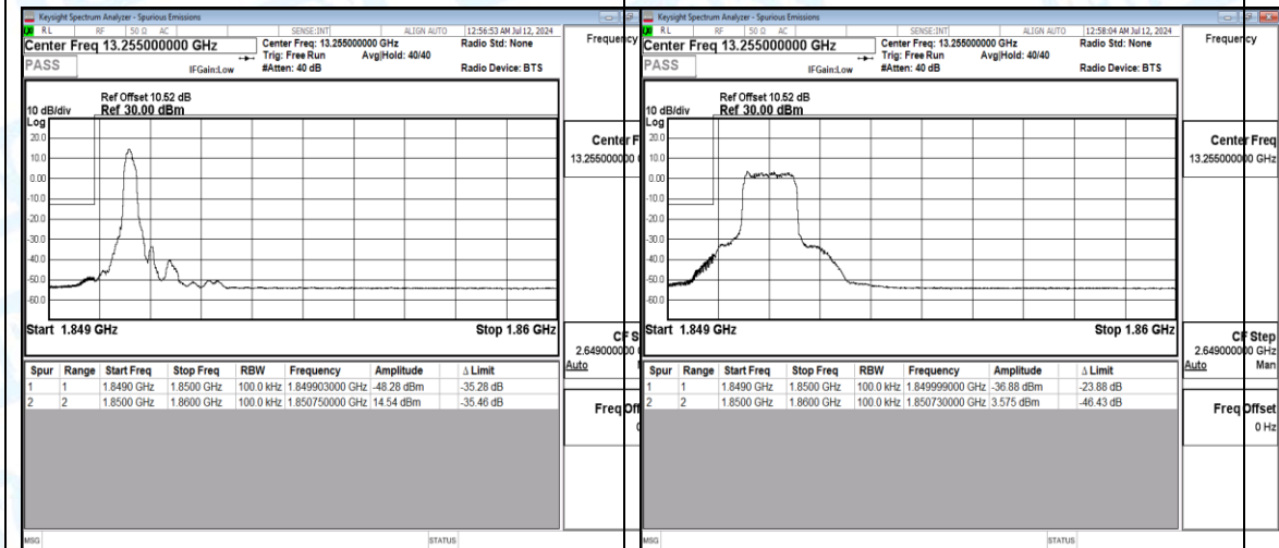
Band2-10MHz-16QAM-18650-1-0-Low-1849.90--48.28-35.28-PASS
