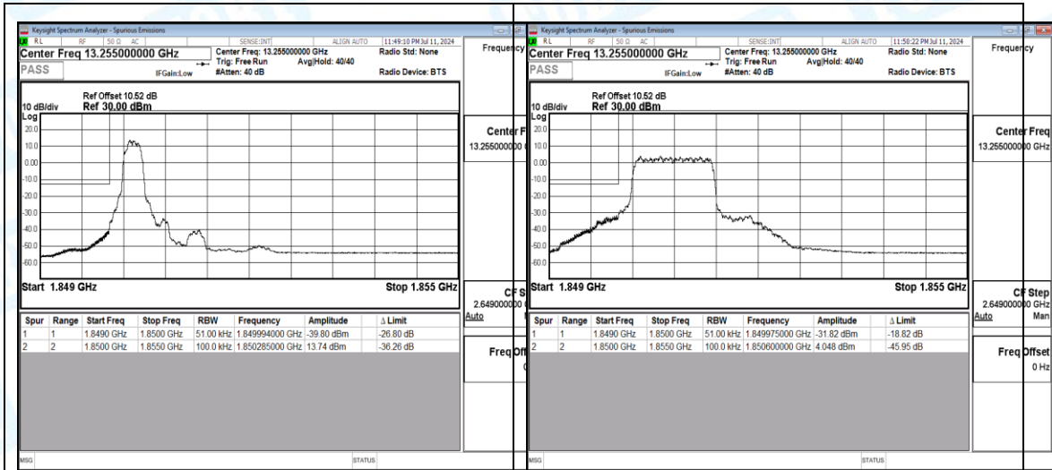
Band2-5MHz-16QAM-18625-1-0-Low-1849.99--39.80-26.80-PASS
