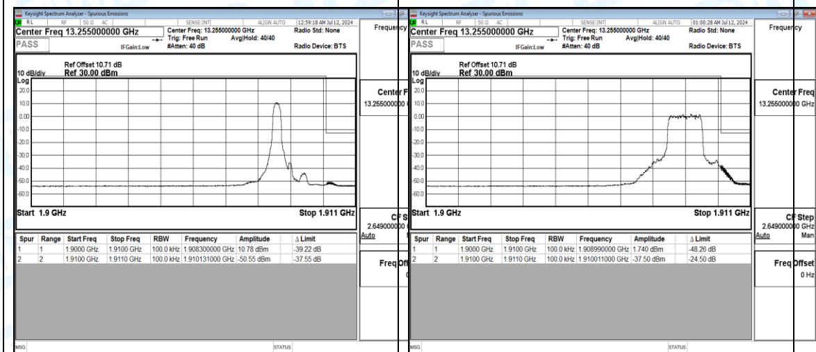
Band2-10MHz-16QAM-19150-1-0-High-1910.13--50.55-37.55-PASS
