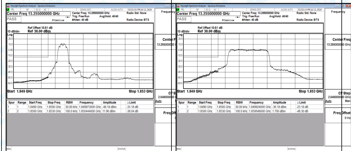
Band2-3MHz-16QAM-18615-1-0-Low-1849.97--48.18-35.18-PASS
