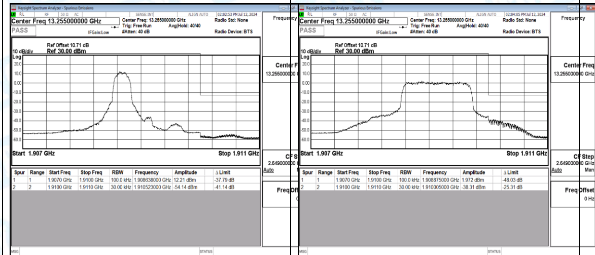
Band2-3MHz-QPSK-19185-1-0-High-1910.52--54.14-41.14-PASS
