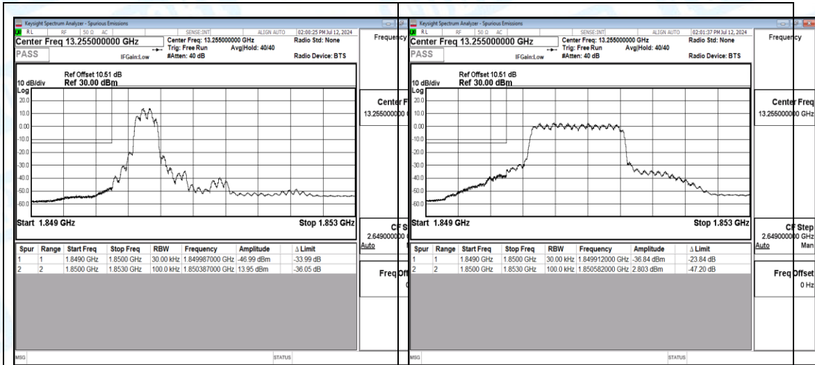
Band2-3MHz-QPSK-18615-1-0-Low-1849.99--46.99-33.99-PASS
