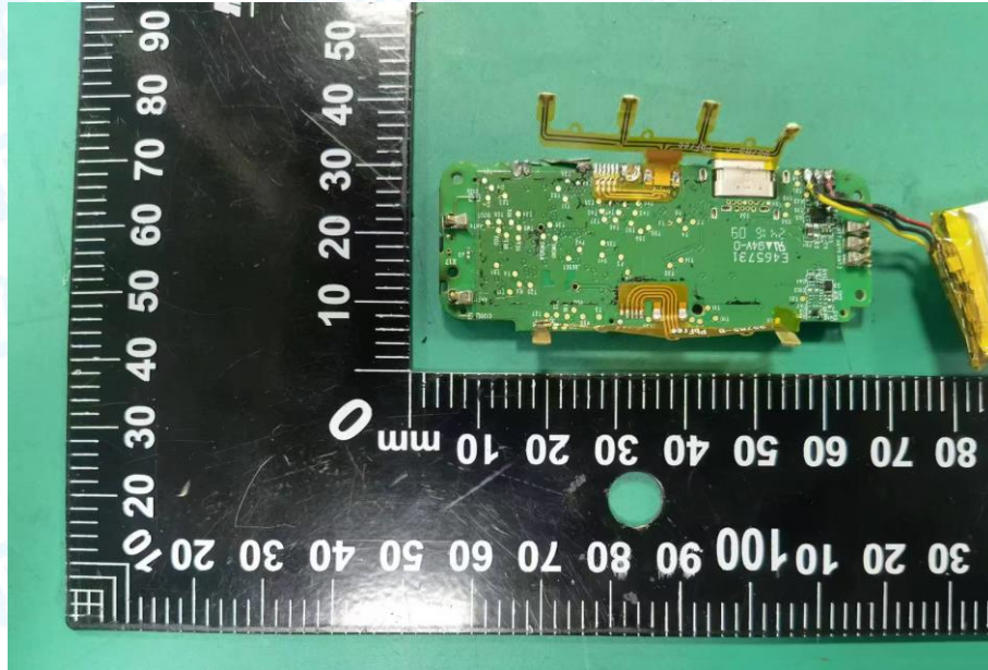
Photo 18 Appearance of PCB
