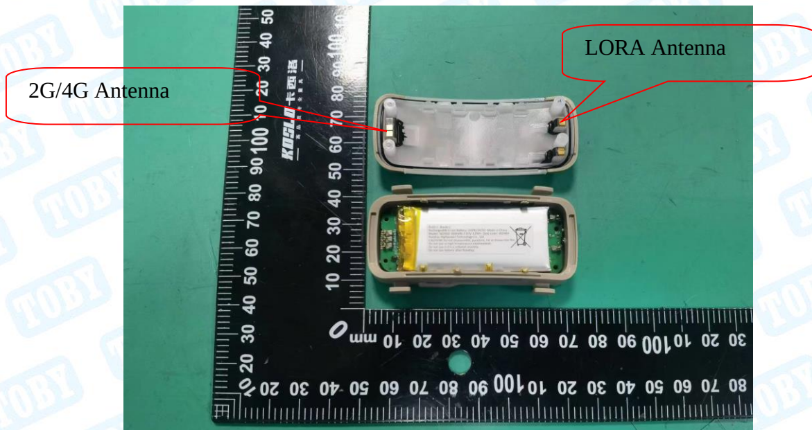
Photo 13 Internal of EUT
