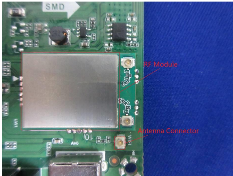
RF Module location-2
