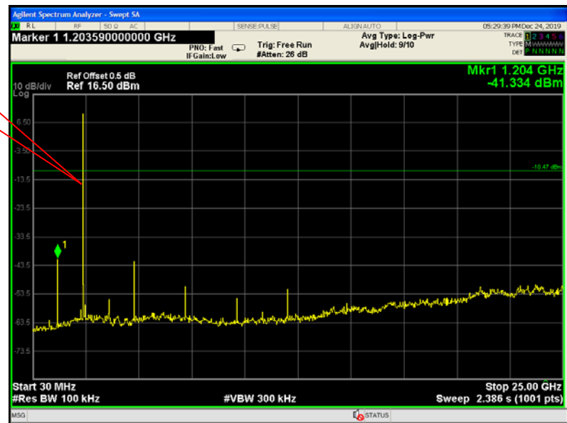
30MHz – 25GHz GFSK Low Channel
