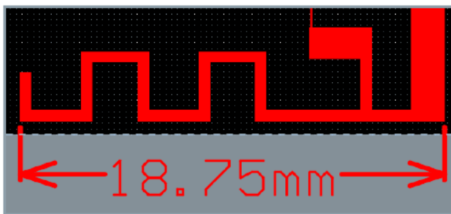
Figure 1 - Antenna structure.
