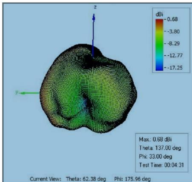
Figure 2 - 3D gain.
