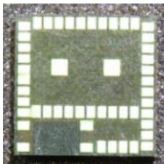
Figure 2: Bottom view
