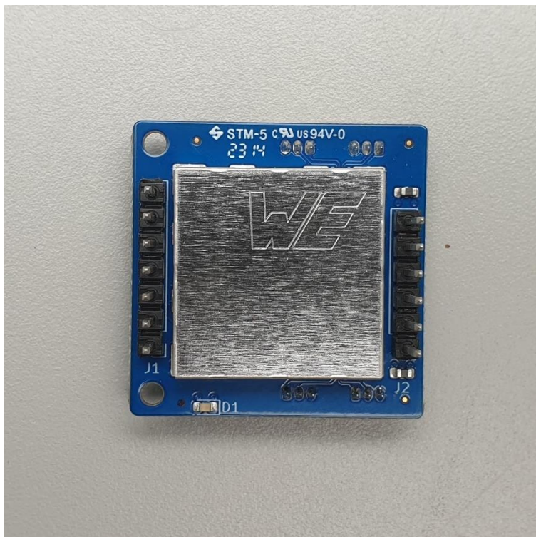
Photo 2. NFC MUX Bottom view.
