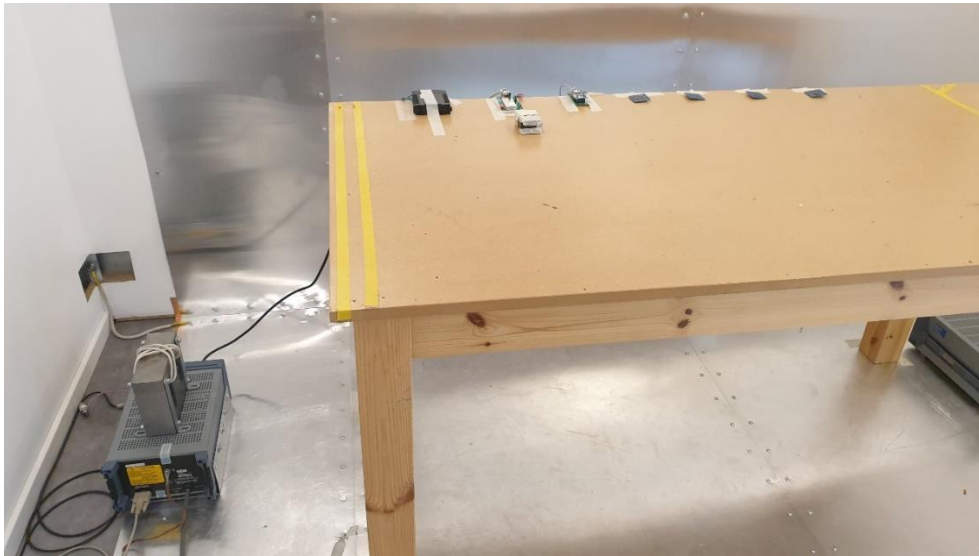
Photo 13. AC Conducted emission test set up.
