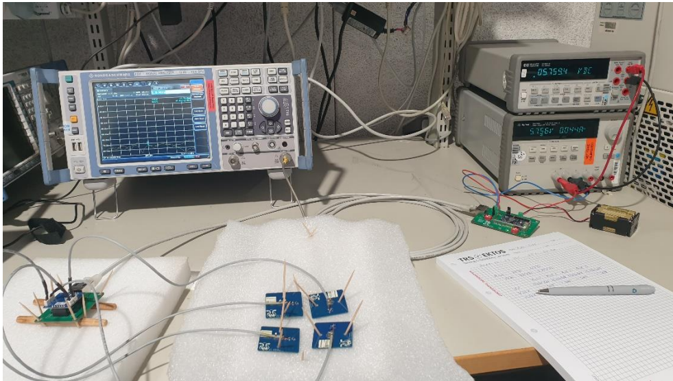
Photo 8. Frequency stability versus supply voltage test setup.
