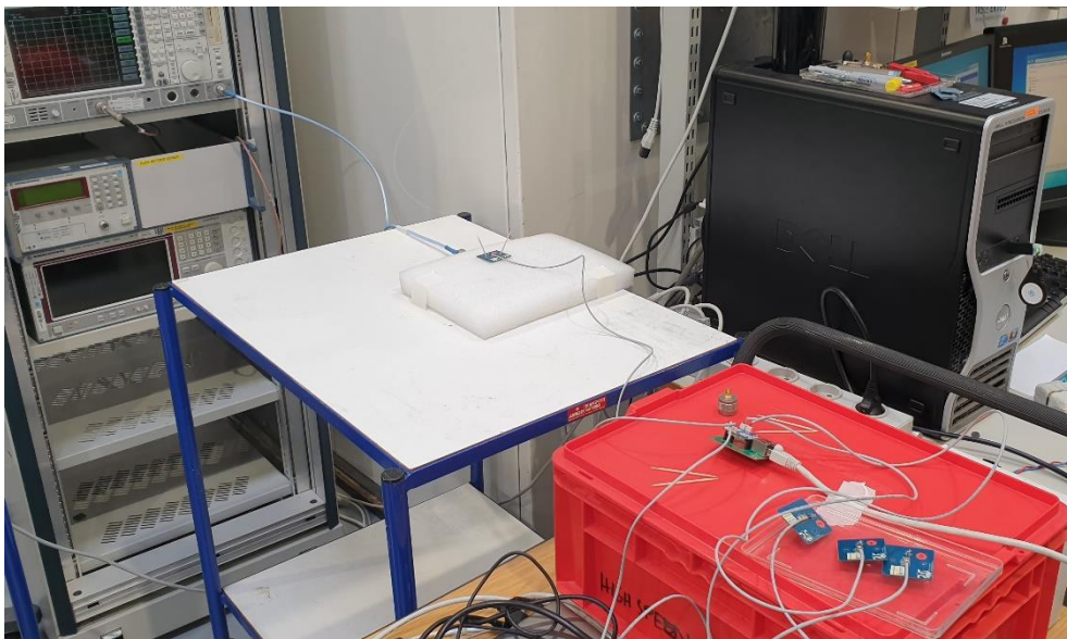
Photo 9. Occupied bandwidth test setup.
