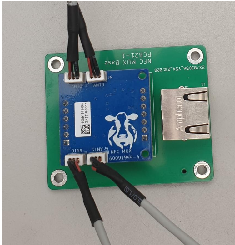
Photo 1. NFC MUX mounted at NFC Mux Base and antennas connected.
