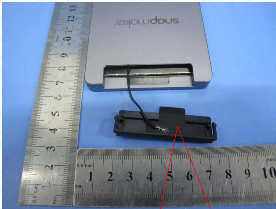
2.4G BT, WiFi and 5G WiFi FPC antenna
