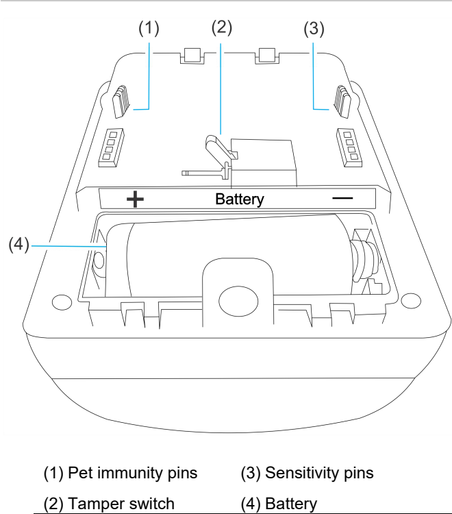
Figure 2: Sensor pins and tamper switch
