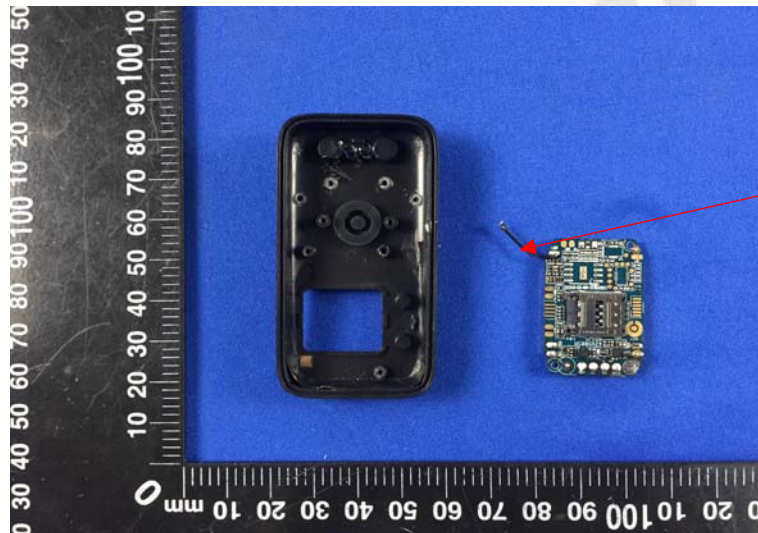
WIFI Antenna
