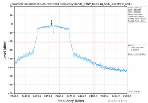
Right bandedge
