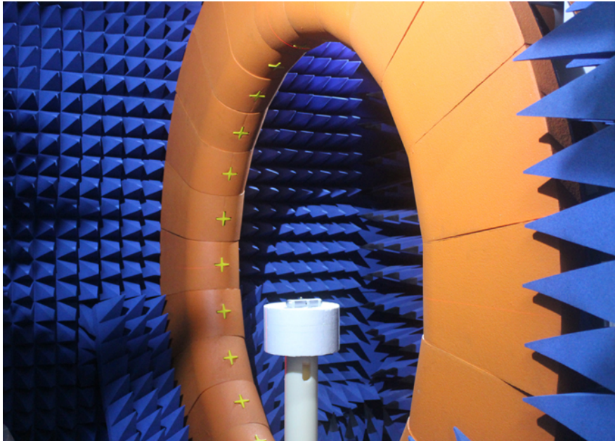
探头微波暗室Probe microwave anechoic chamber
